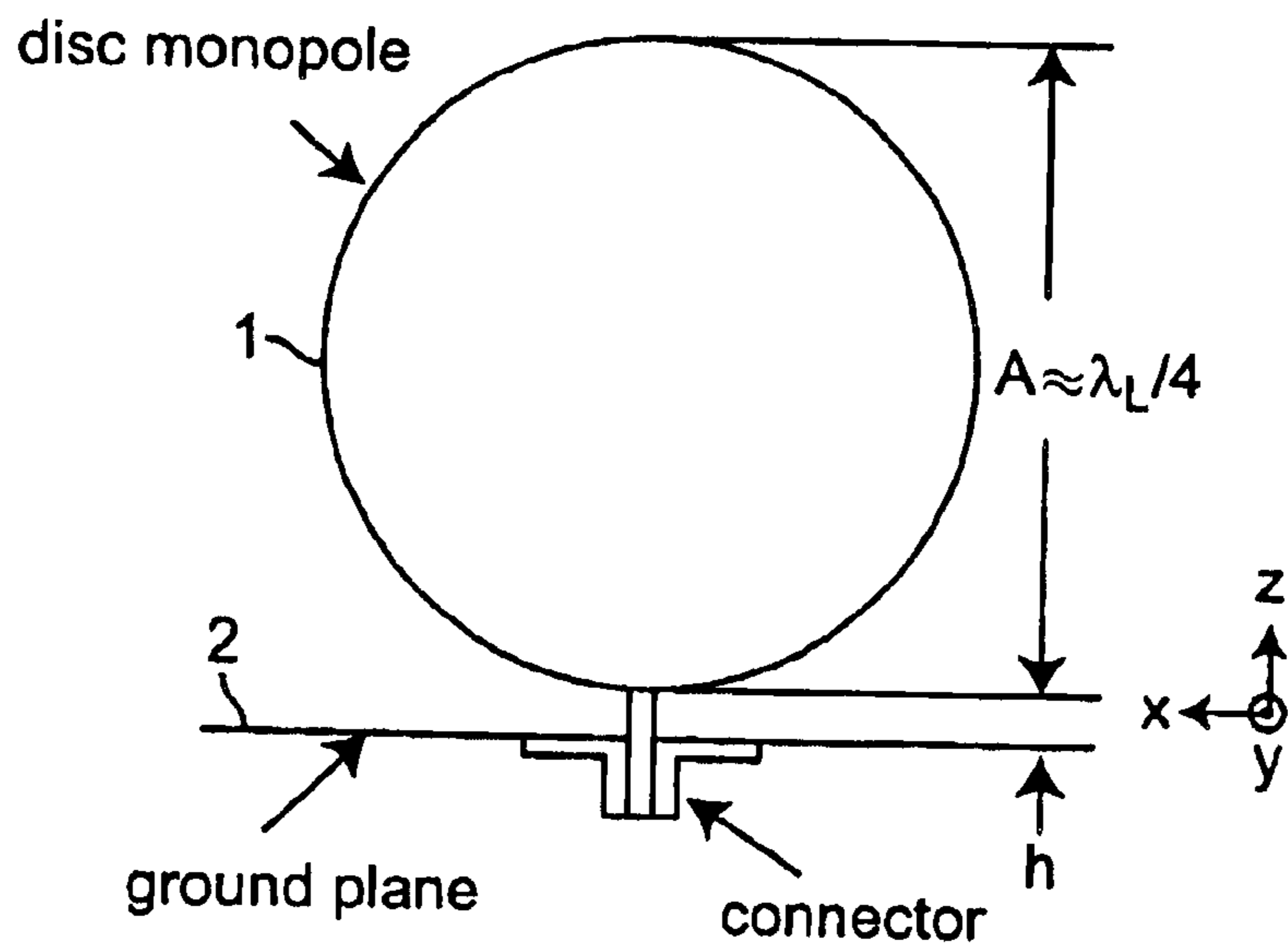
Figure 1 PRIOR ART
