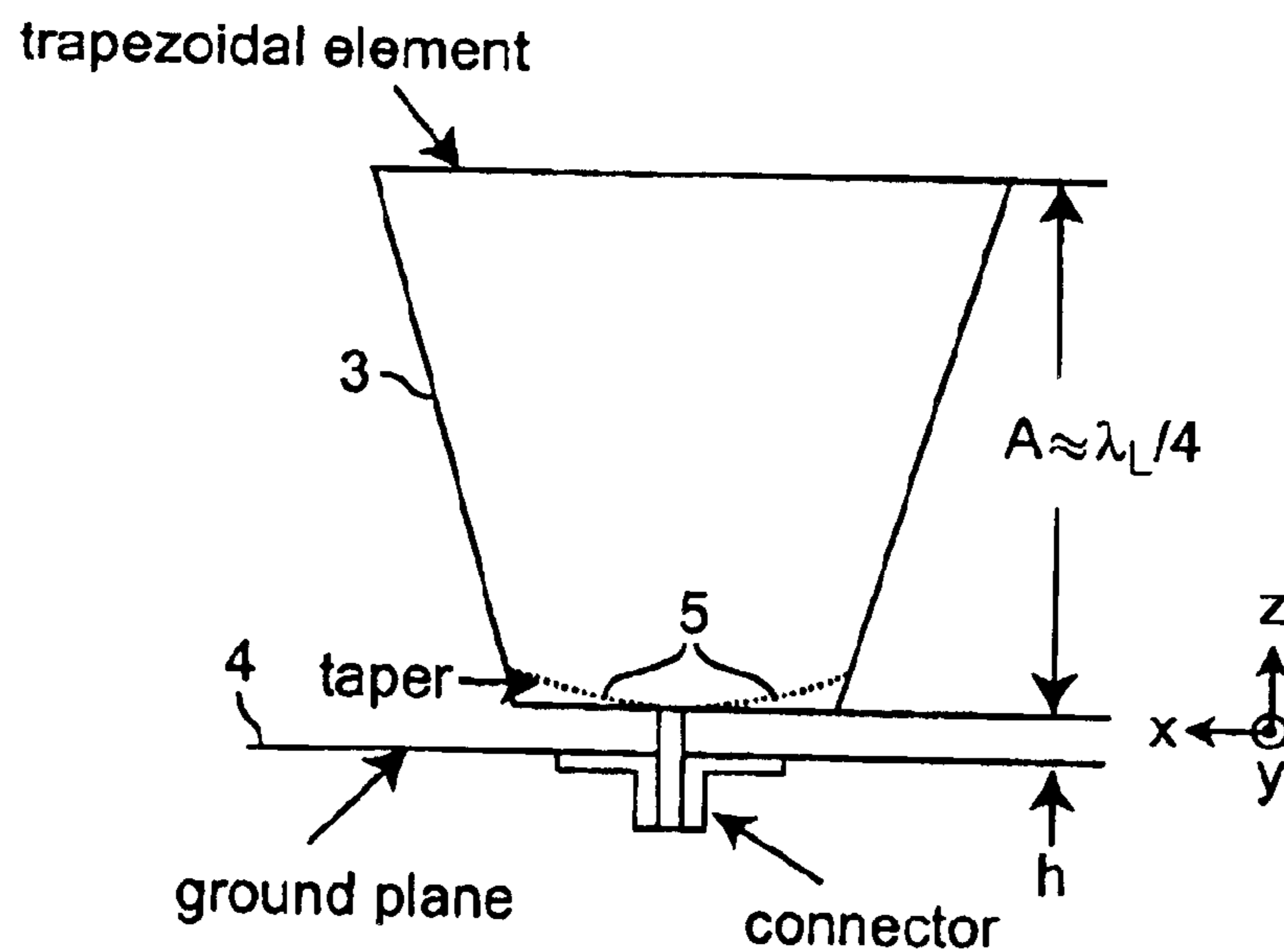
Figure 2 PRIOR ART
