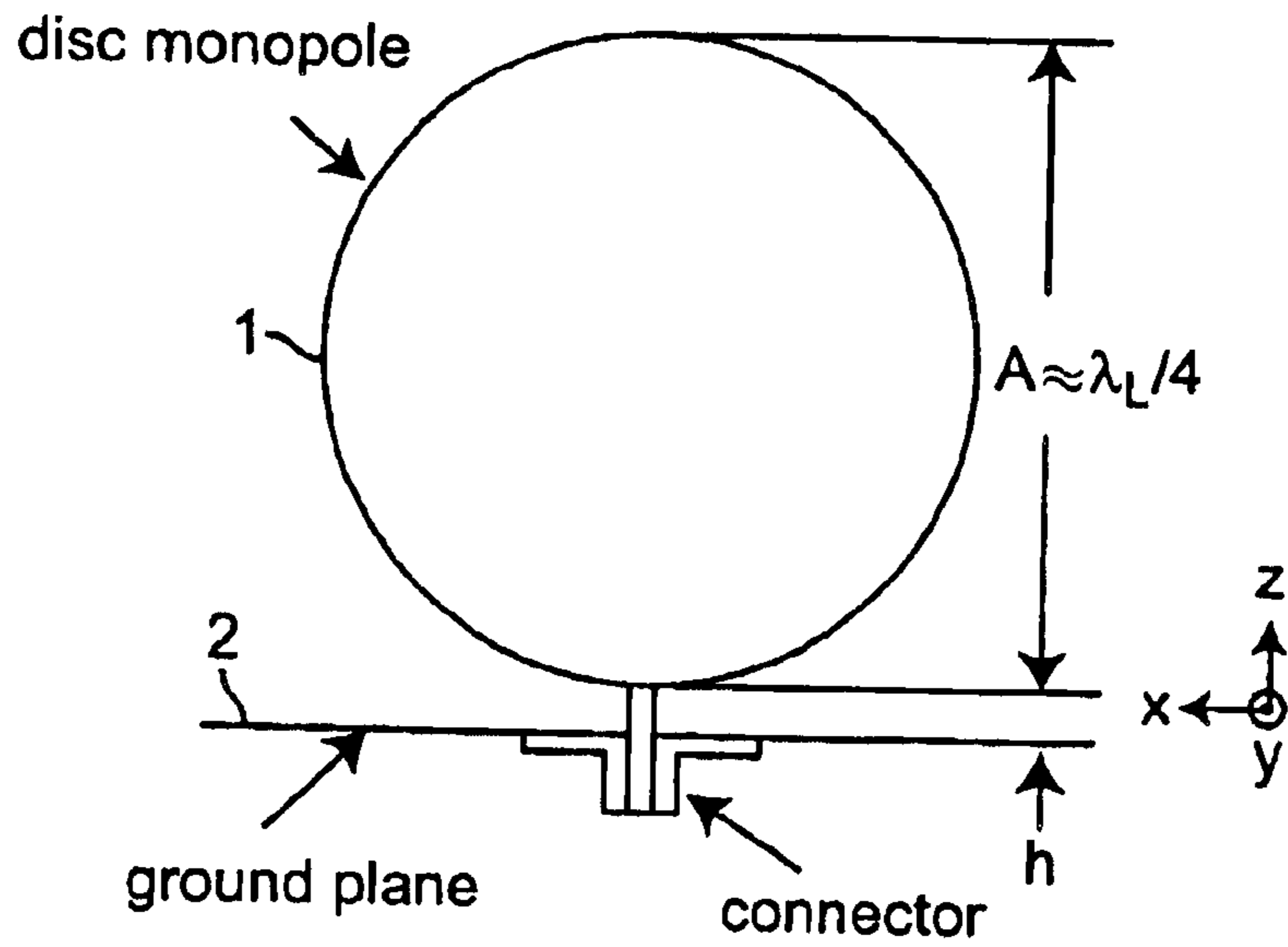
Figure 1 PRIOR ART
