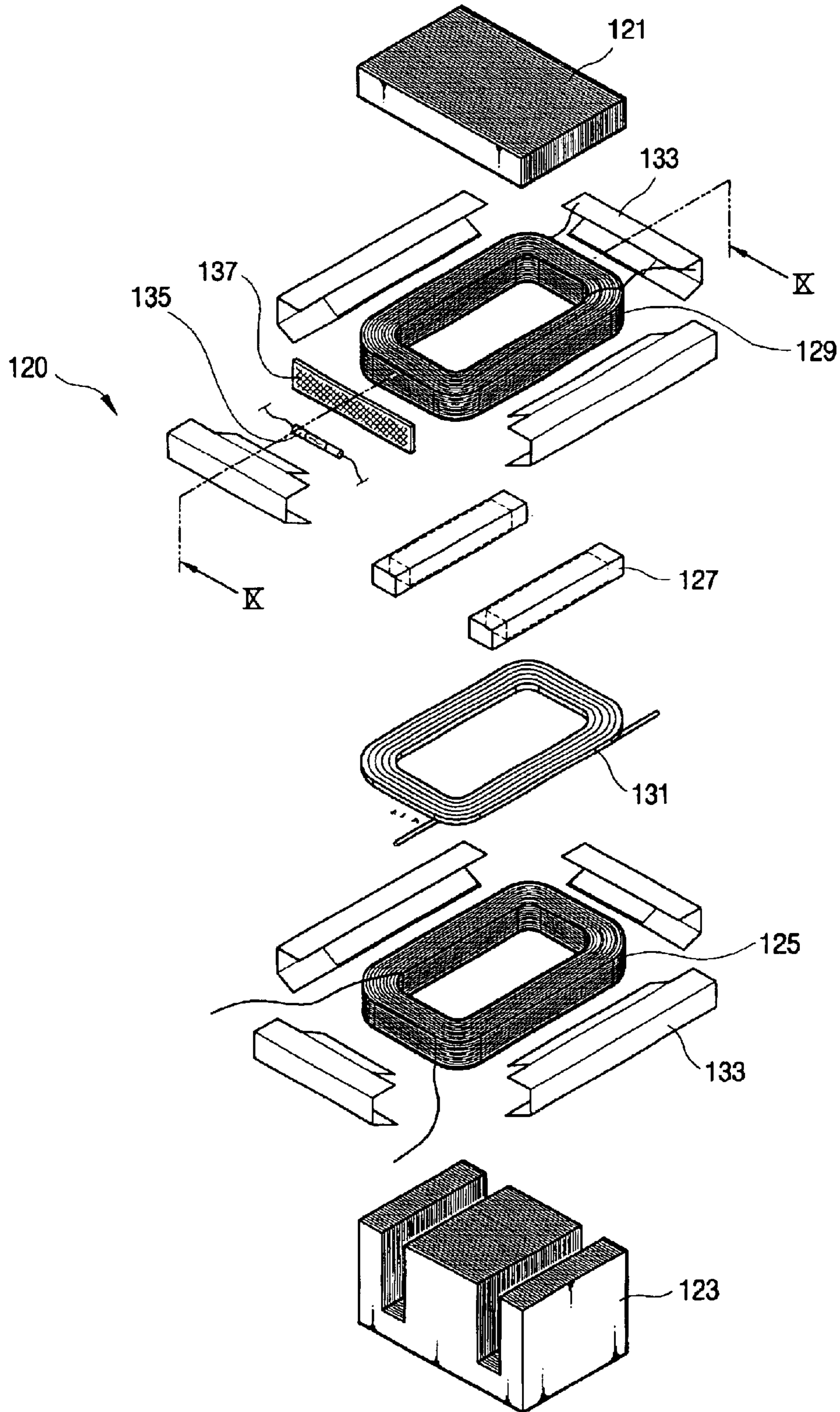
FIG. 8 PRIOR ART
