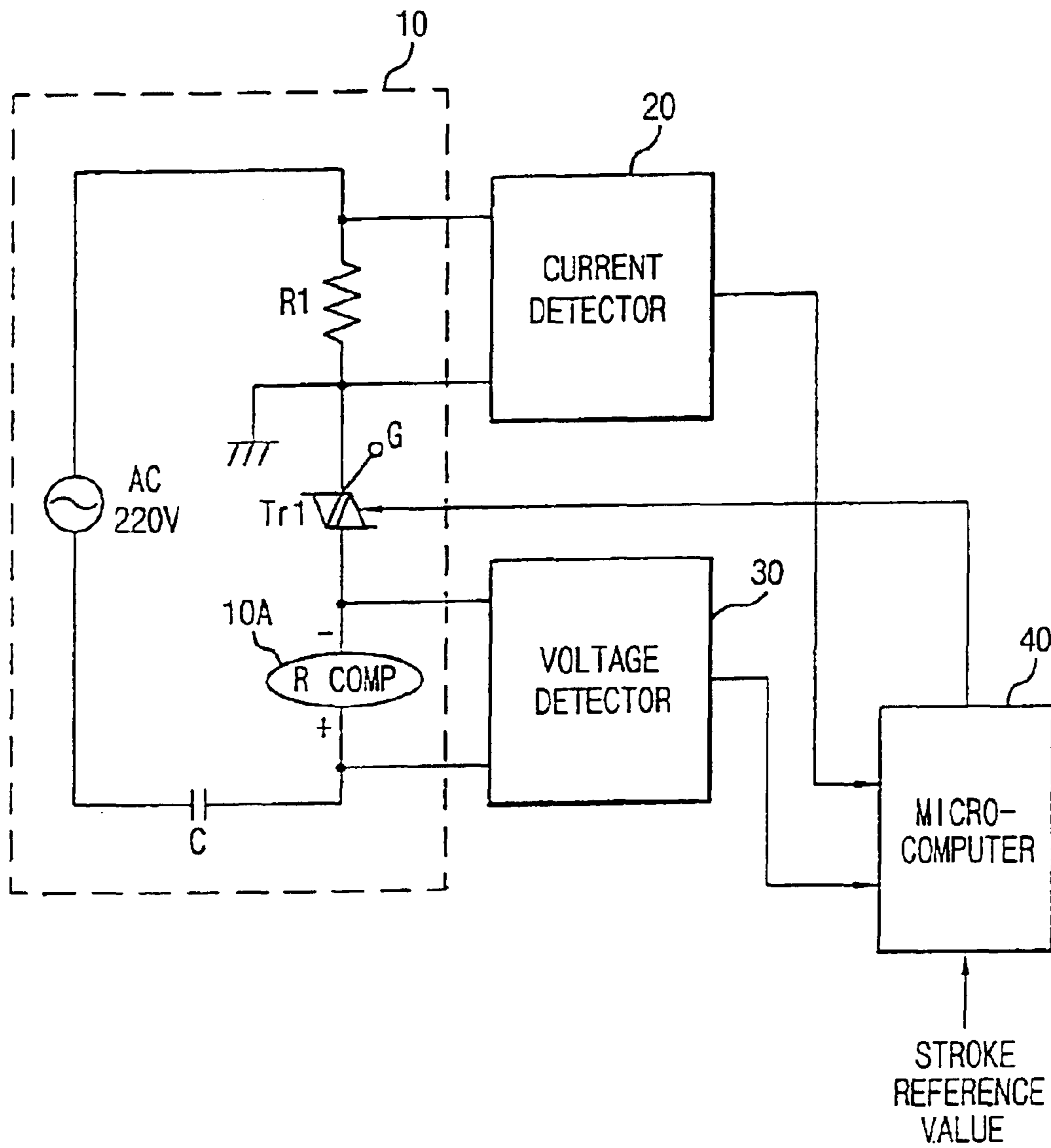
FIG. 1 CONVENTIONAL ART
