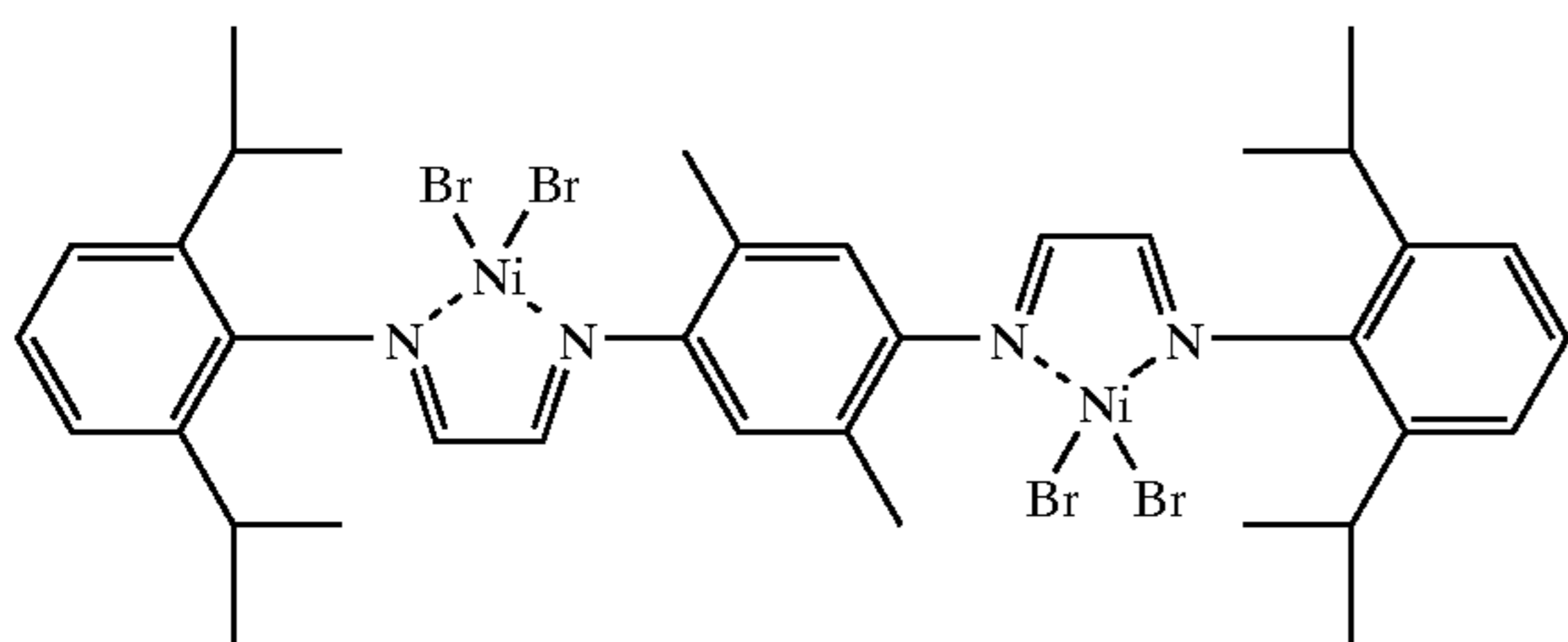
[COMPOUND 18]
