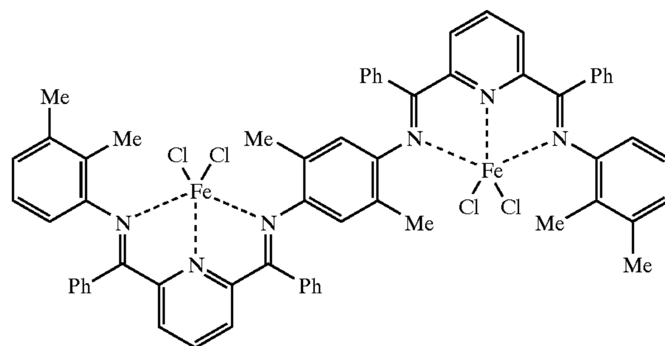
[COMPOUND 6]
