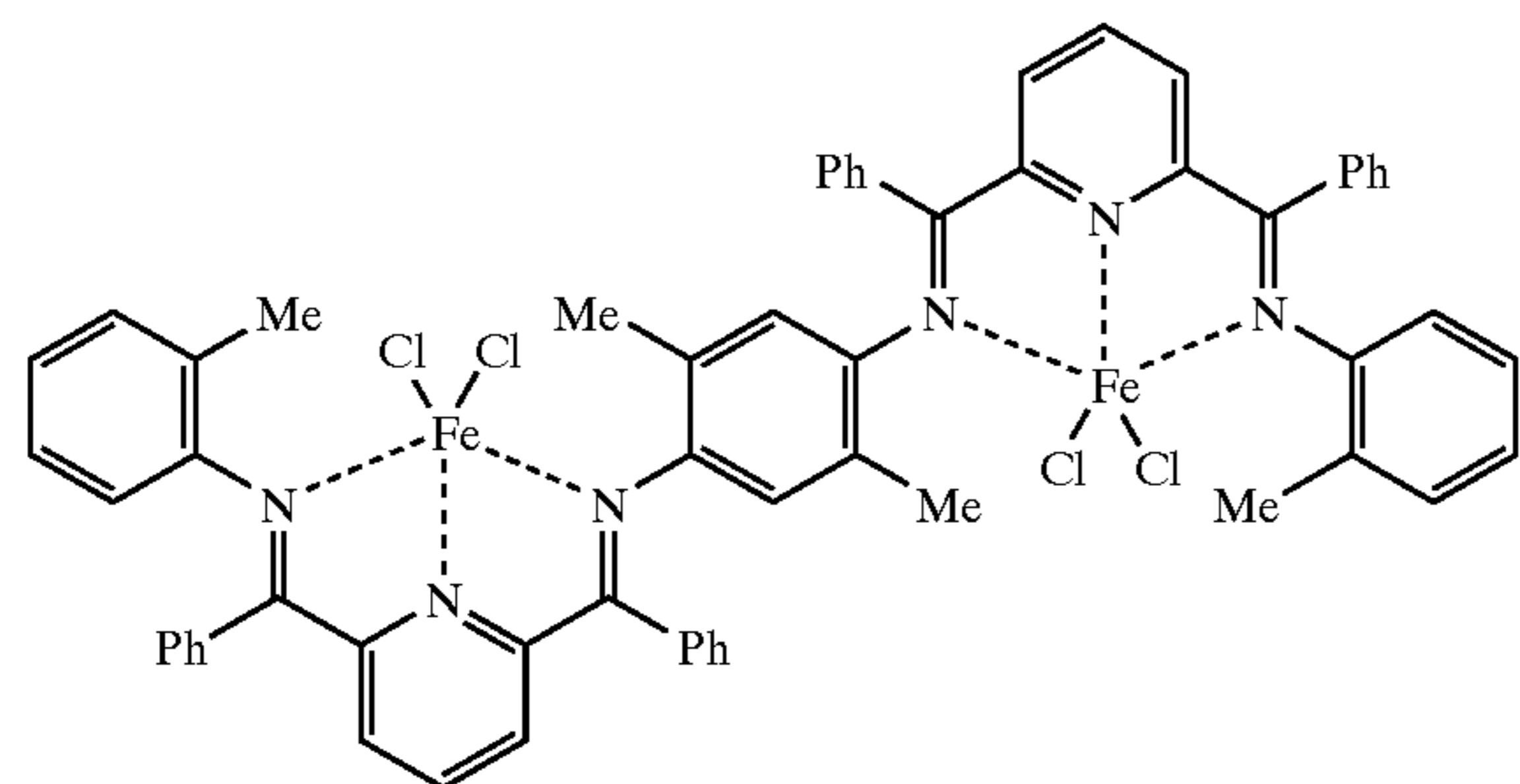
[COMPOUND 5]
