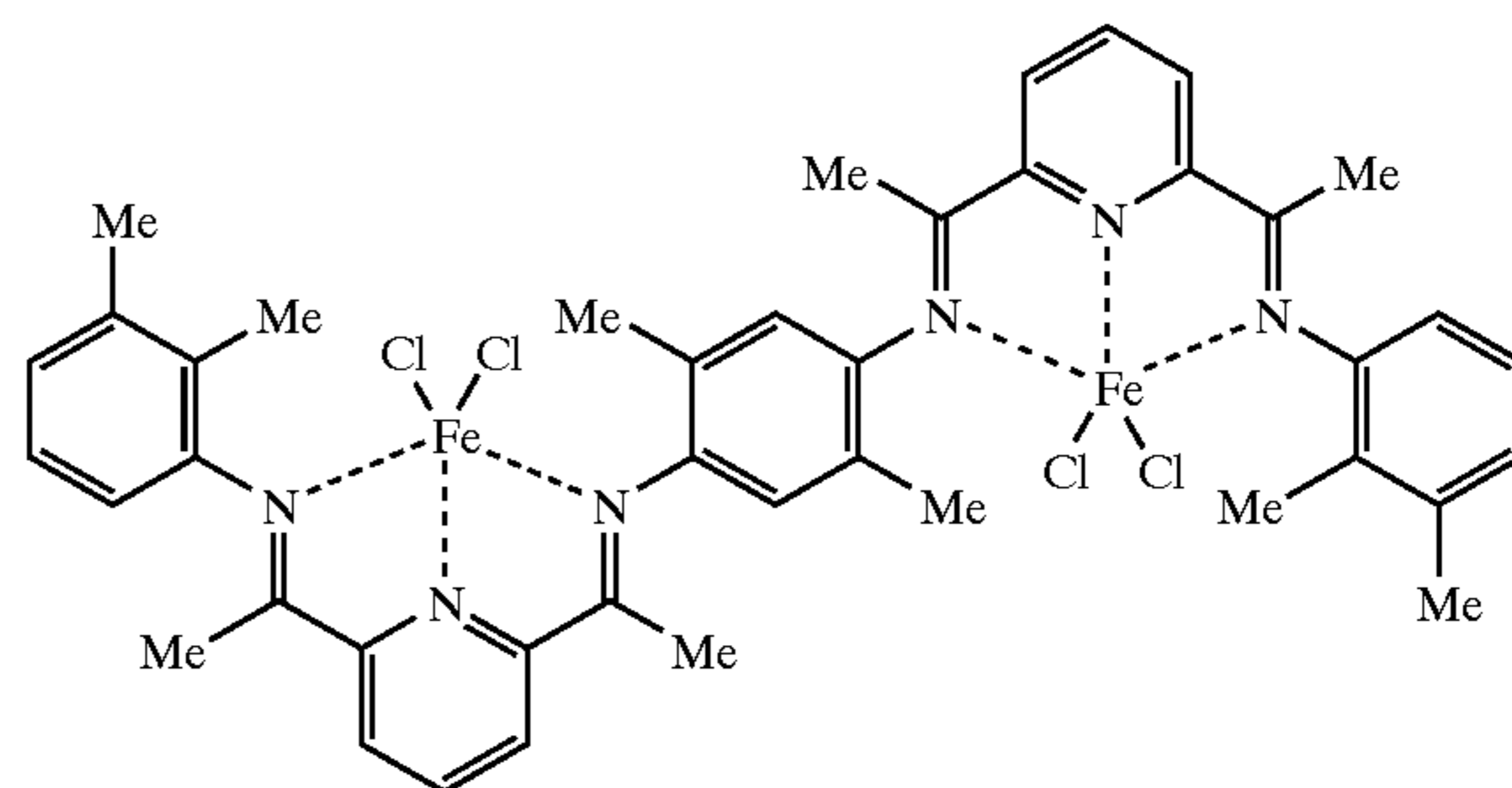
[COMPOUND 2]
