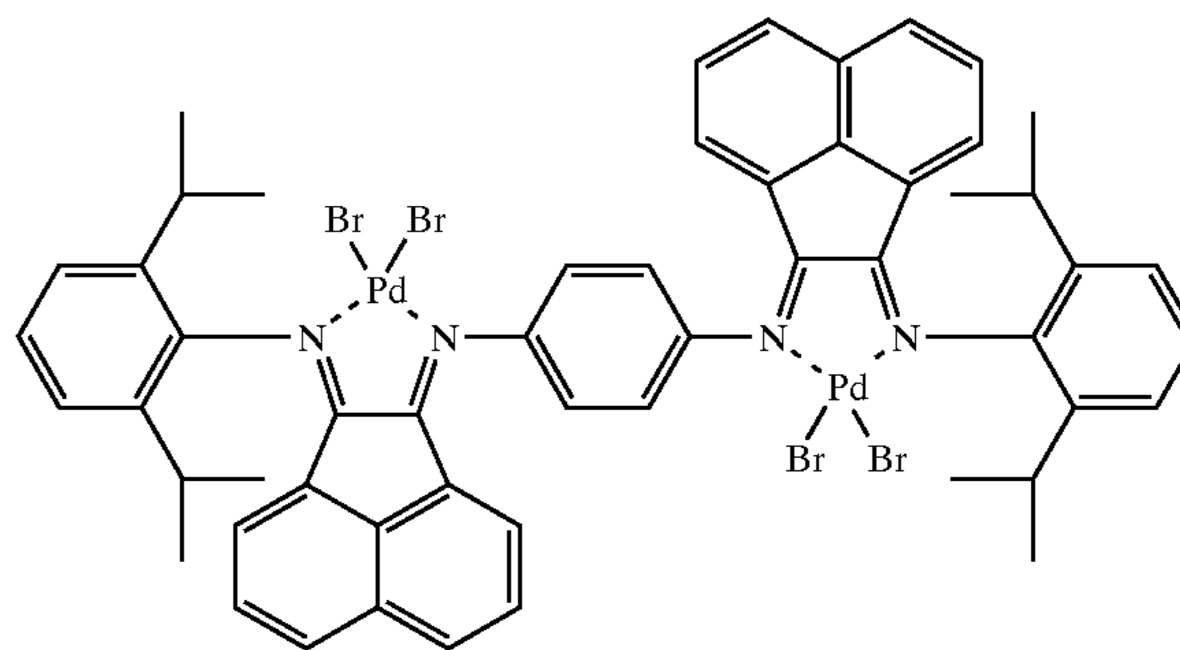
[COMPOUND 25]
