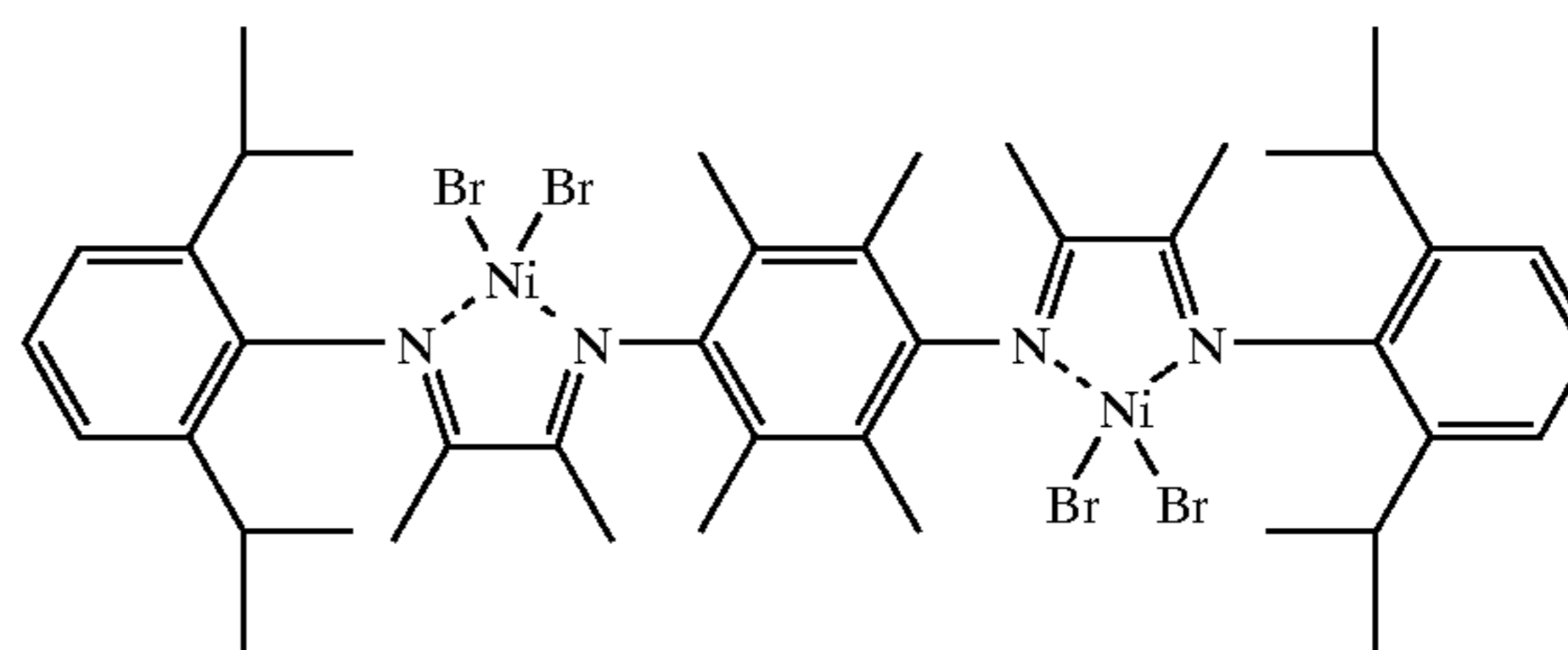
[COMPOUND 19]
