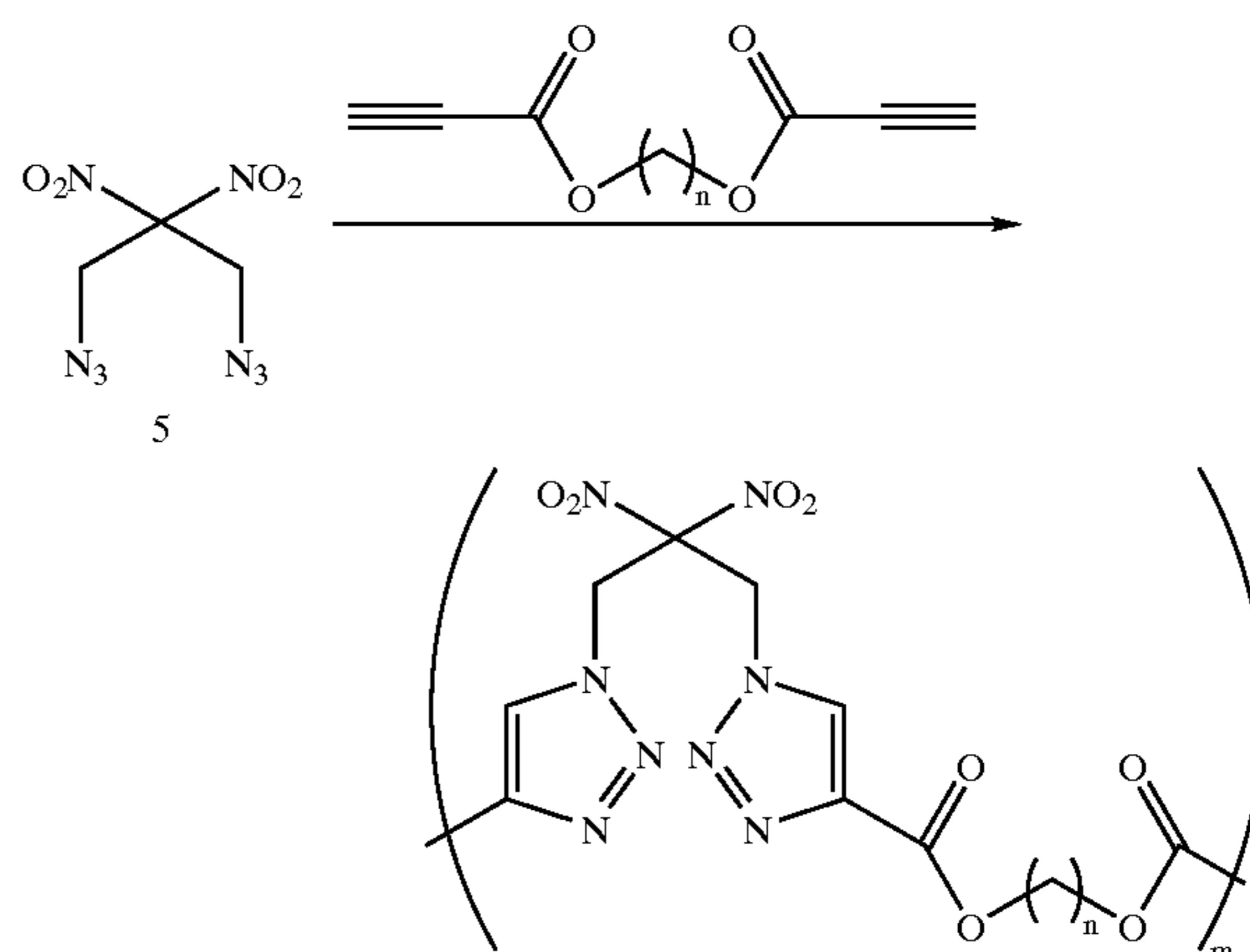
Scheme 5
