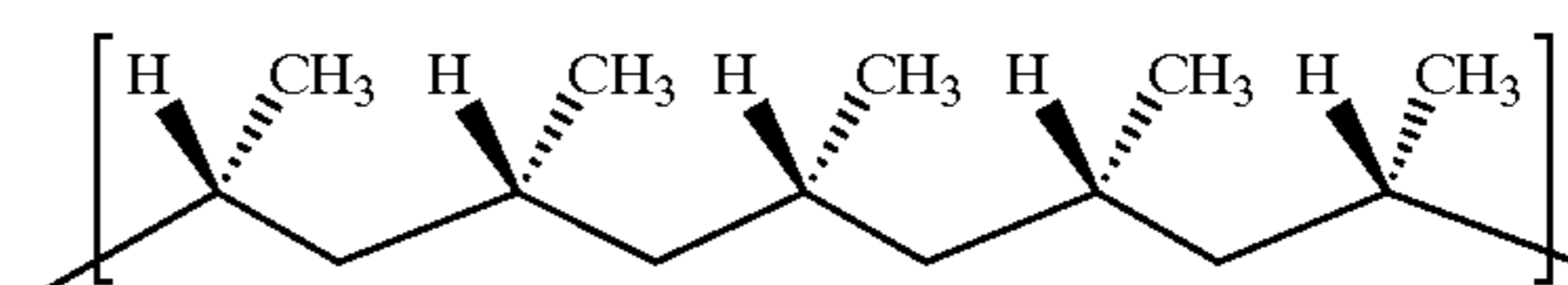
ISOTACTIC POLYPROPYLENE
