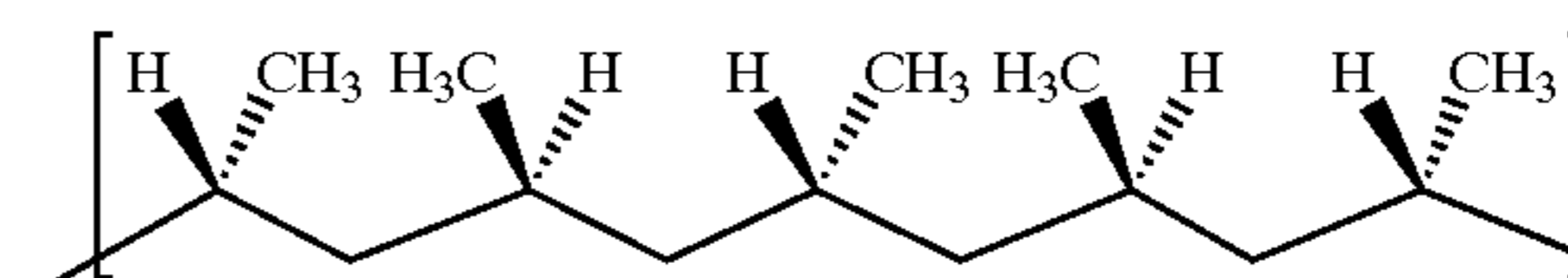
SYNDIOTACTIC POLYPROPYLENE
