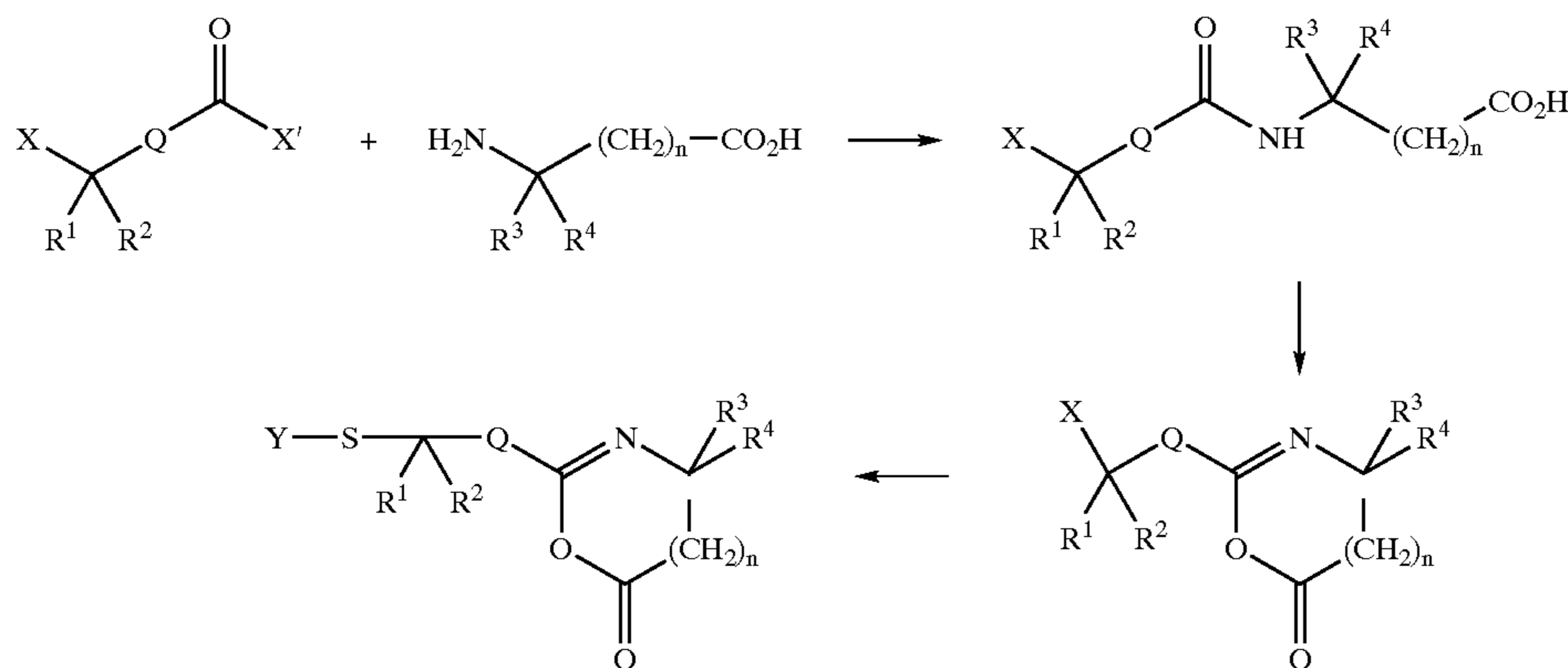
Scheme I
