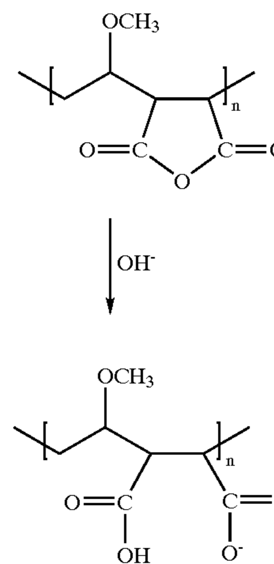
Reaction Scheme 1
