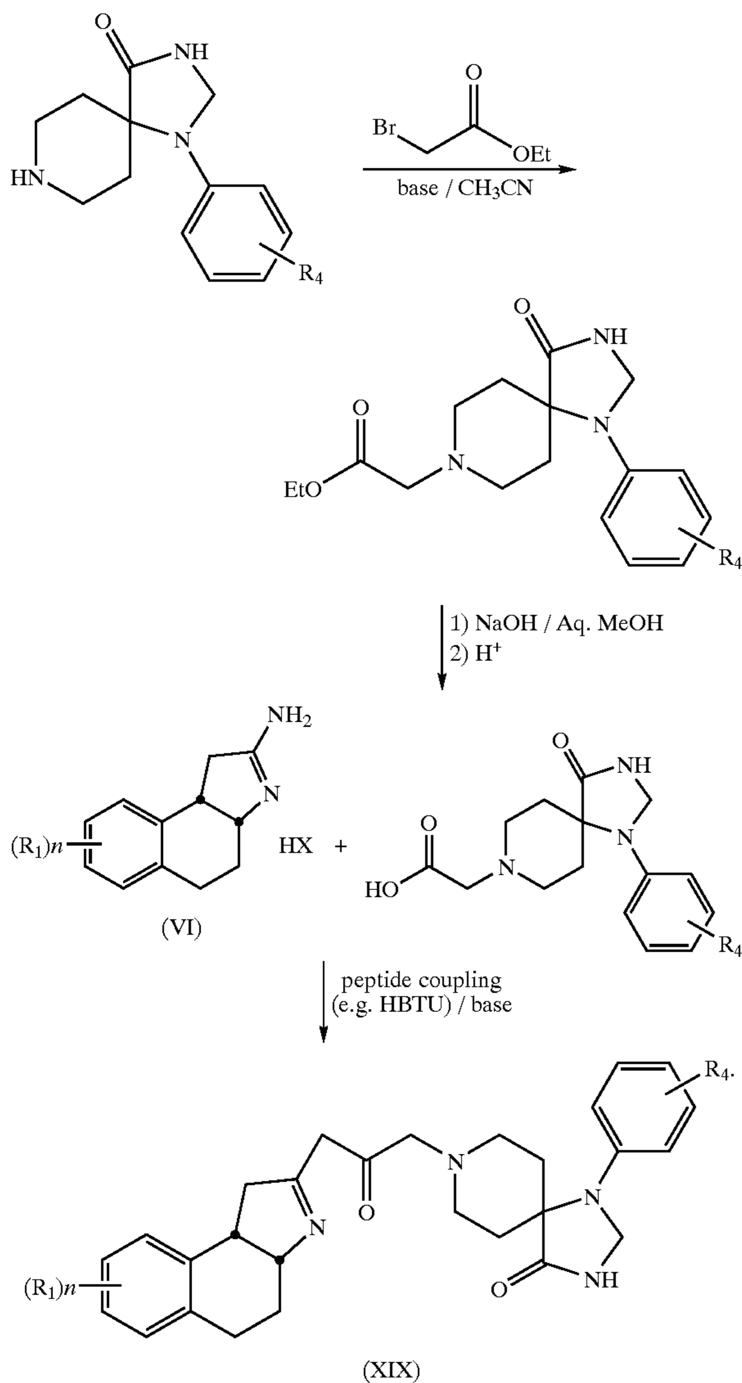
Scheme 9
