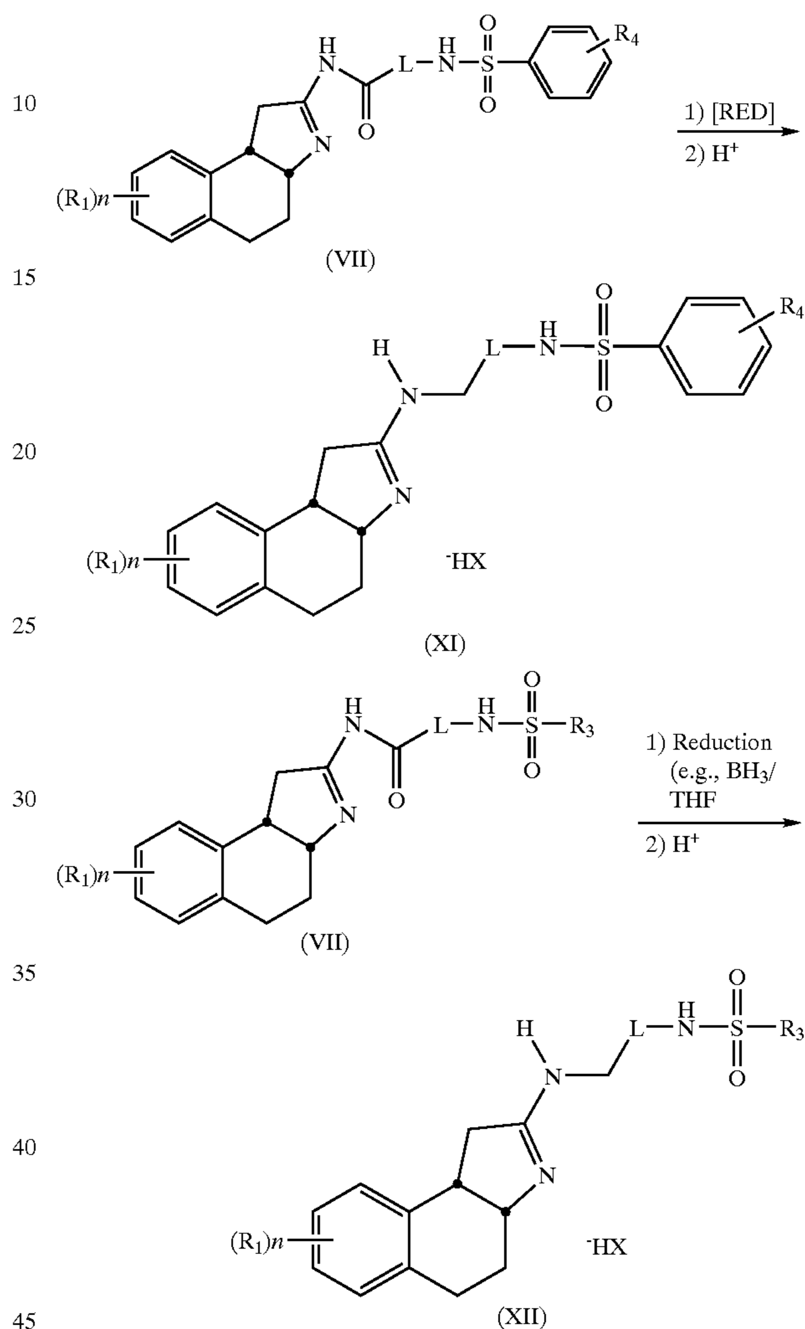
Scheme 3
