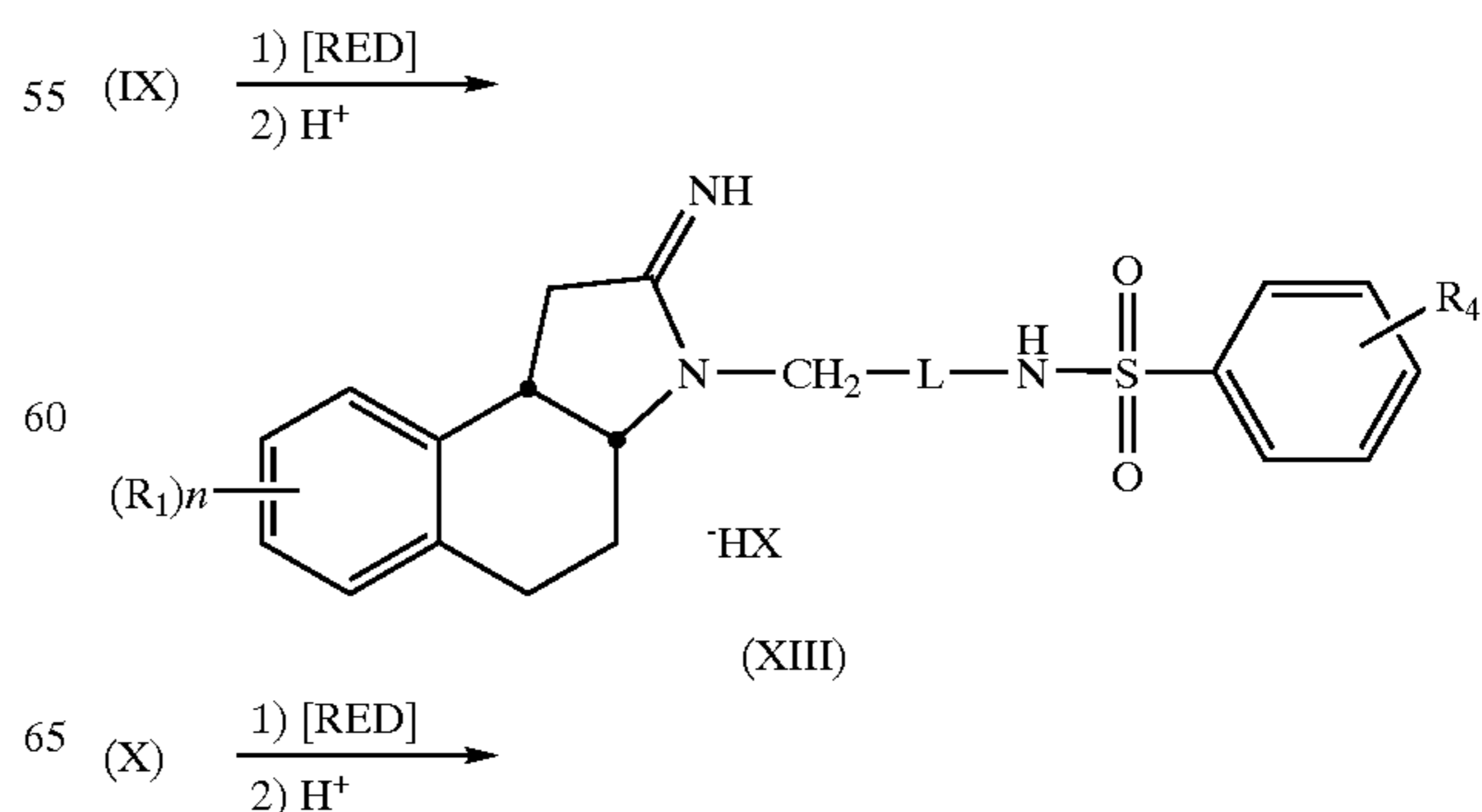
Scheme 4
