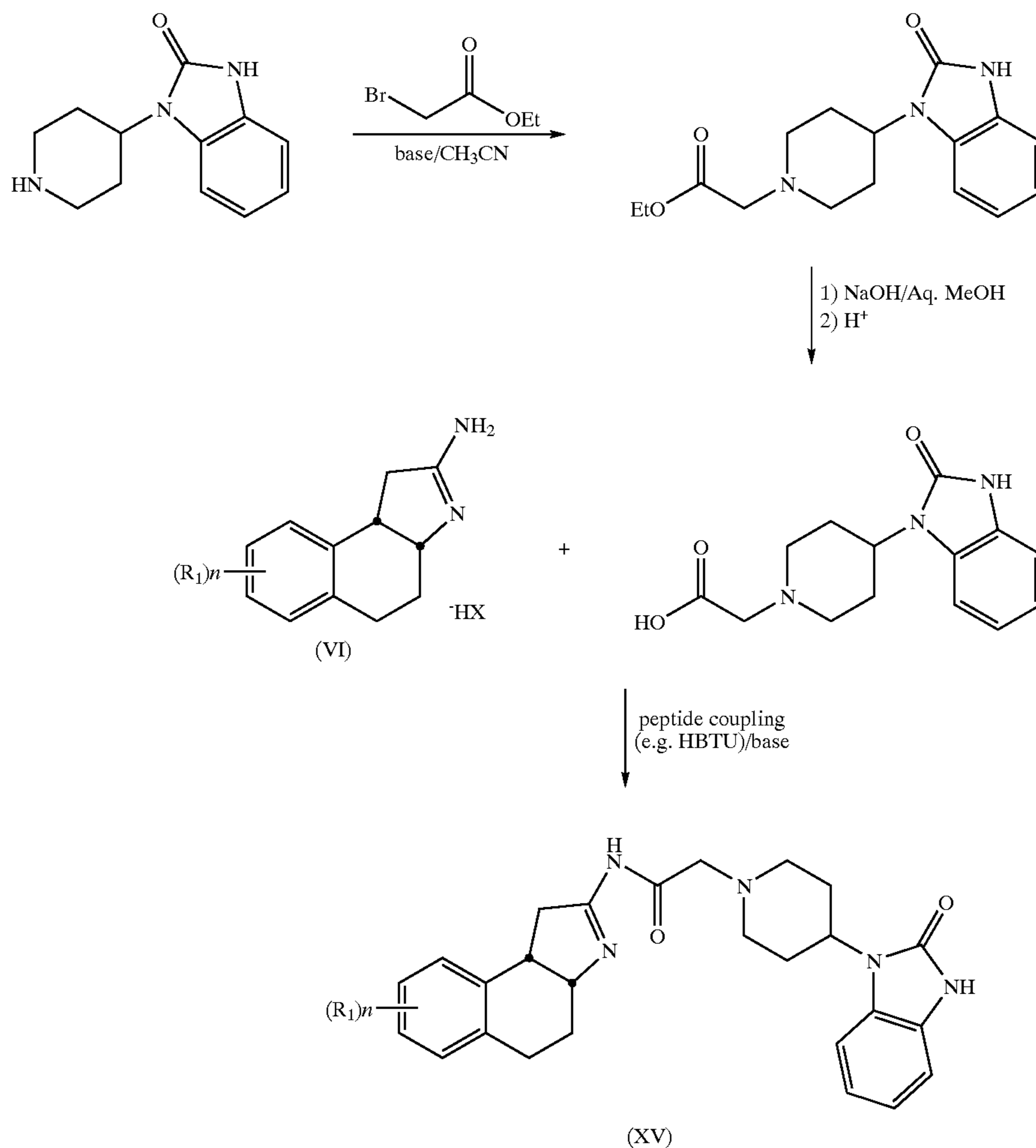
Scheme 5
