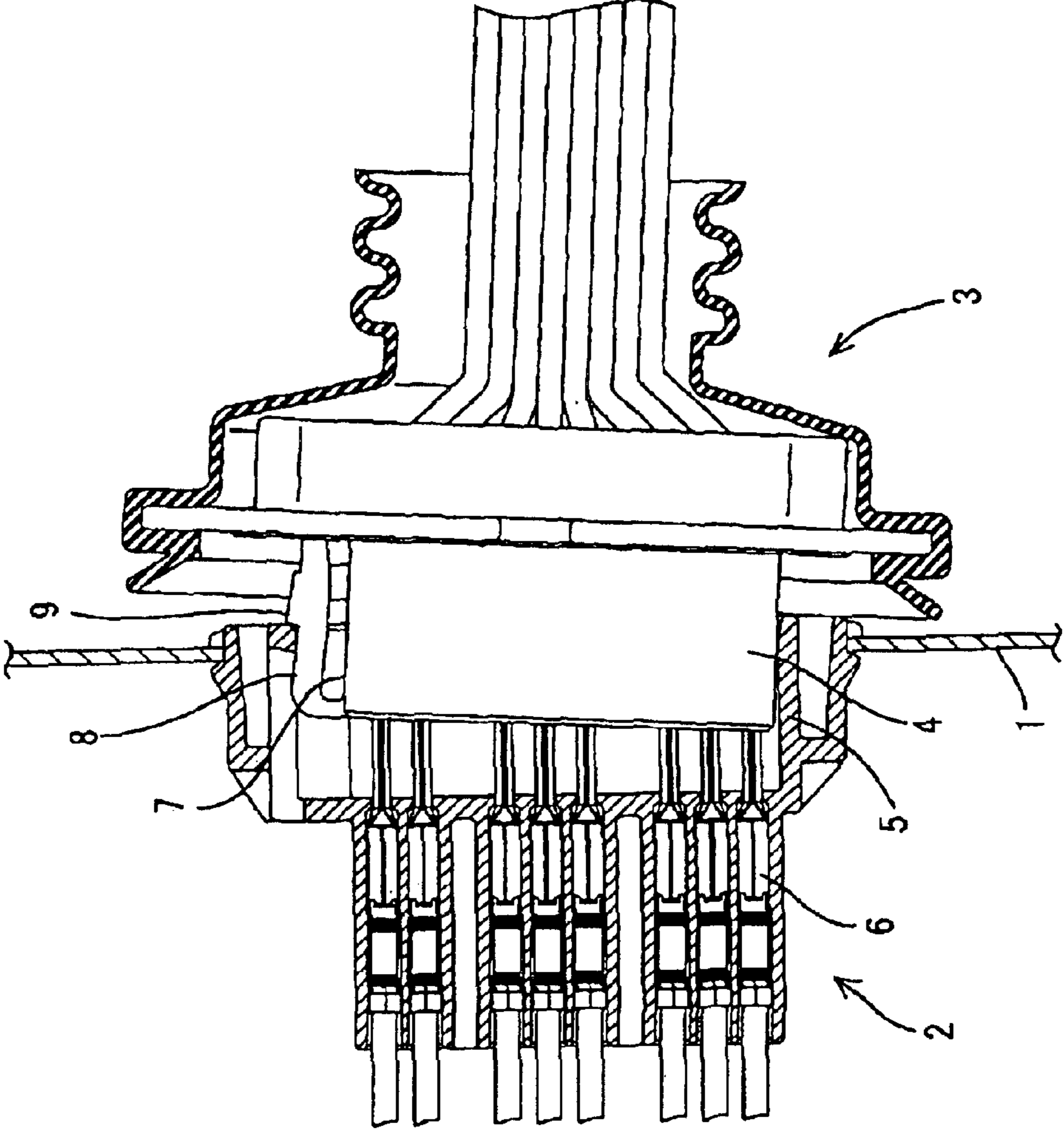
FIG. 9 PRIOR ART
