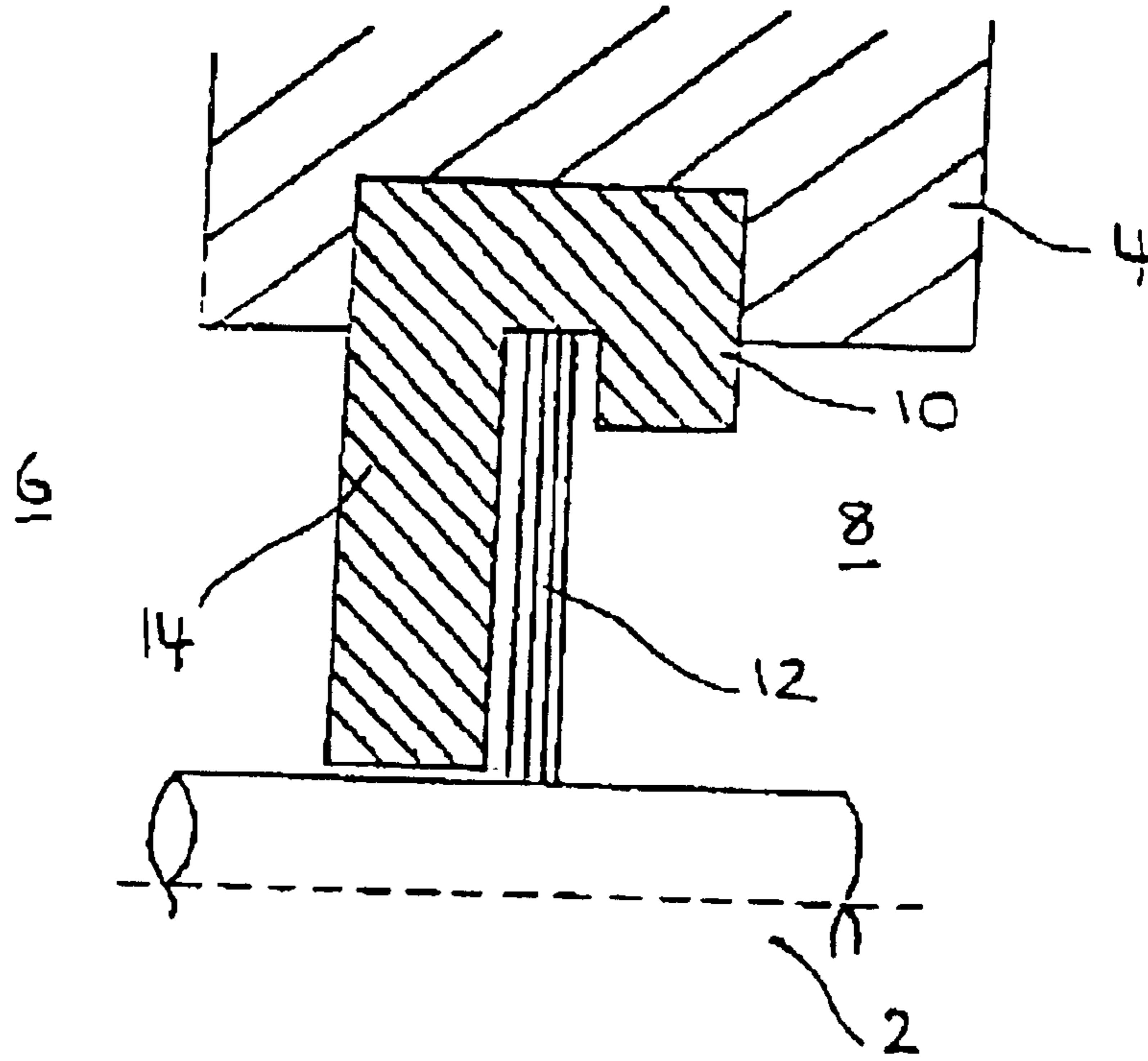
Figure 2 (PRIOR ART)
