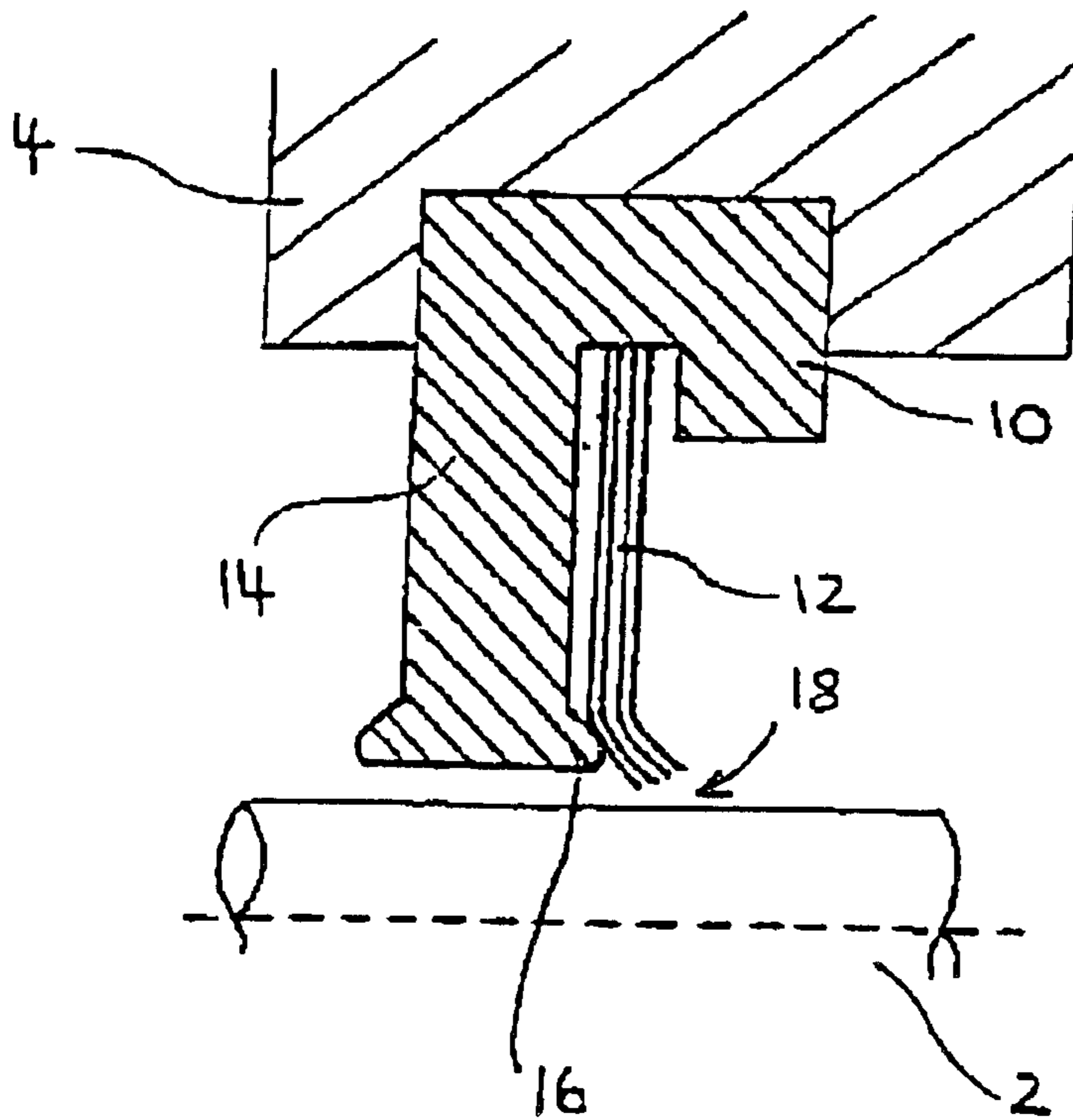
Figure 2 (PRIOR ART)
