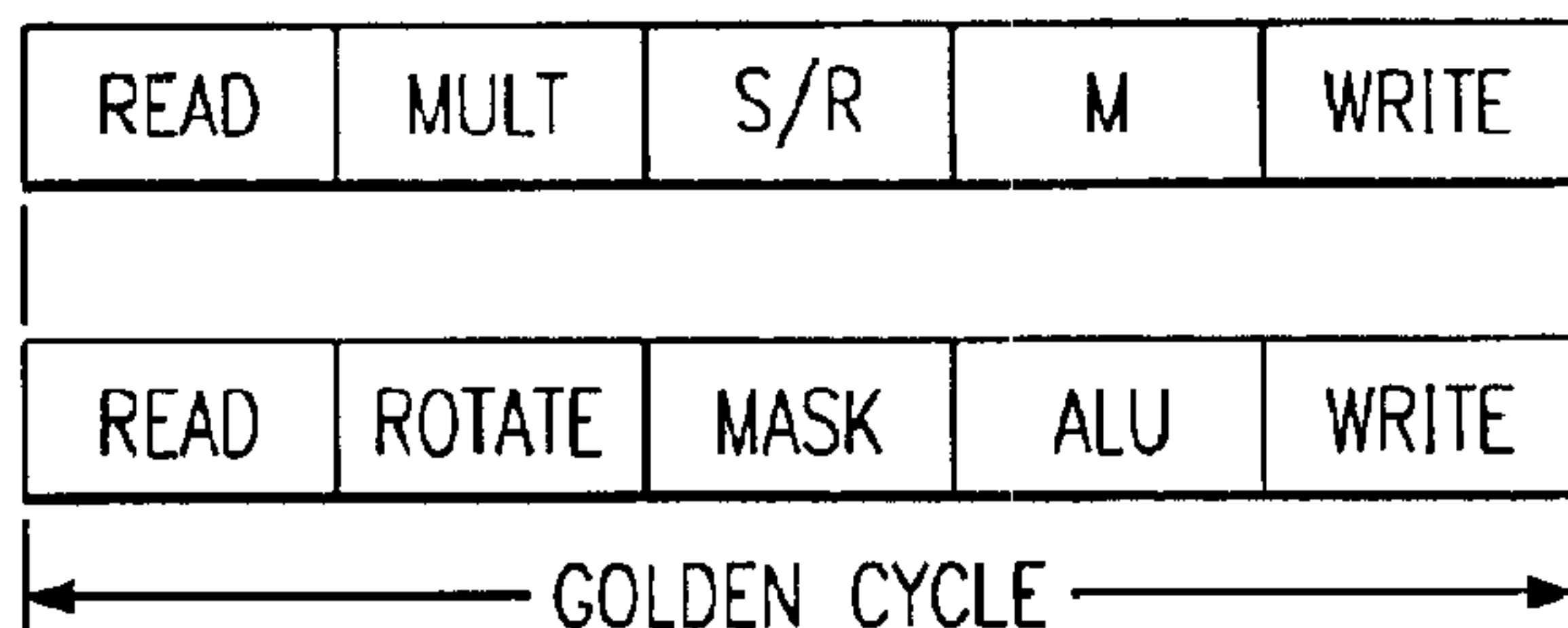
FIG. 16a (PRIOR ART)
