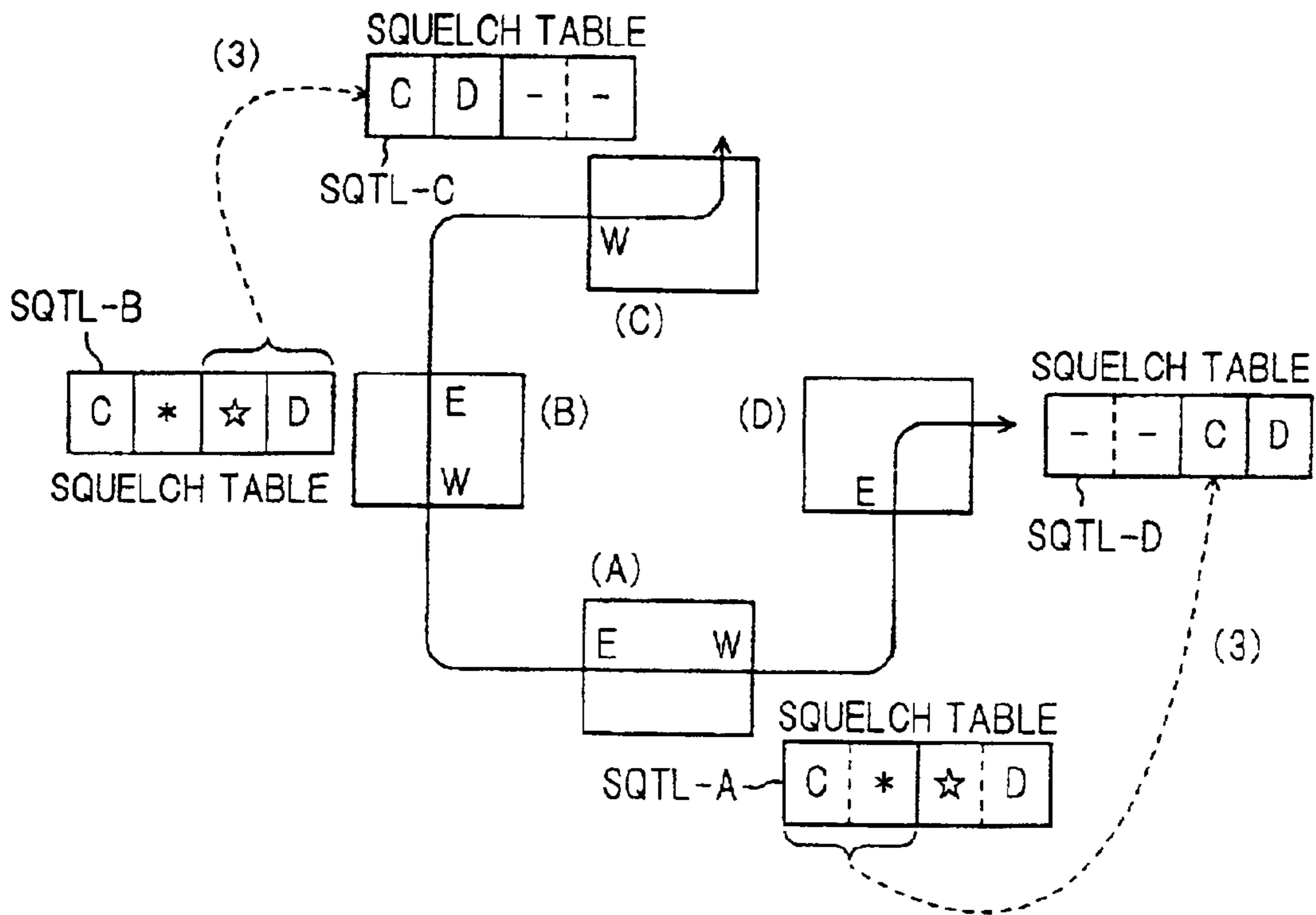
FIG. 33 PRIOR ART
