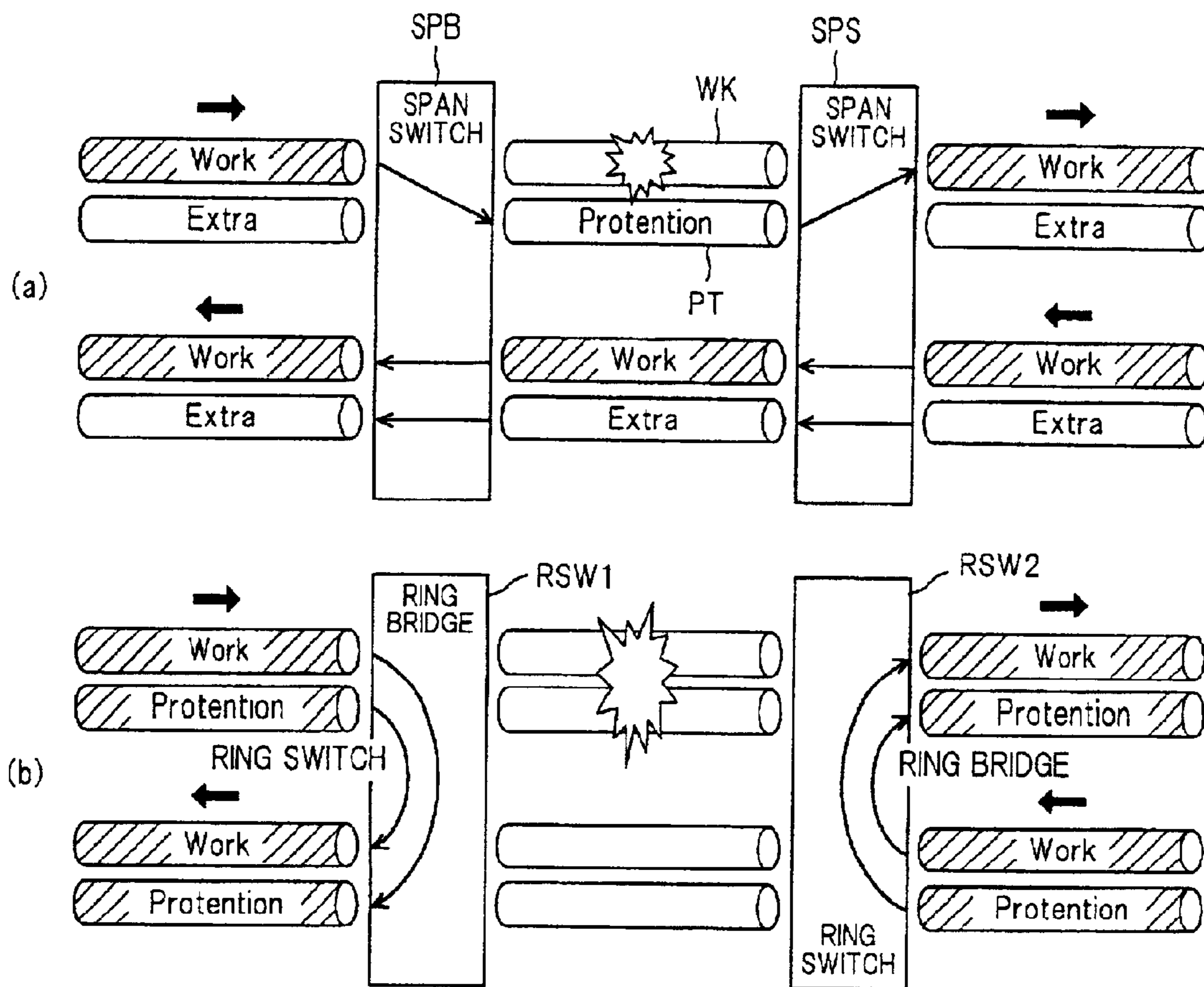
FIG. 37 PRIOR ART
