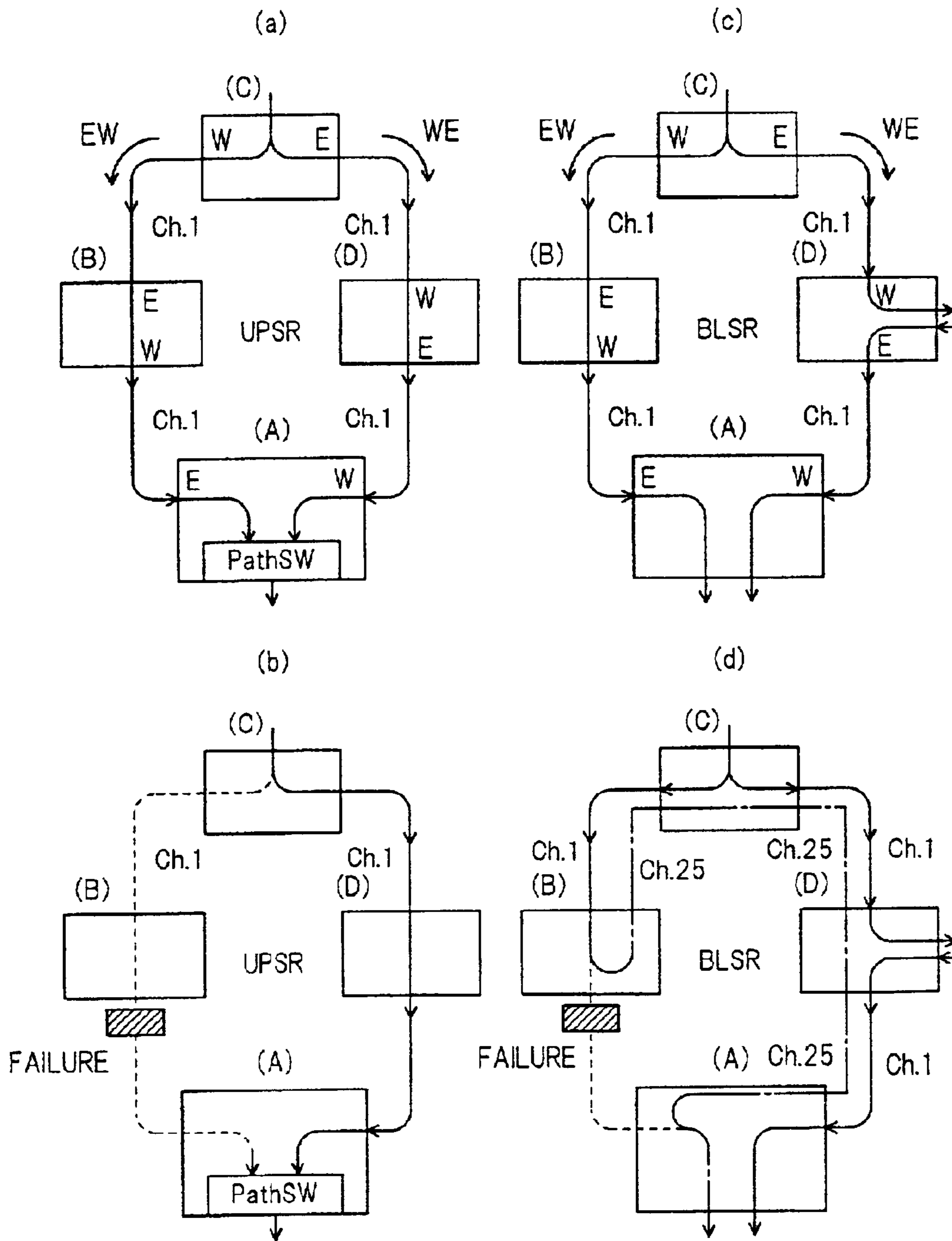
FIG. 21 PRIOR ART
