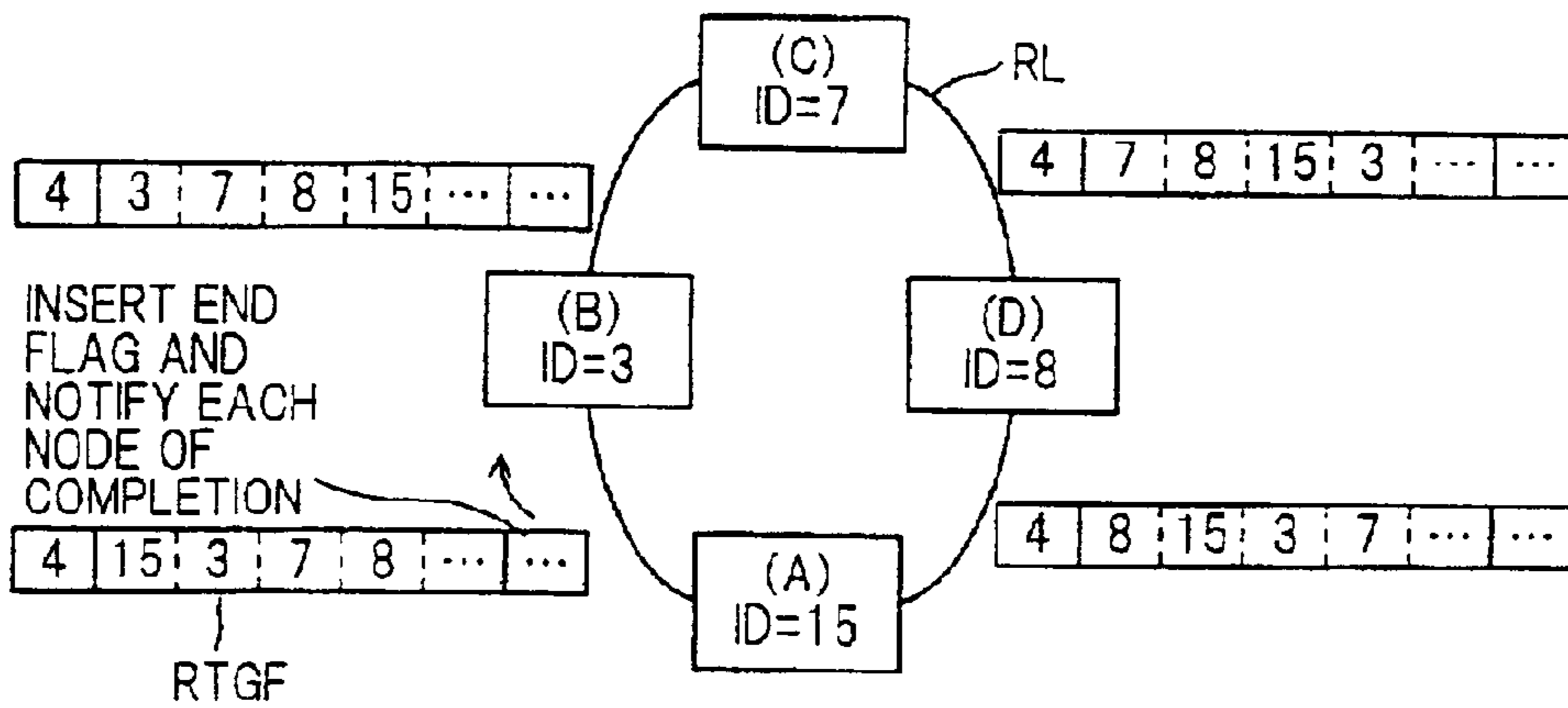
FIG. 30C PRIOR ART
