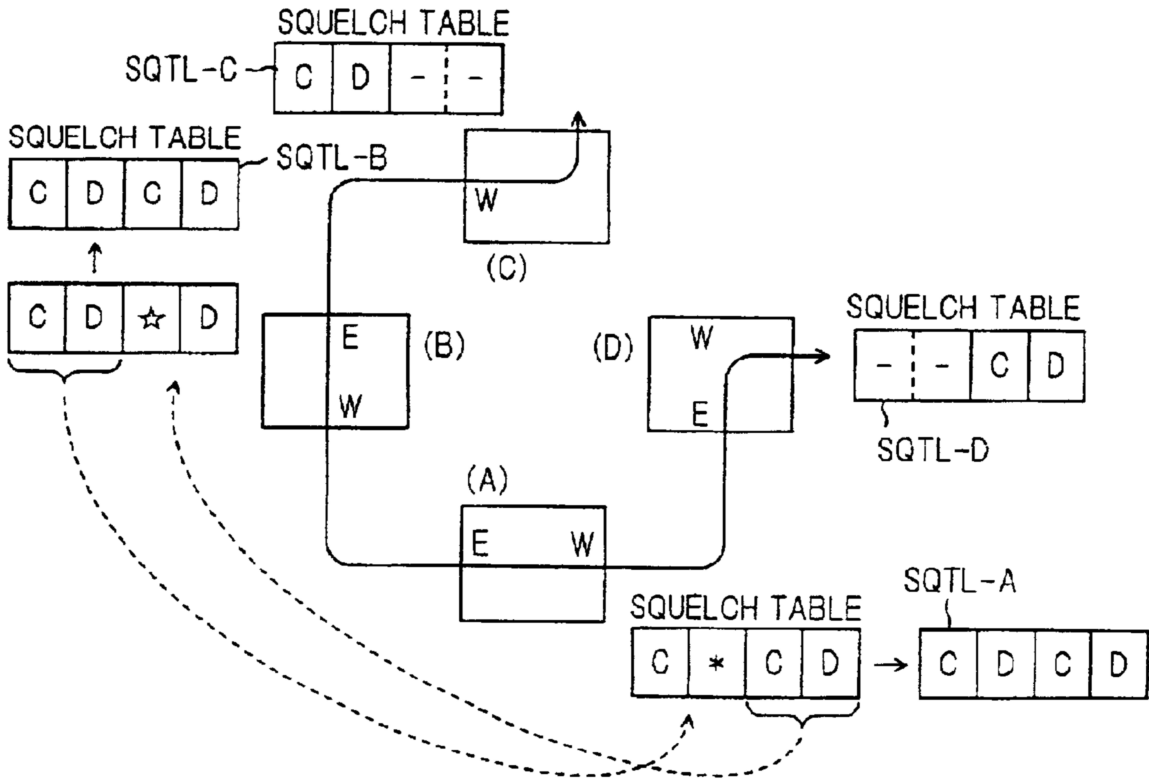
FIG. 35 PRIOR ART
