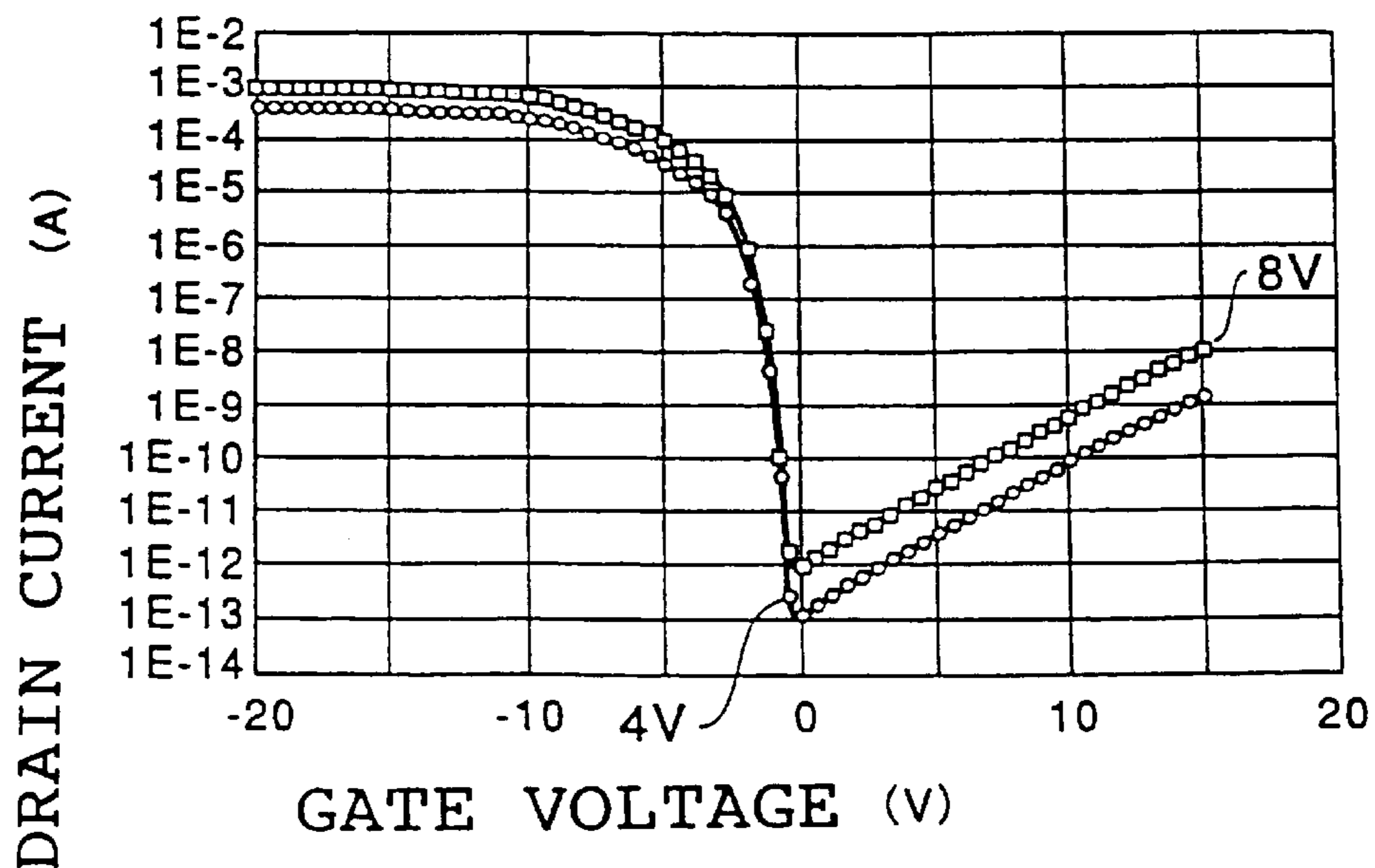
FIG. 12 AMPERE/VOLT CHARACTERISTICS P CHANNEL TYPE TFT
