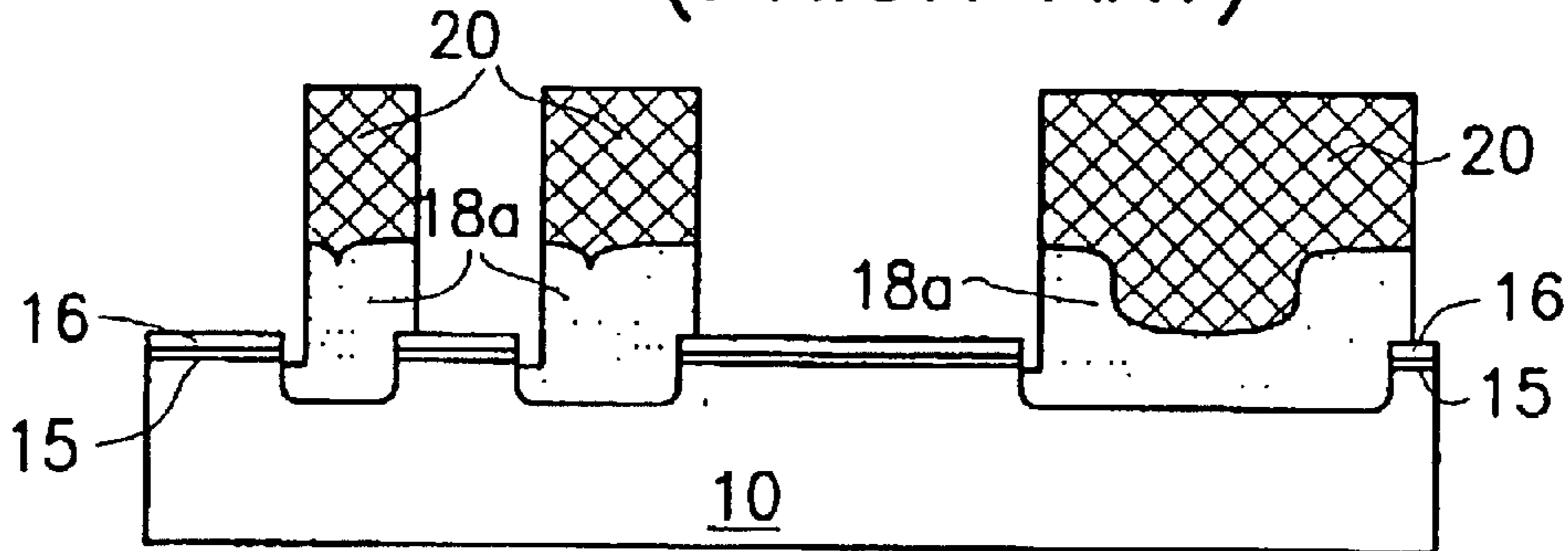
FIG. 1C (PRIOR ART)
