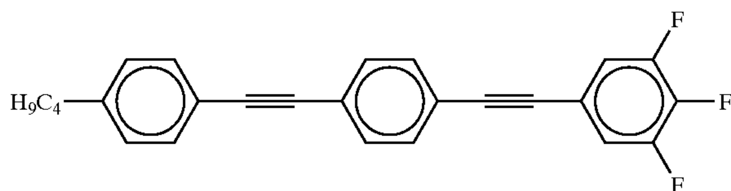
(Structure X)
