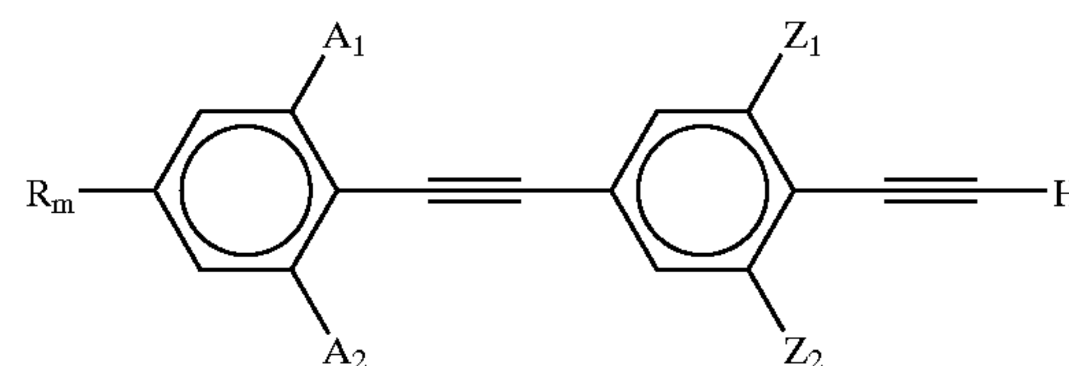
(Structure 10)
