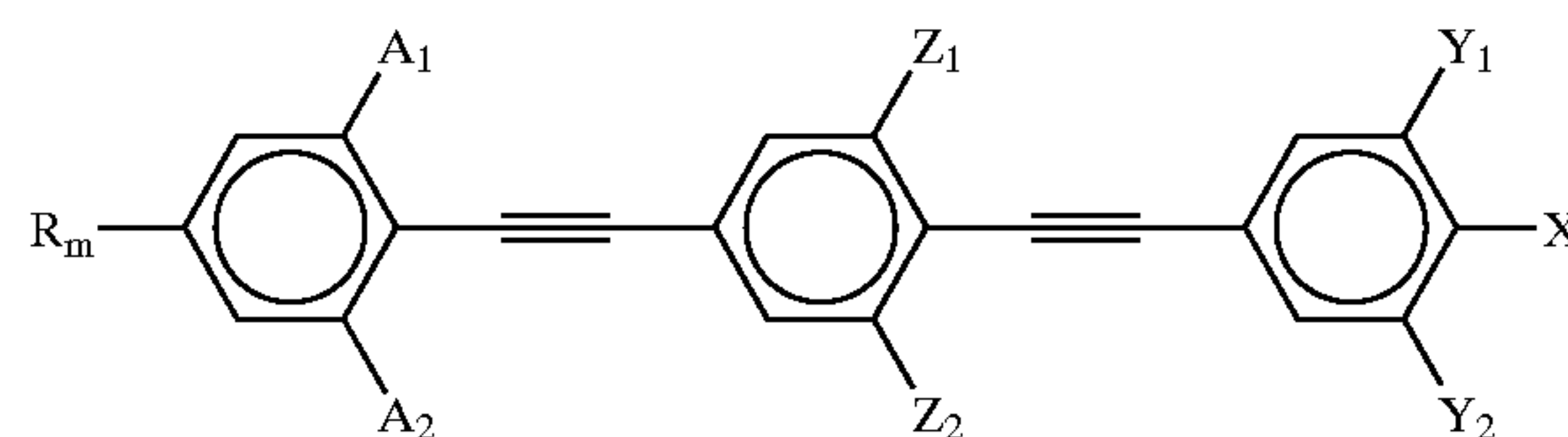
(Structure 11)
