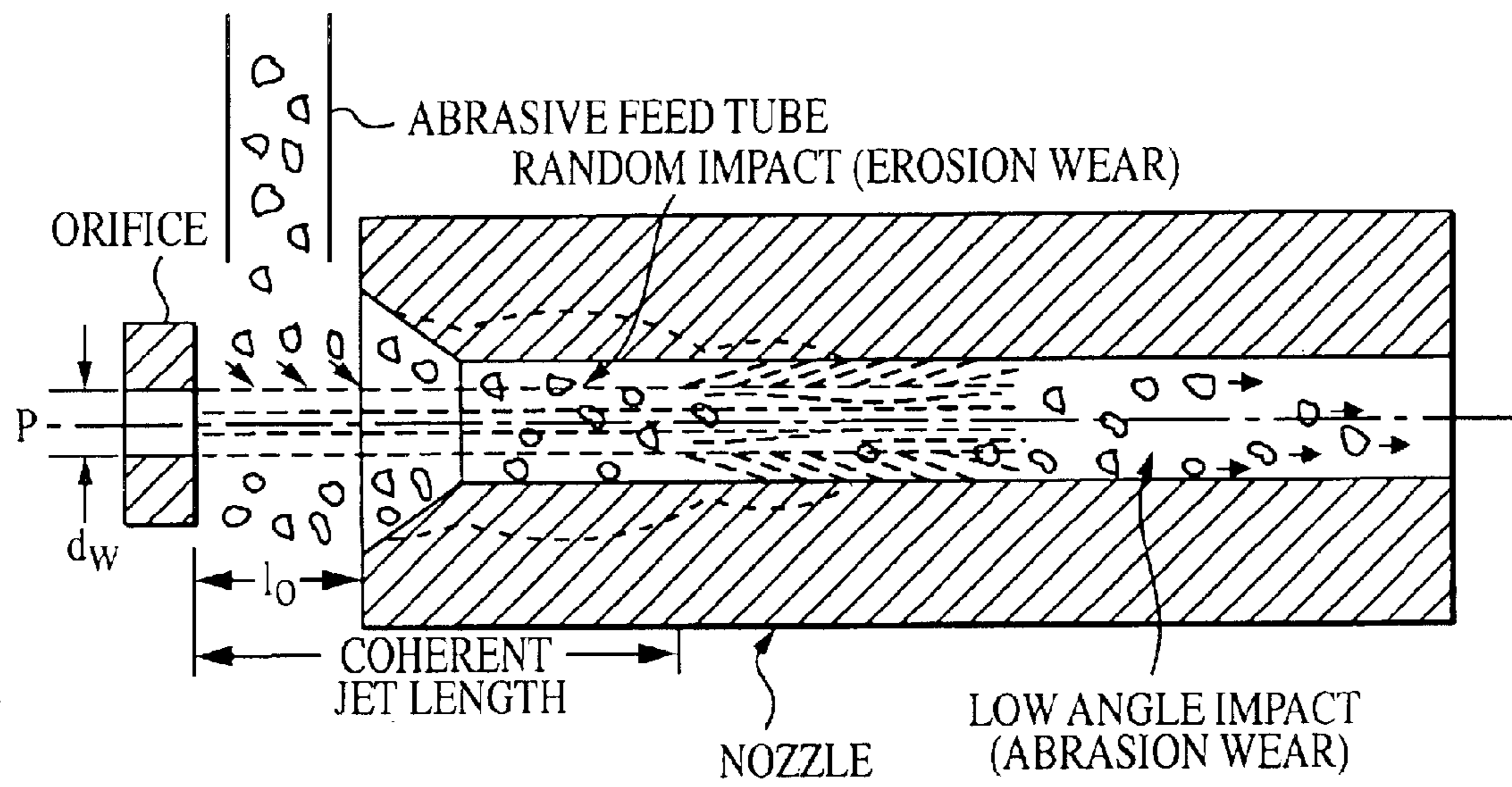
FIG. 3 PRIOR ART
