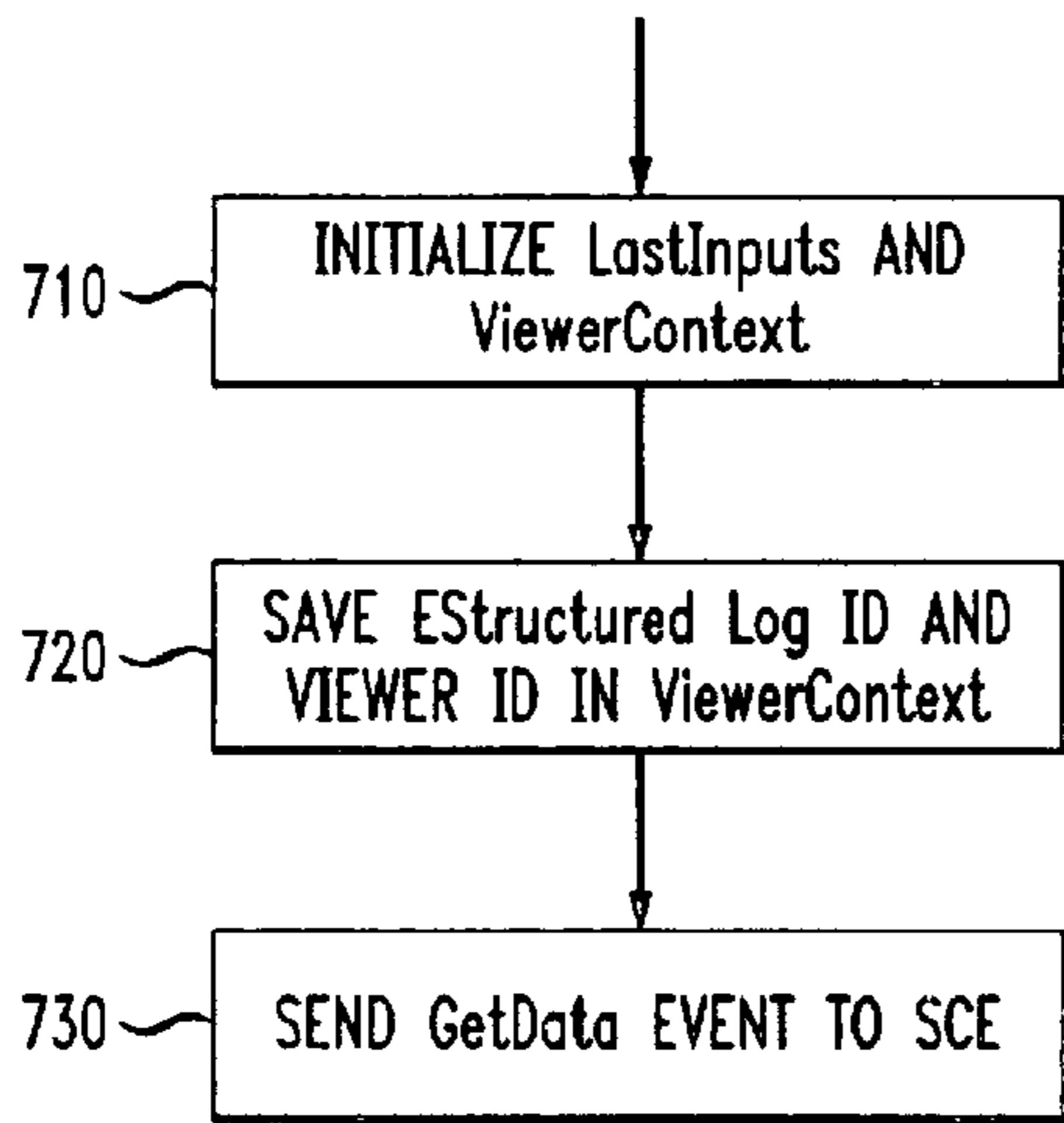
FIG. 10A A VIEWER PROCESS WHEN SCE/INITIALIZE EVENT IS RECEIVED
