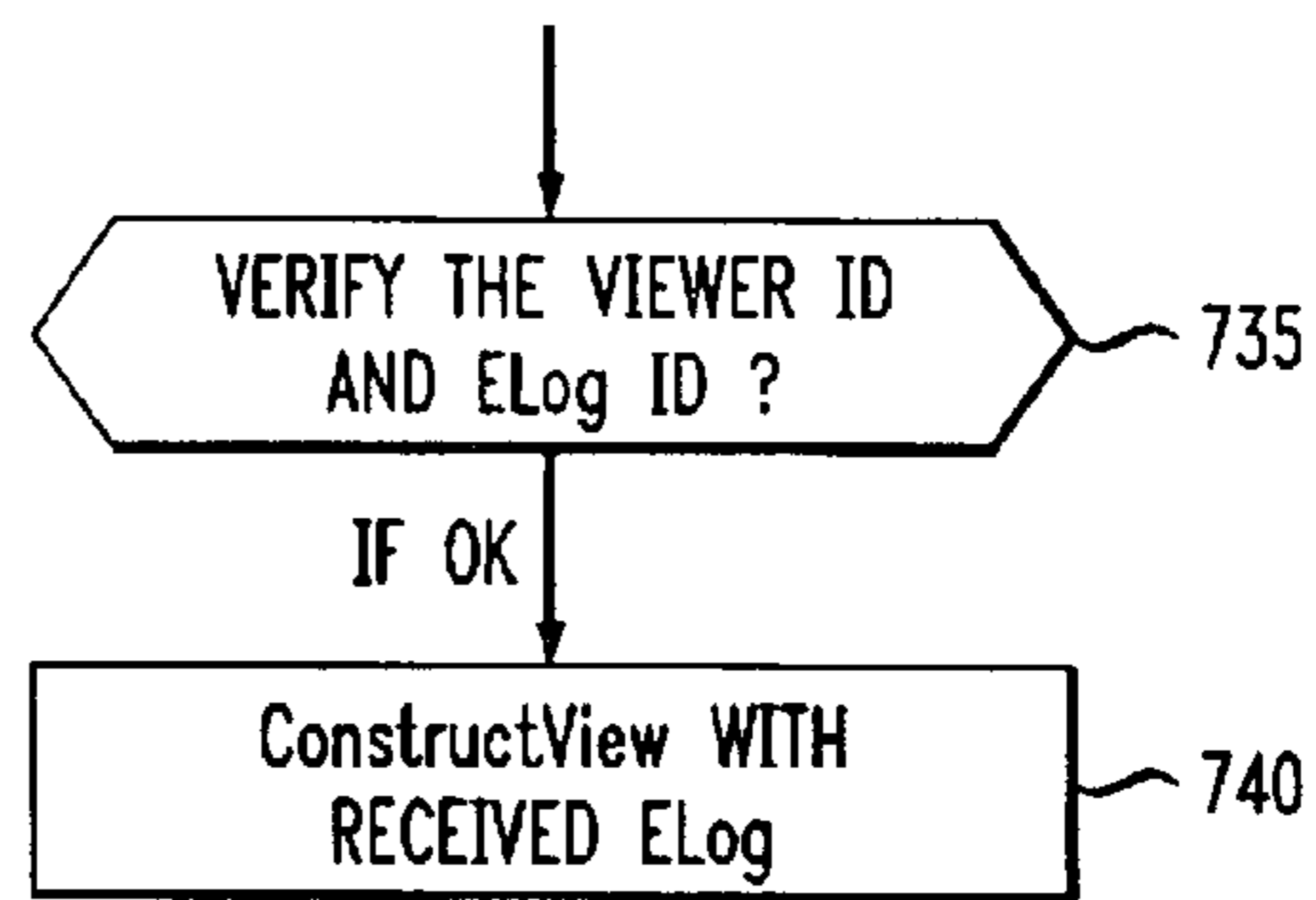
FIG. 10B A VIEWER PROCESS WHEN SCE/UpdateViewer EVENT IS RECEIVED
