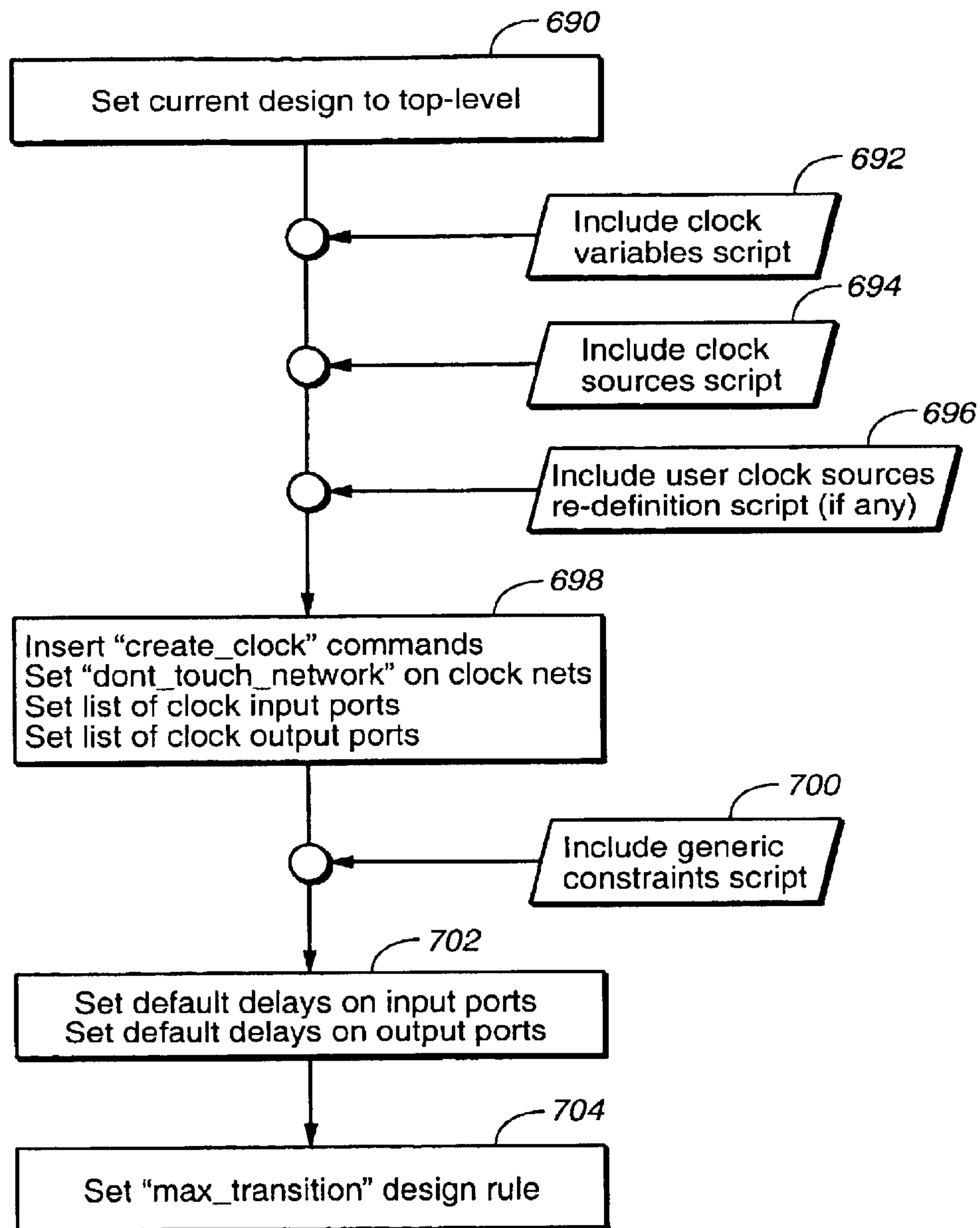
FIG. 31 : Structure of constraints setting on top-level
