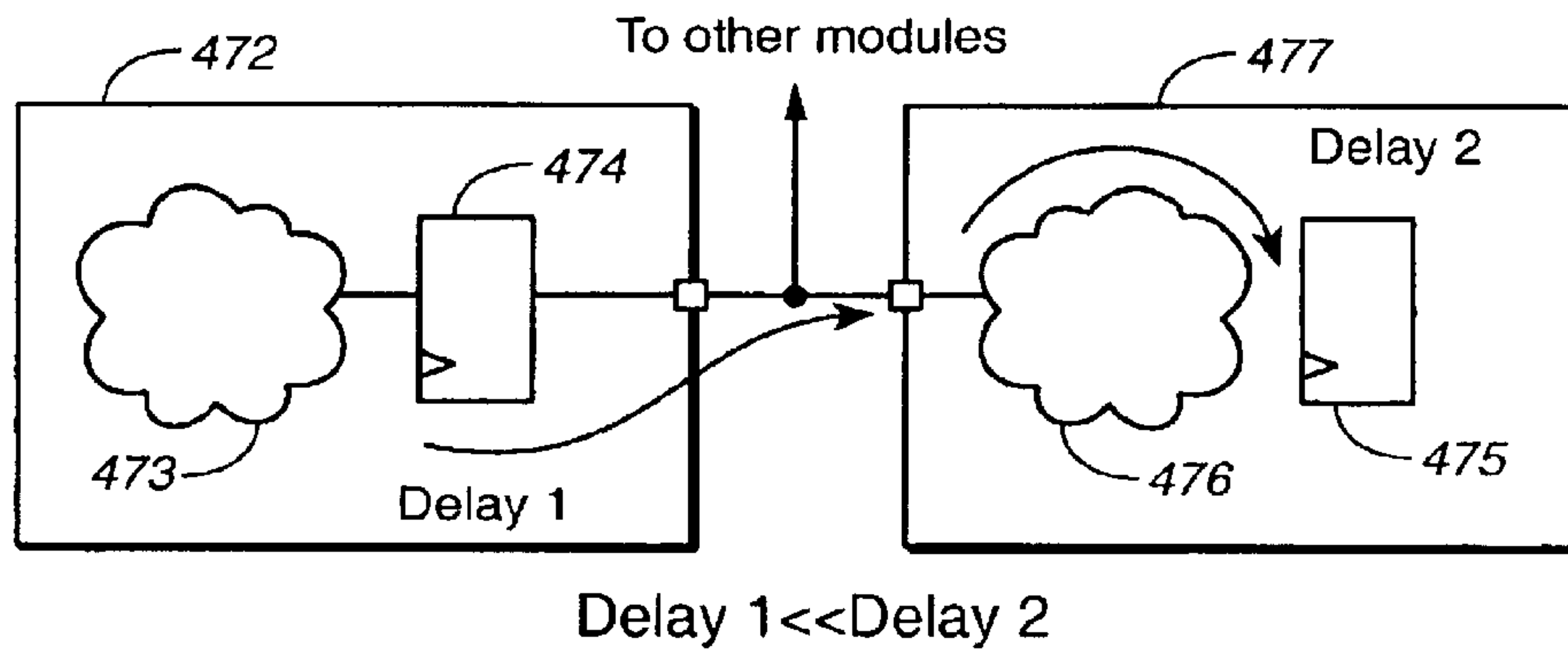
FIG. 20B : In the absence of broken timing paths
