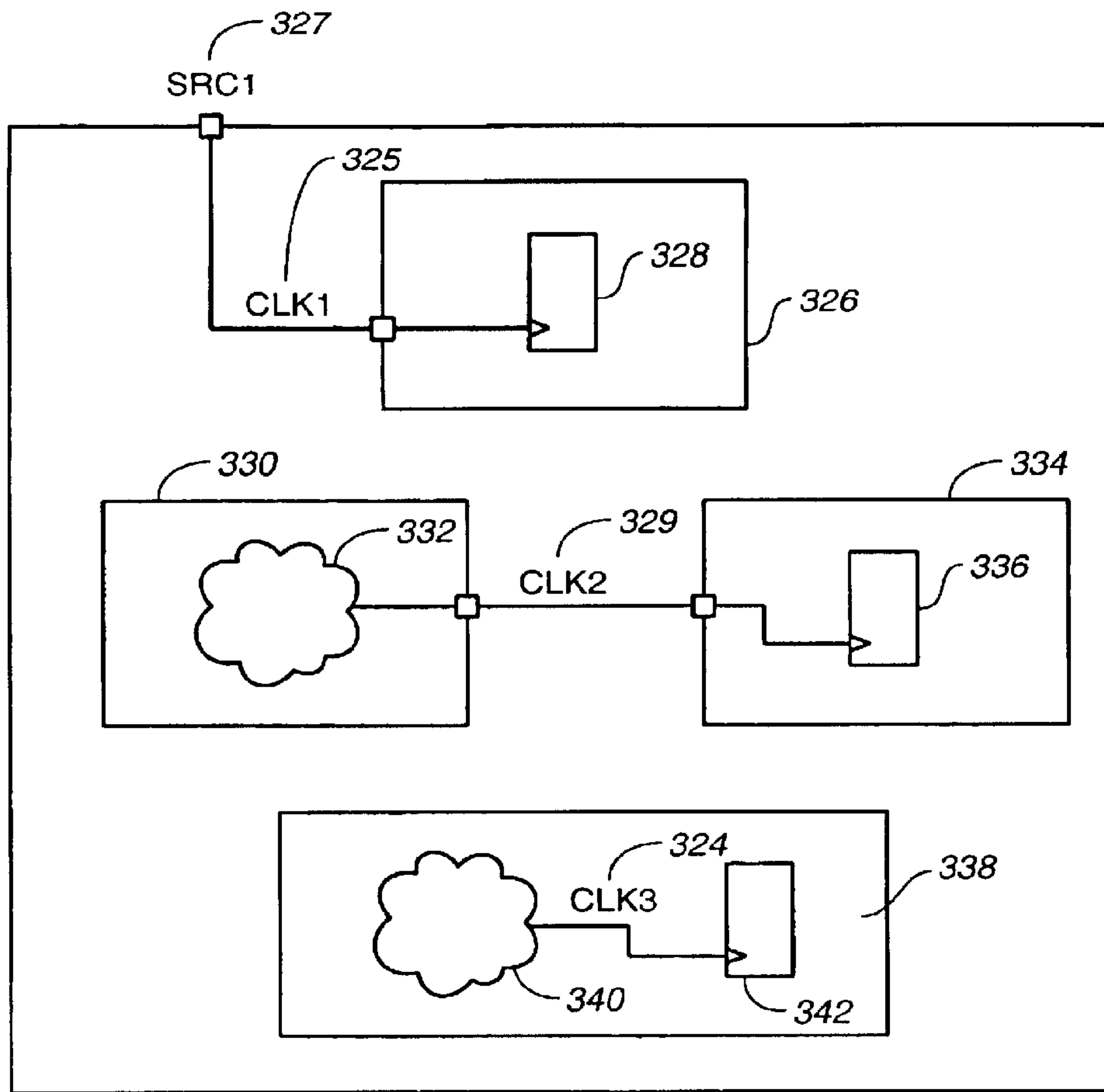
FIG. 39 : External and internal clocks.
