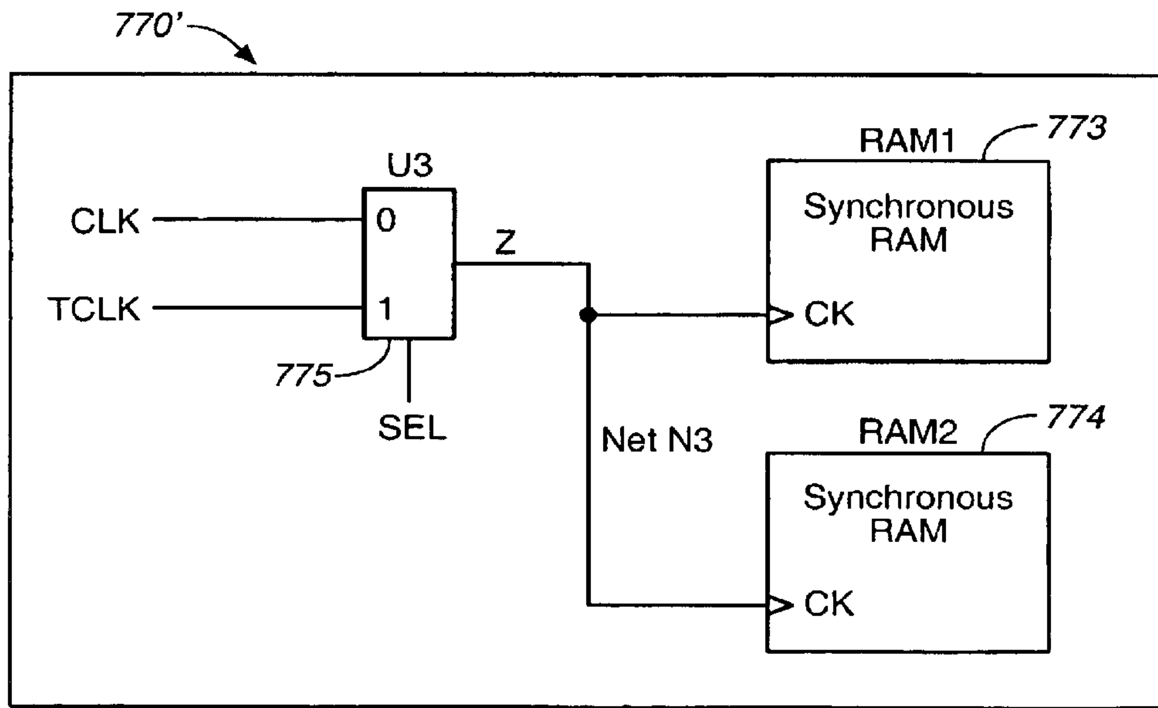
(b) After initial mapping
