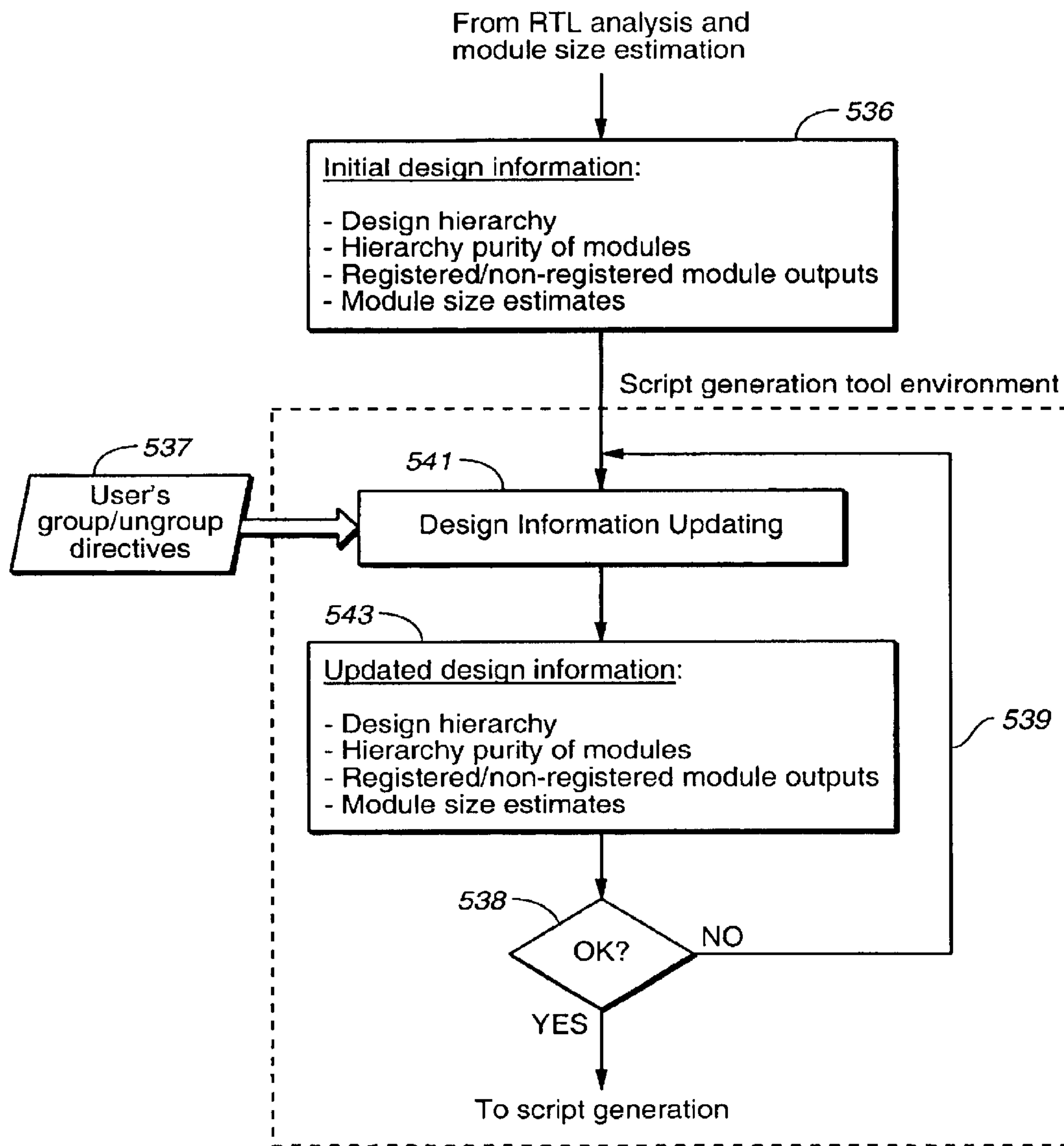
FIG. 24 : Support for design hierarchy re-arrangement
