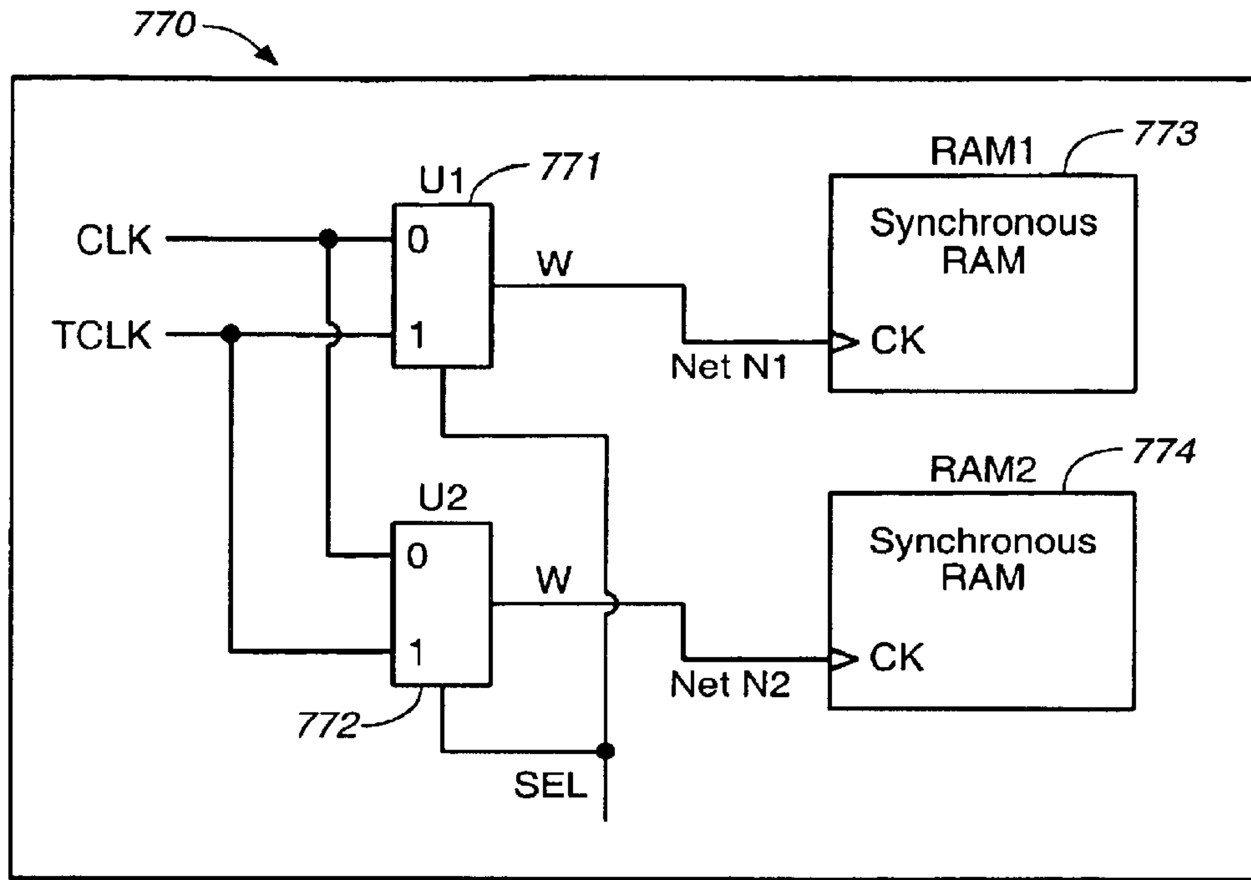
(a) Before initial mapping
