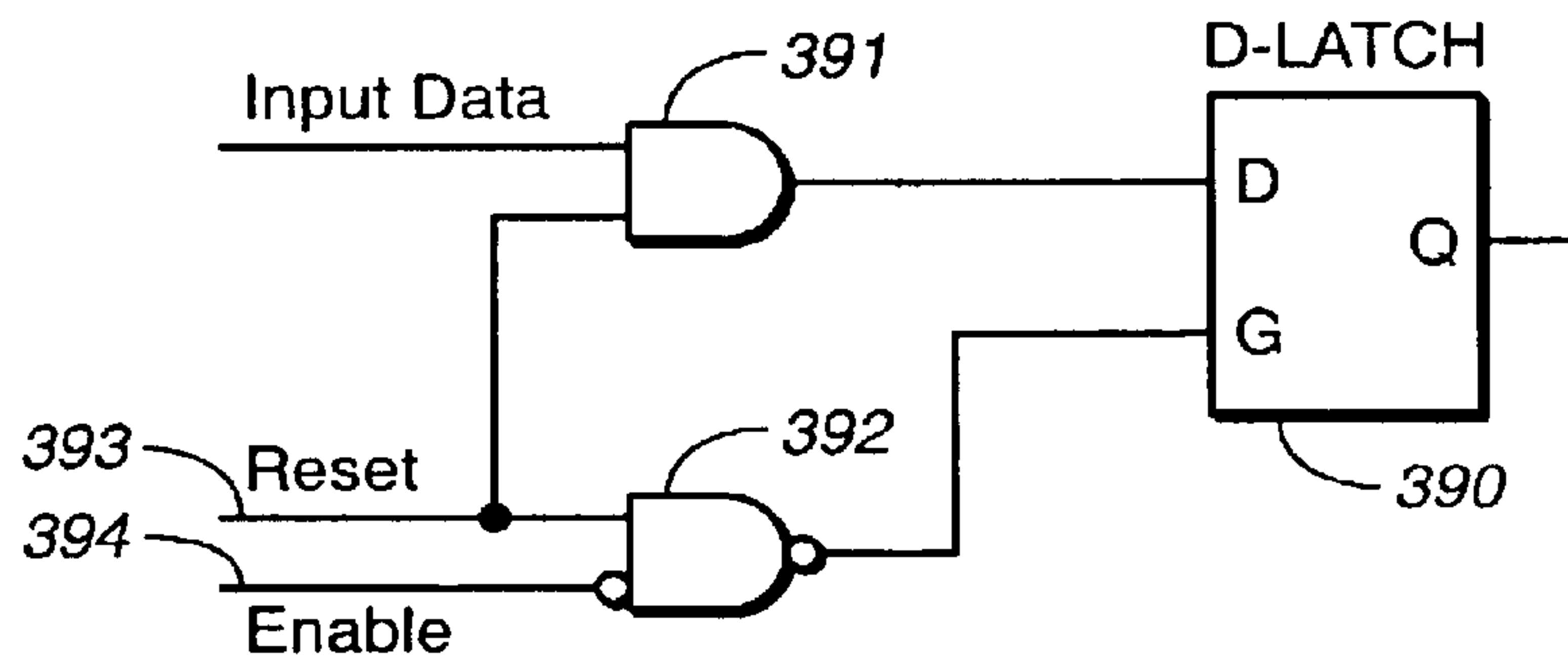
FIG. 37 : Failing implementation of a latch with clear.
