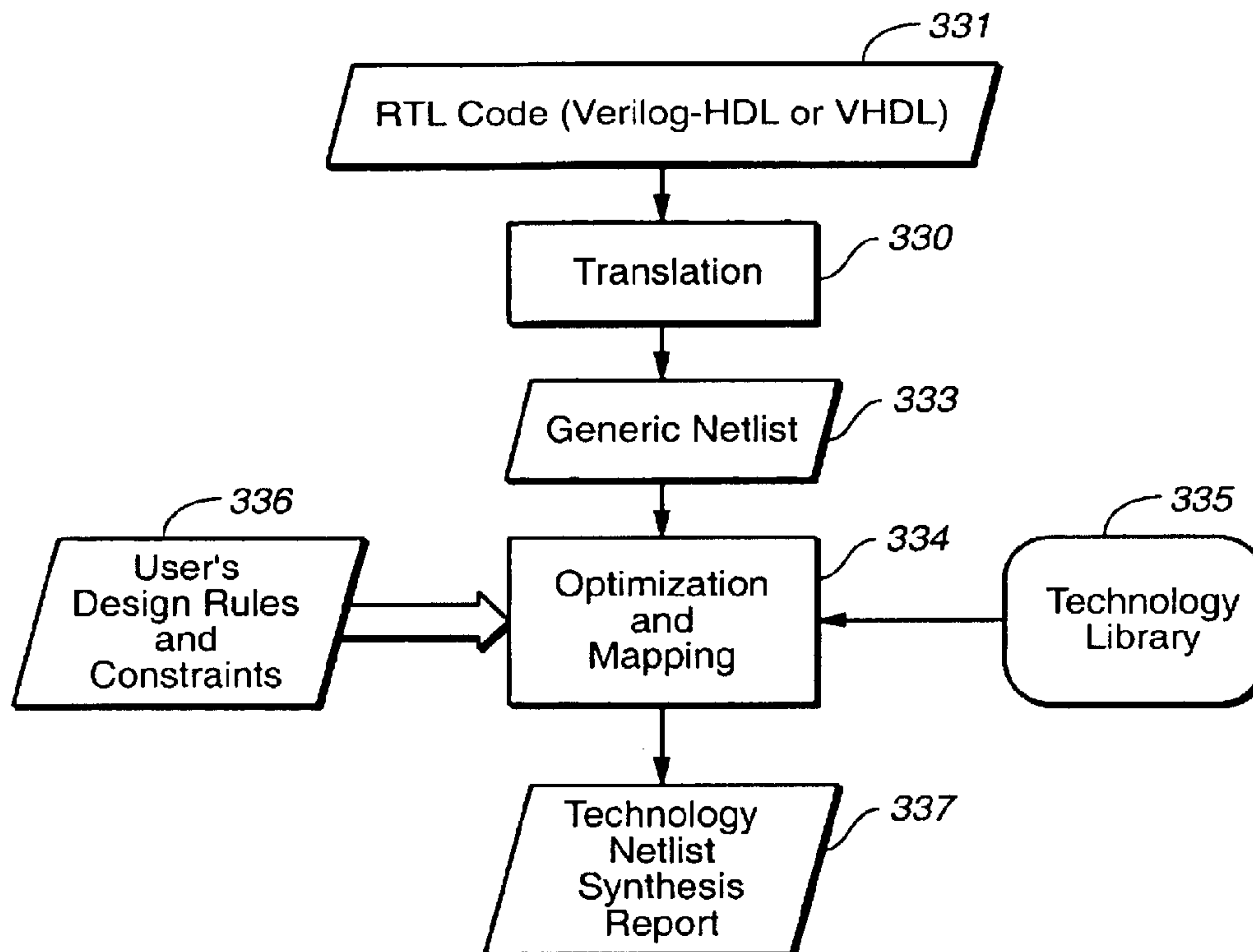
: Logic synthesis process
