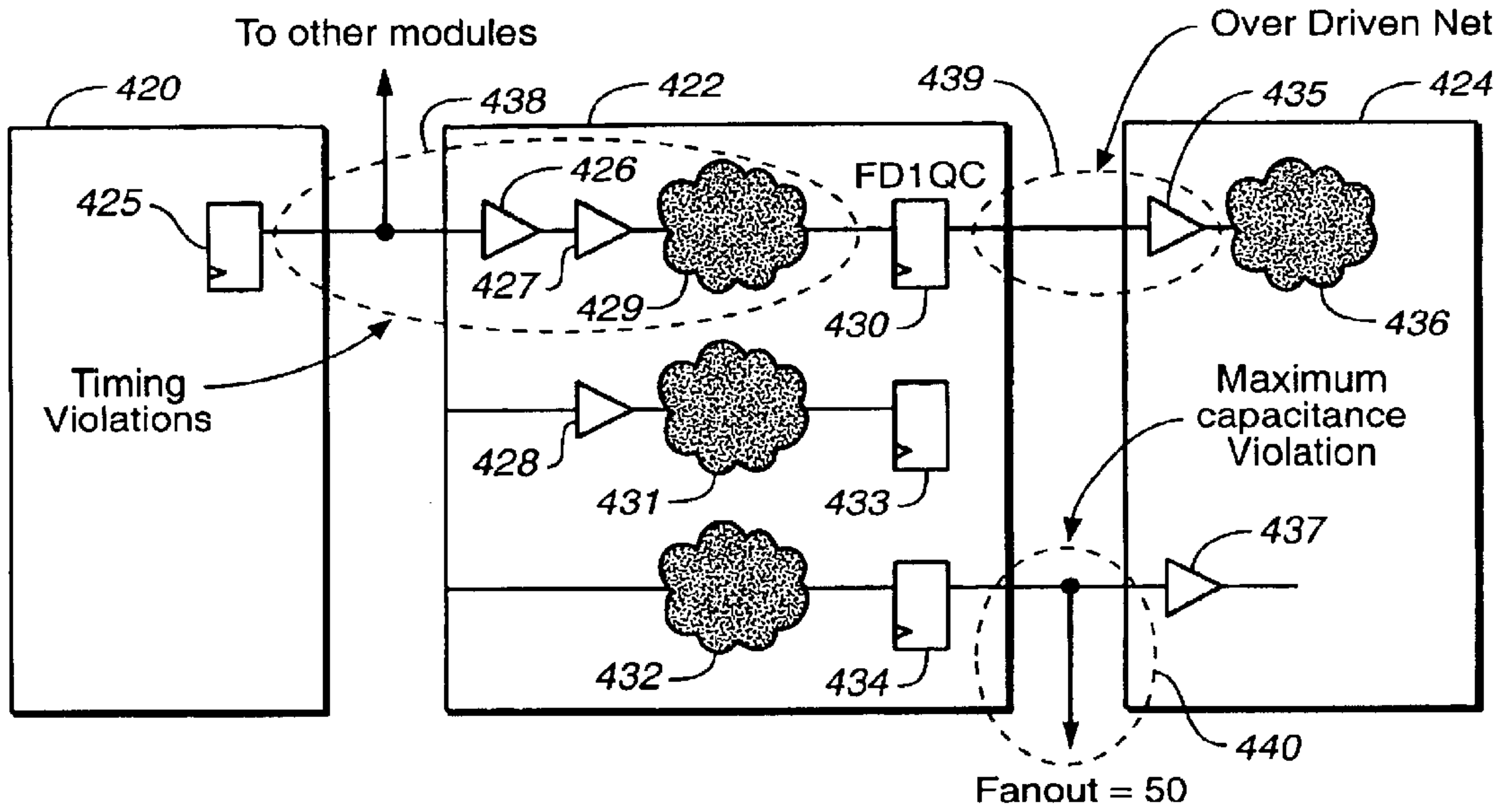
FIG. 18 : Results after initial mapping.
