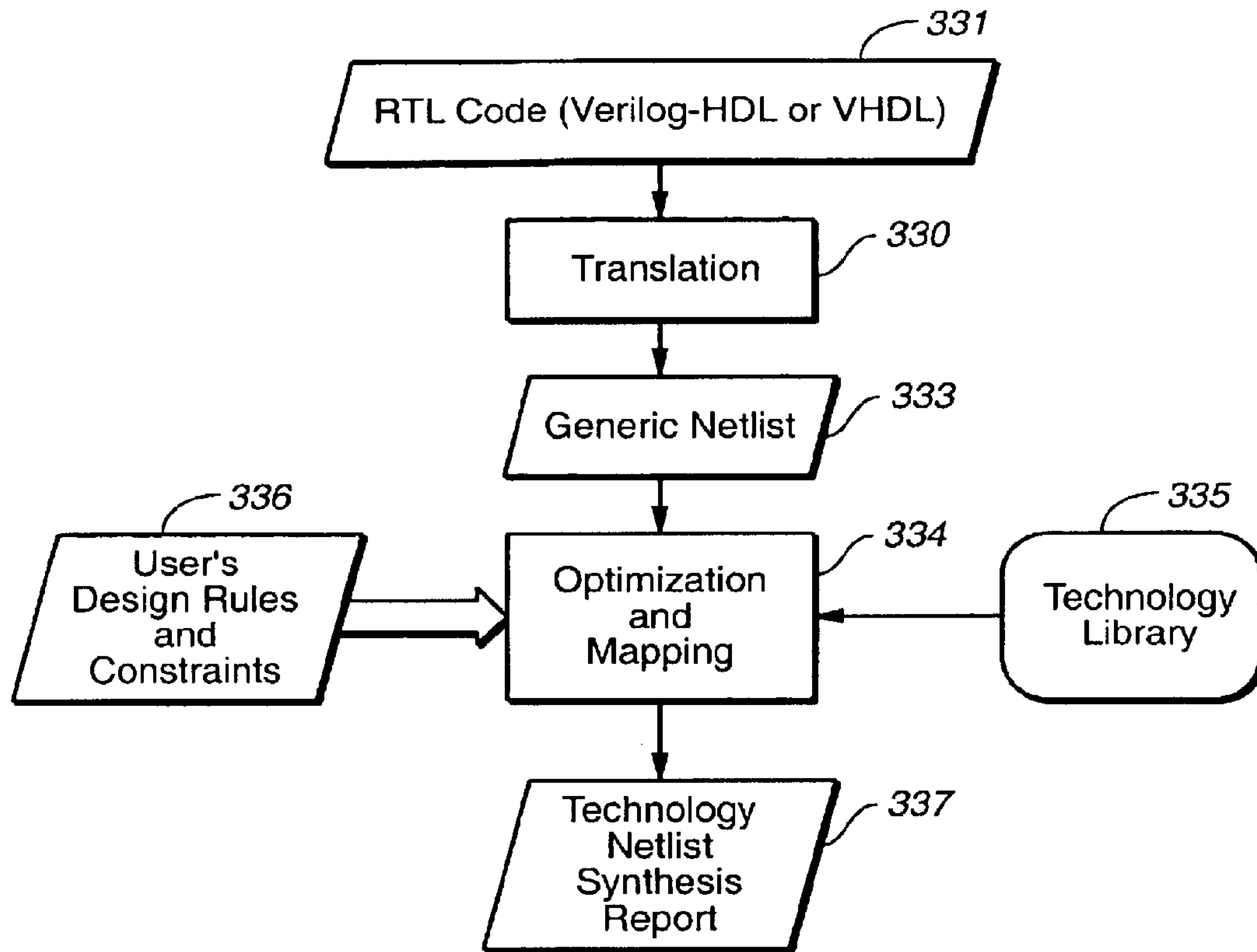
FIG. 36 : Logic synthesis process
