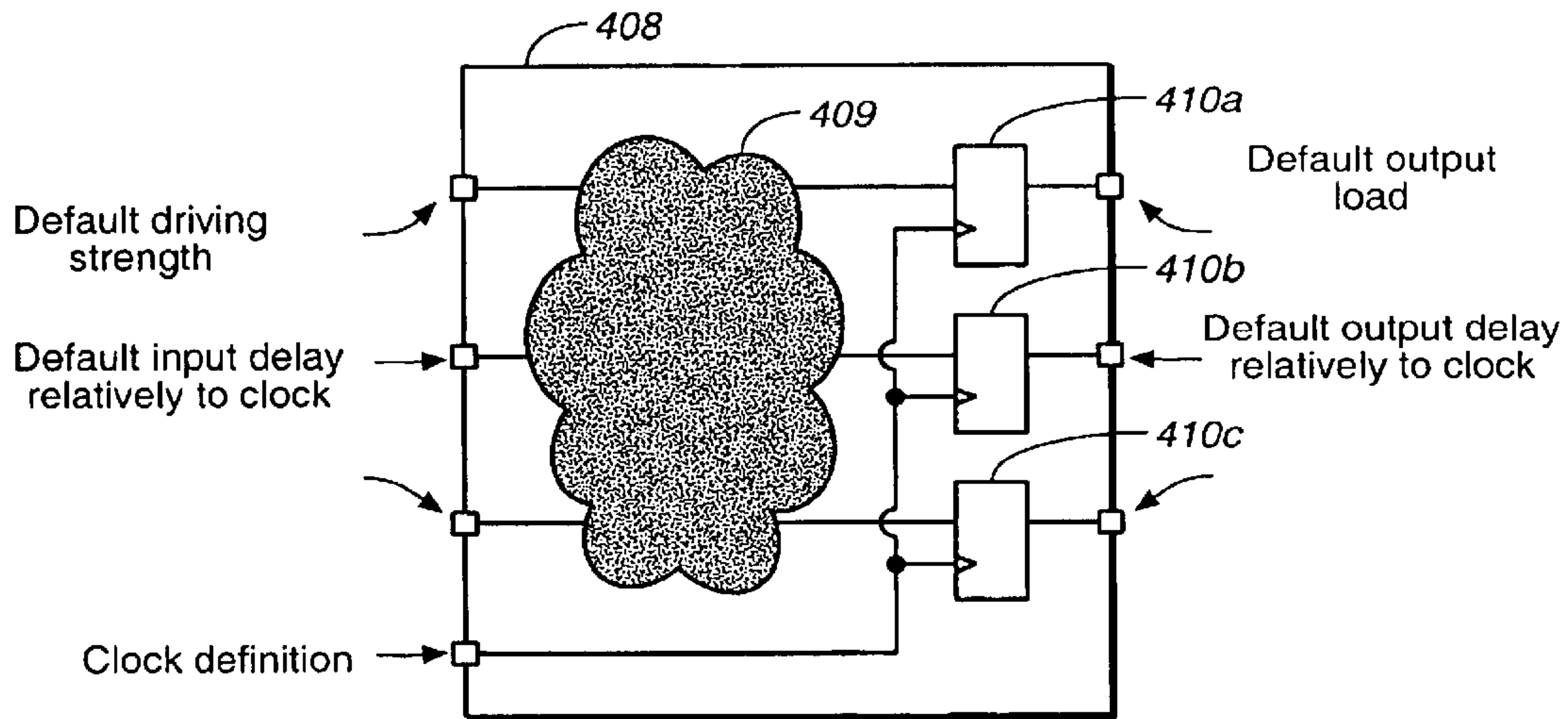
FIG. 17 :Default constraints used for initial mapping.
