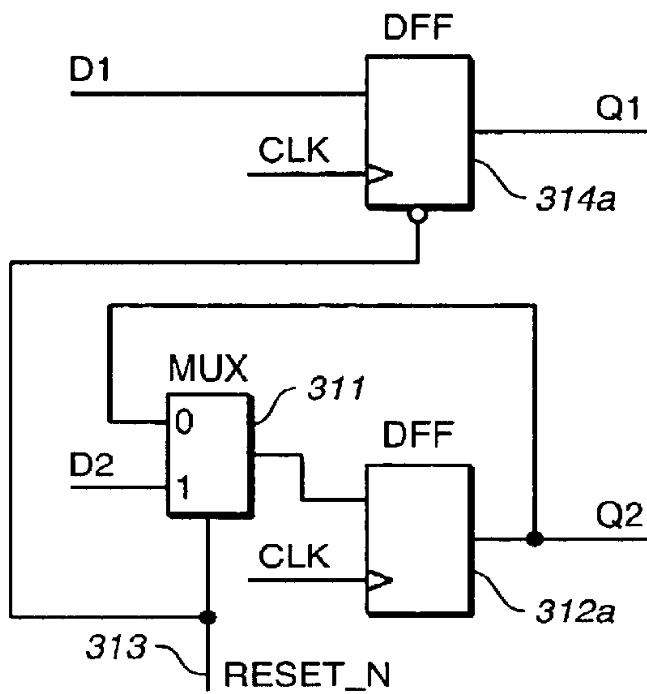
b. Implementation created by Synopsys Design Compiler
