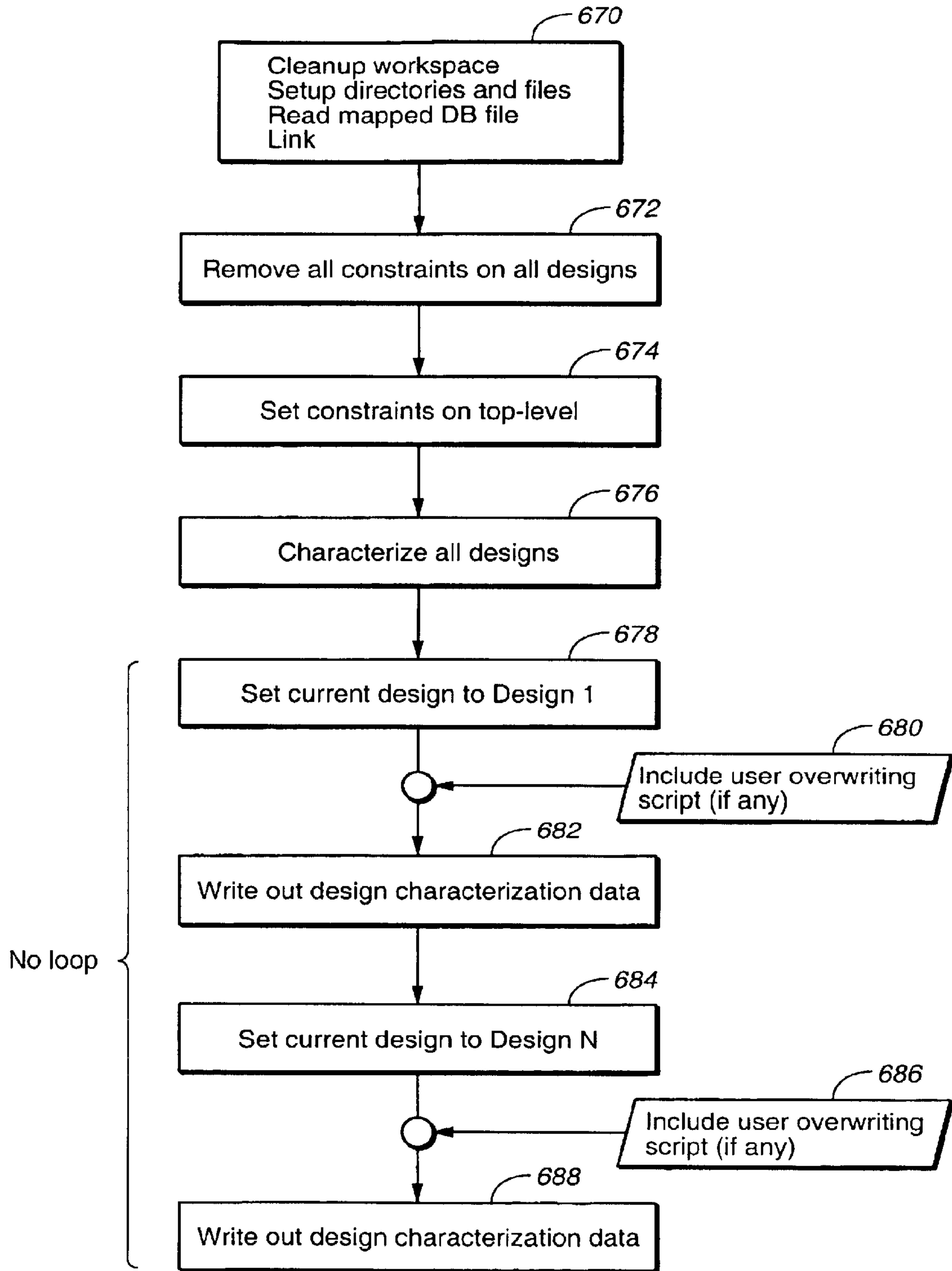
FIG. 30 : Structure of characterization script
