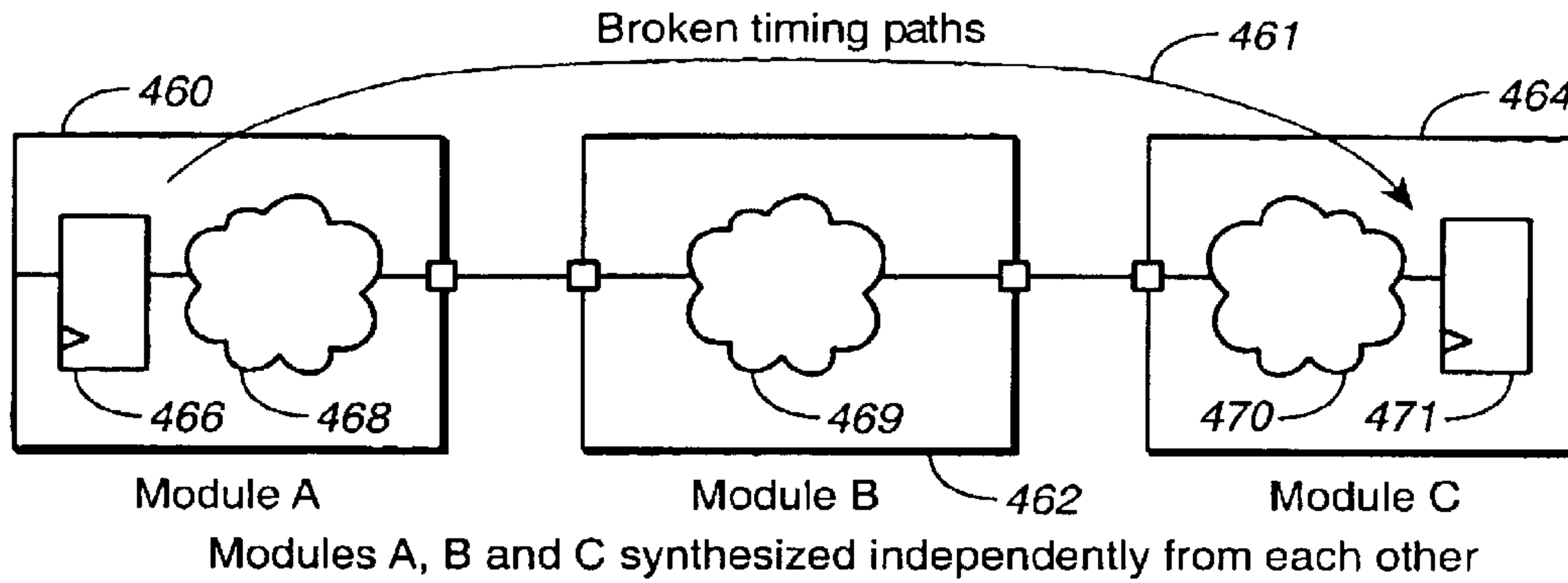
FIG. 20A : Broken timing paths
