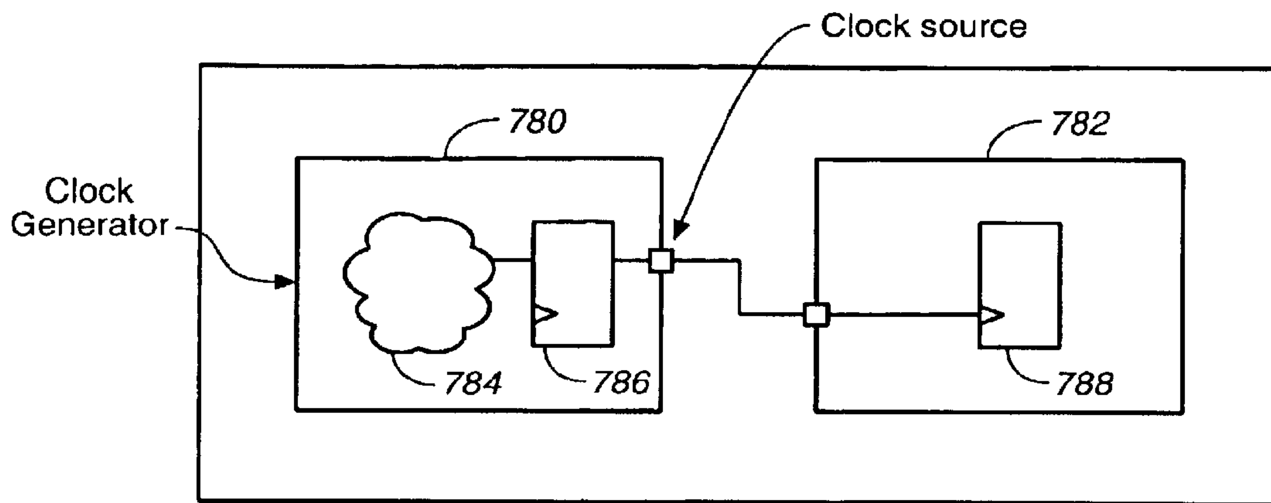
(a) Generic netlist
