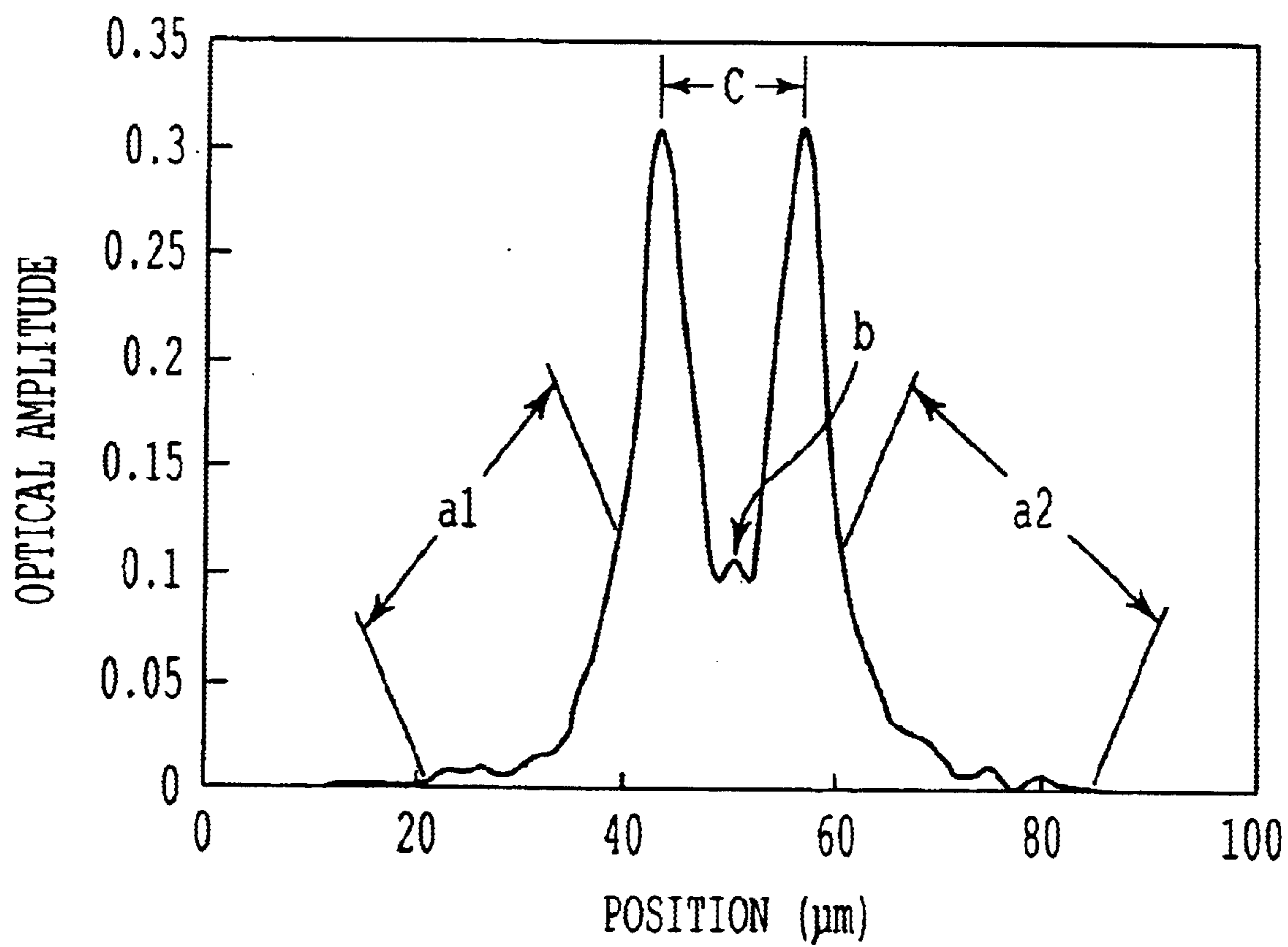
FIG. 25 (BACKGROUND ART)
