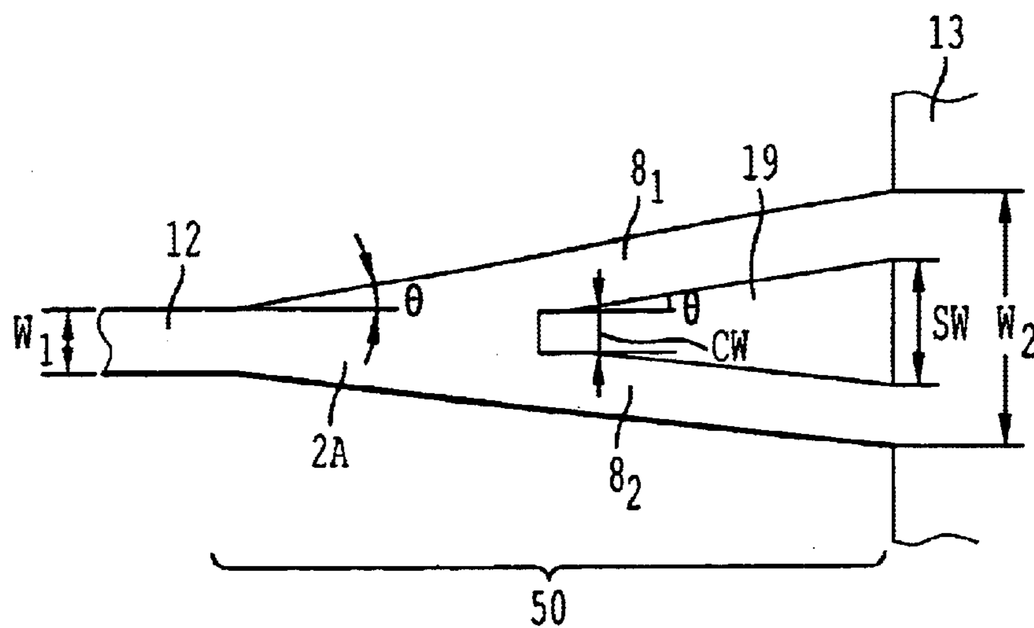
FIG. 21 (BACKGROUND ART)
