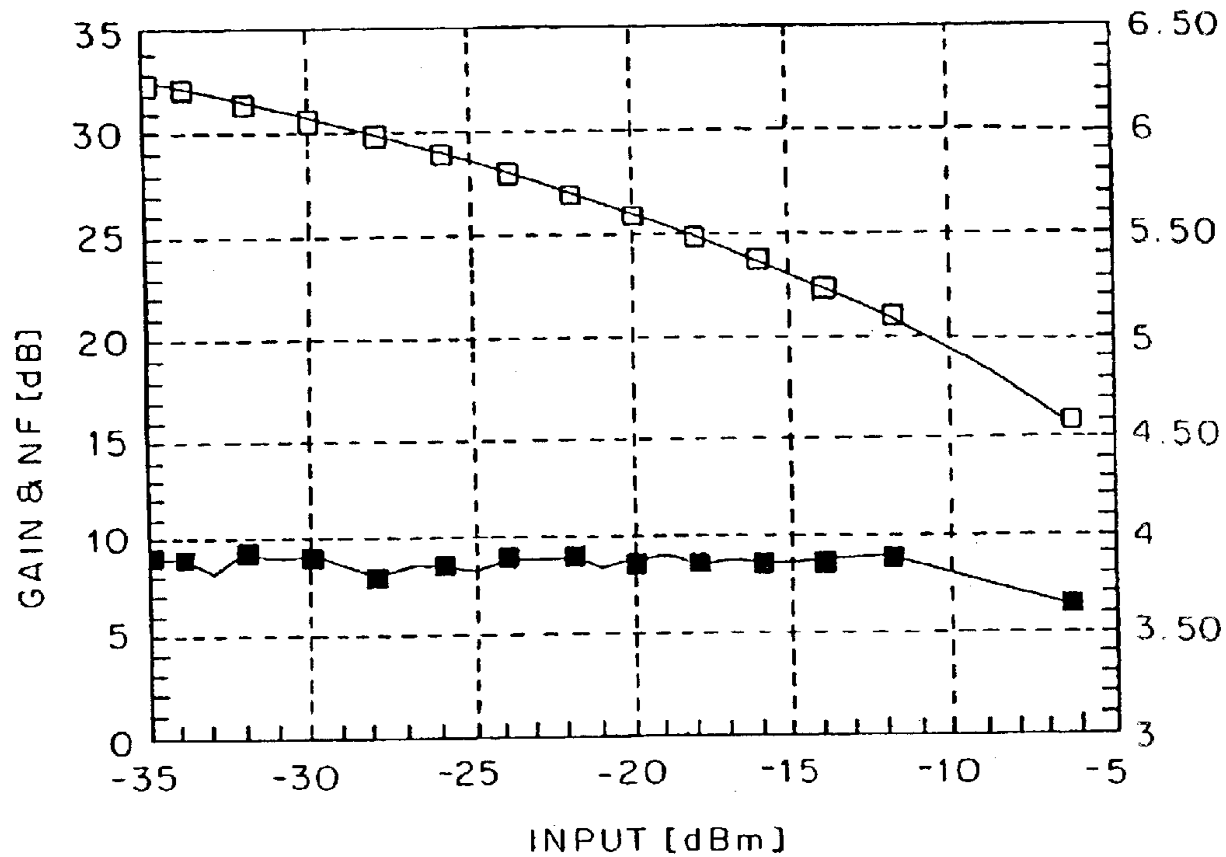
INPUT VS GAIN & NF TEST
