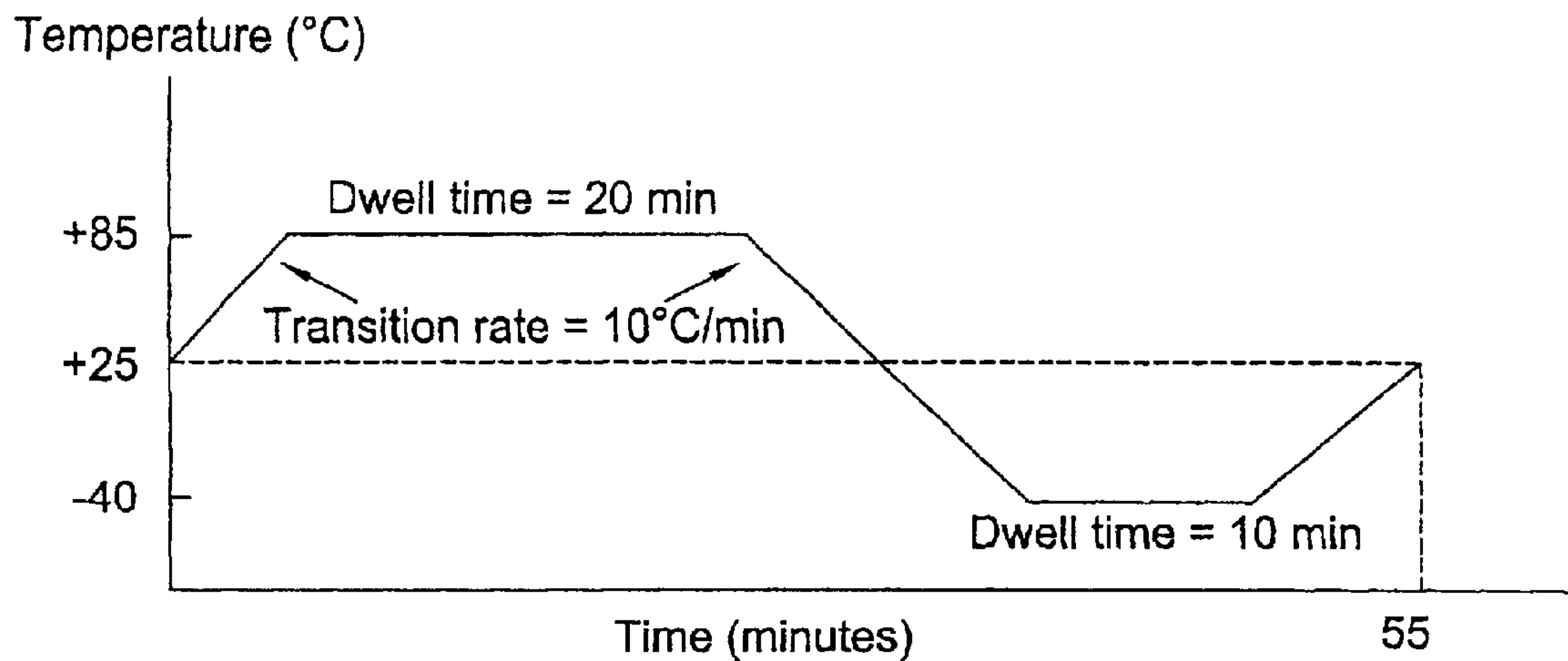
PTMCL temperature profile
