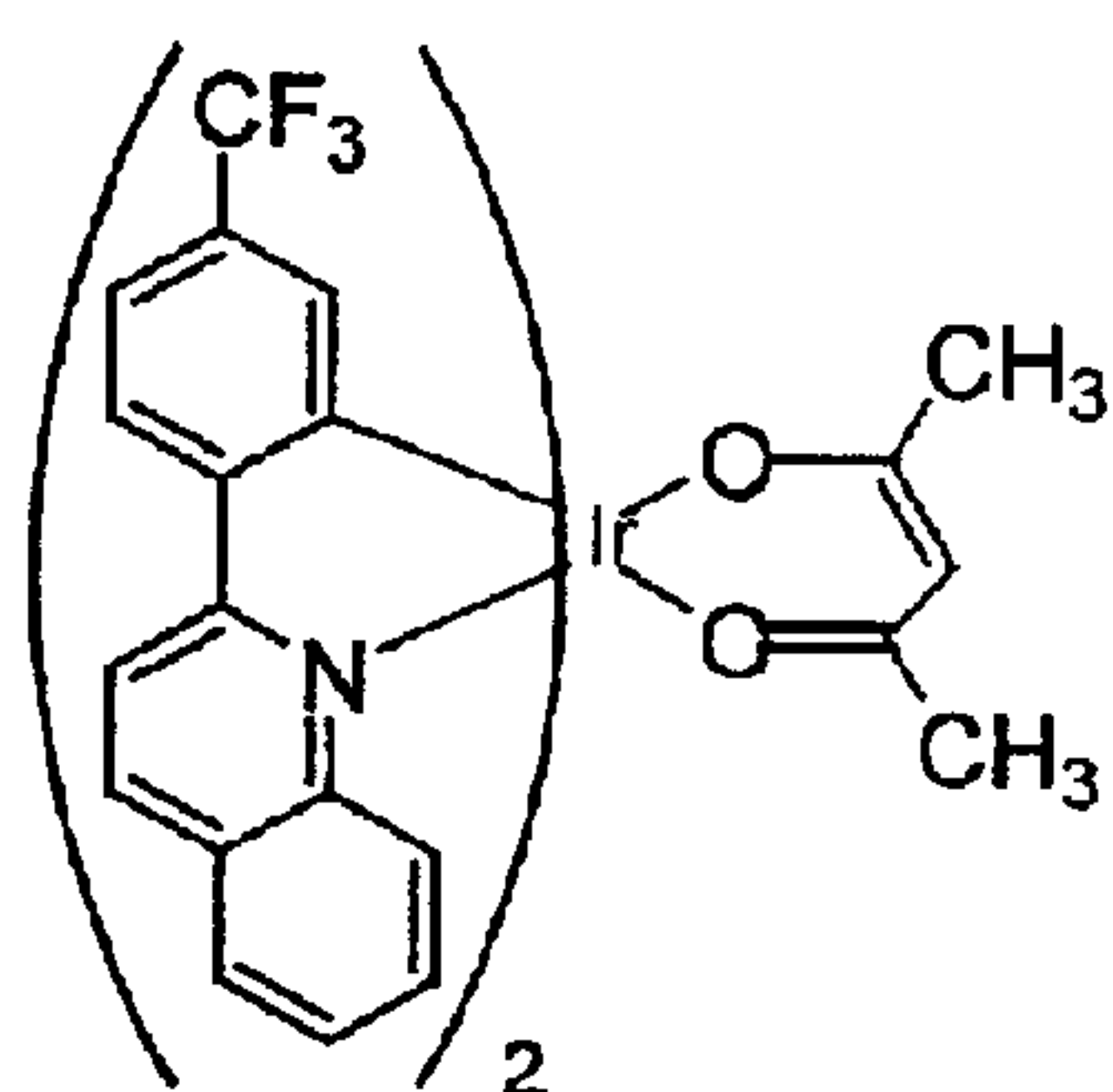
Compound 9
