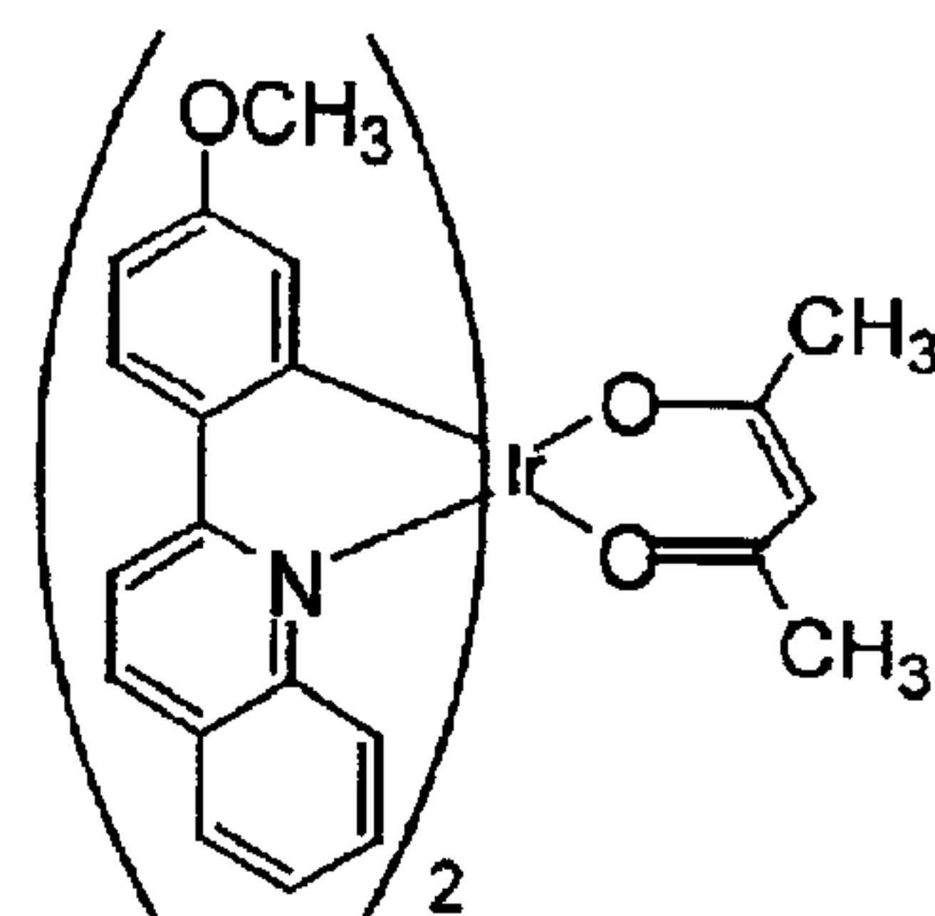
Compound 6
