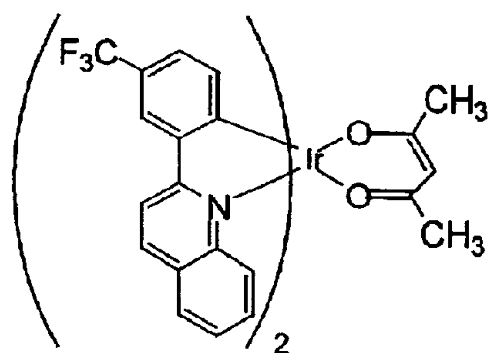
Compound 8
