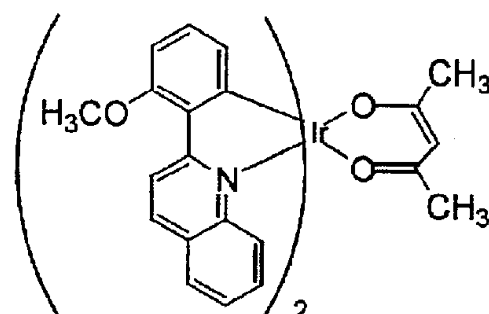
Compound 4
