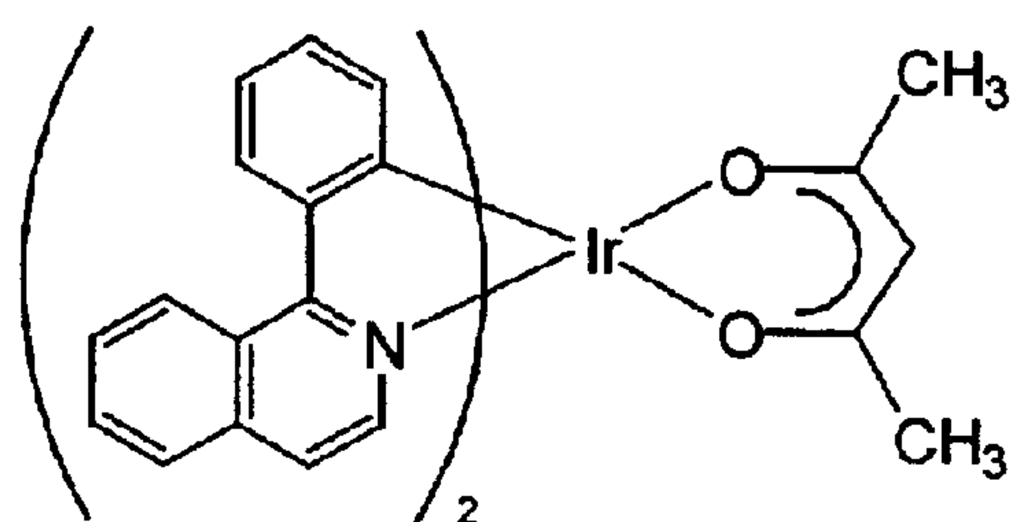
Compound 13
