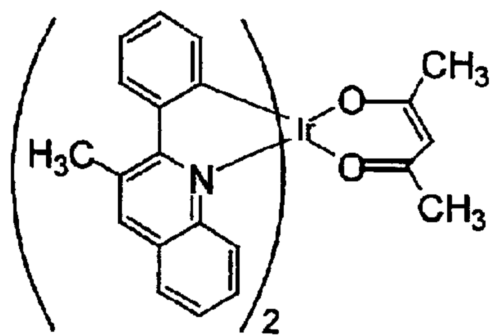
Compound 12
