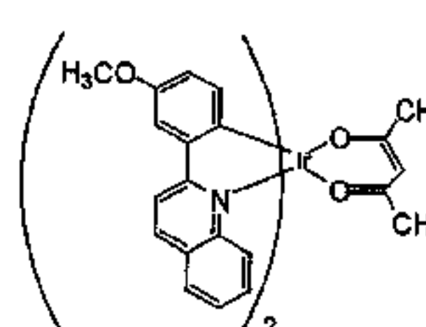
Compound 5
