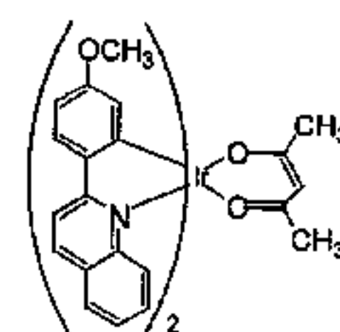
Compound 6
