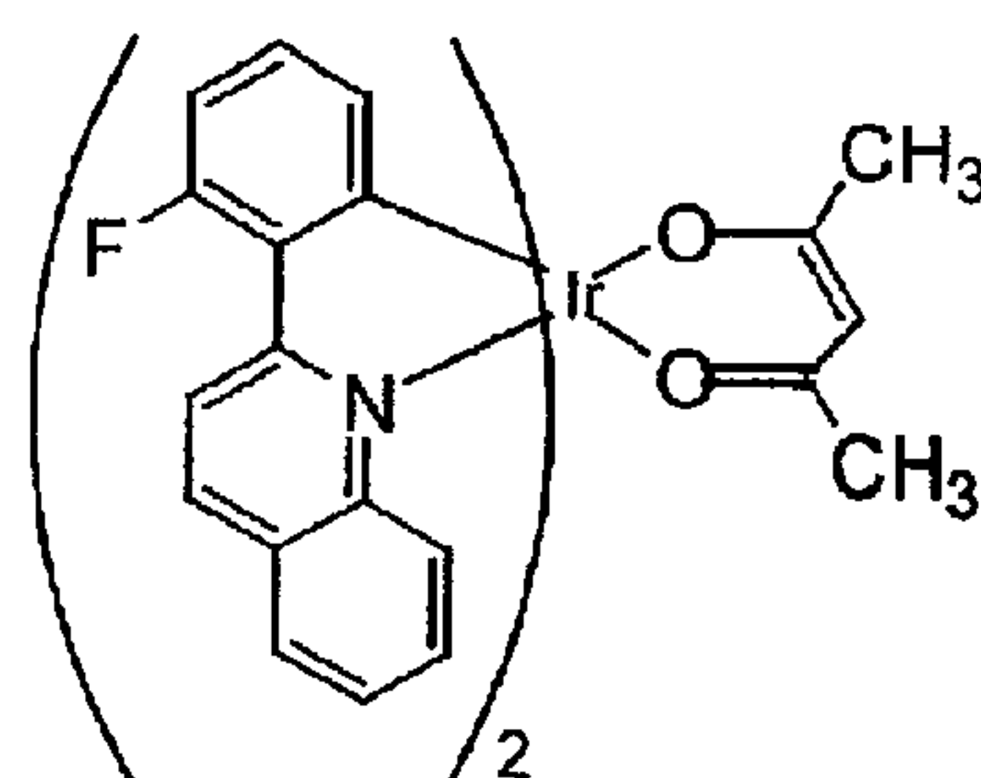
Compound 2
