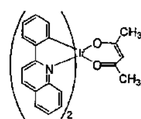
Compound 1
