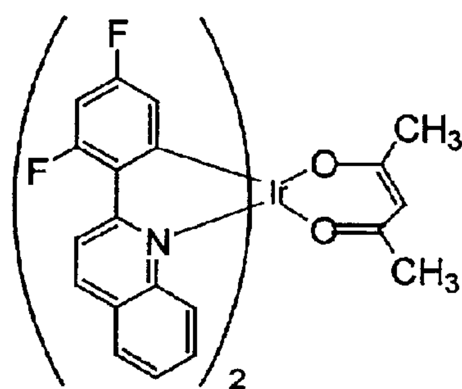
Compound 10
