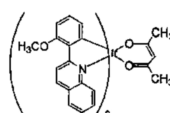
Compound 4
