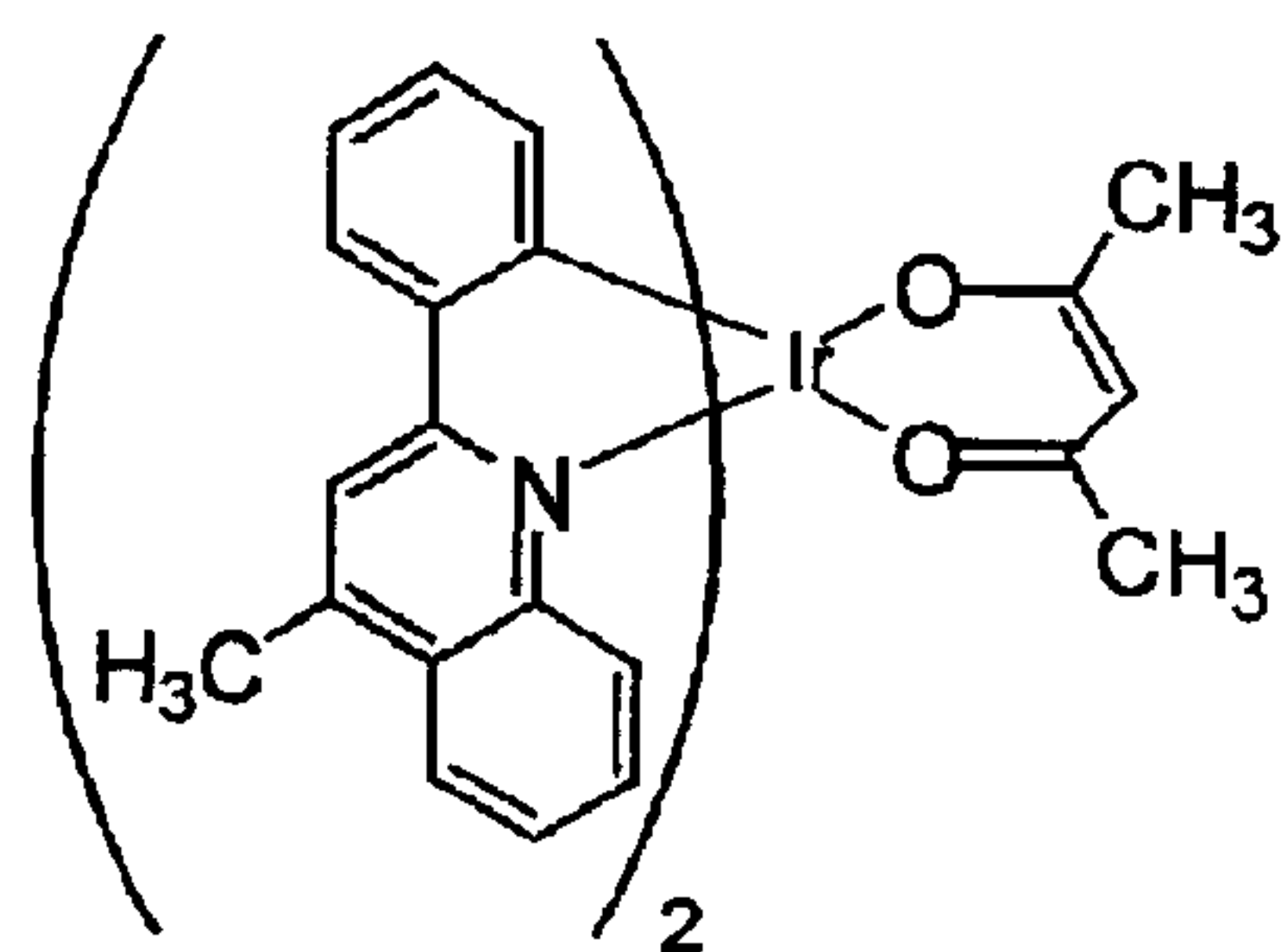
Compound 11
