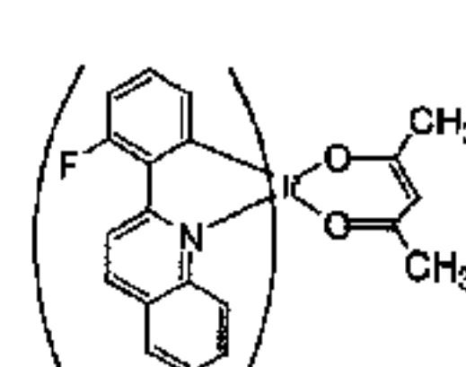
Compound 2
