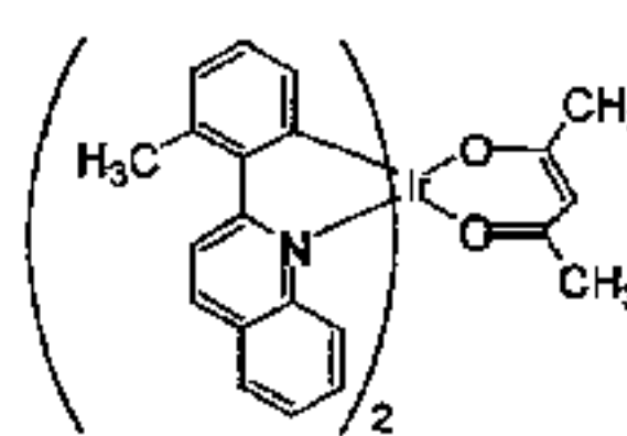
Compound 3
