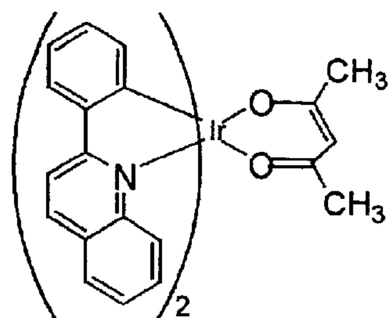
Compound 1
