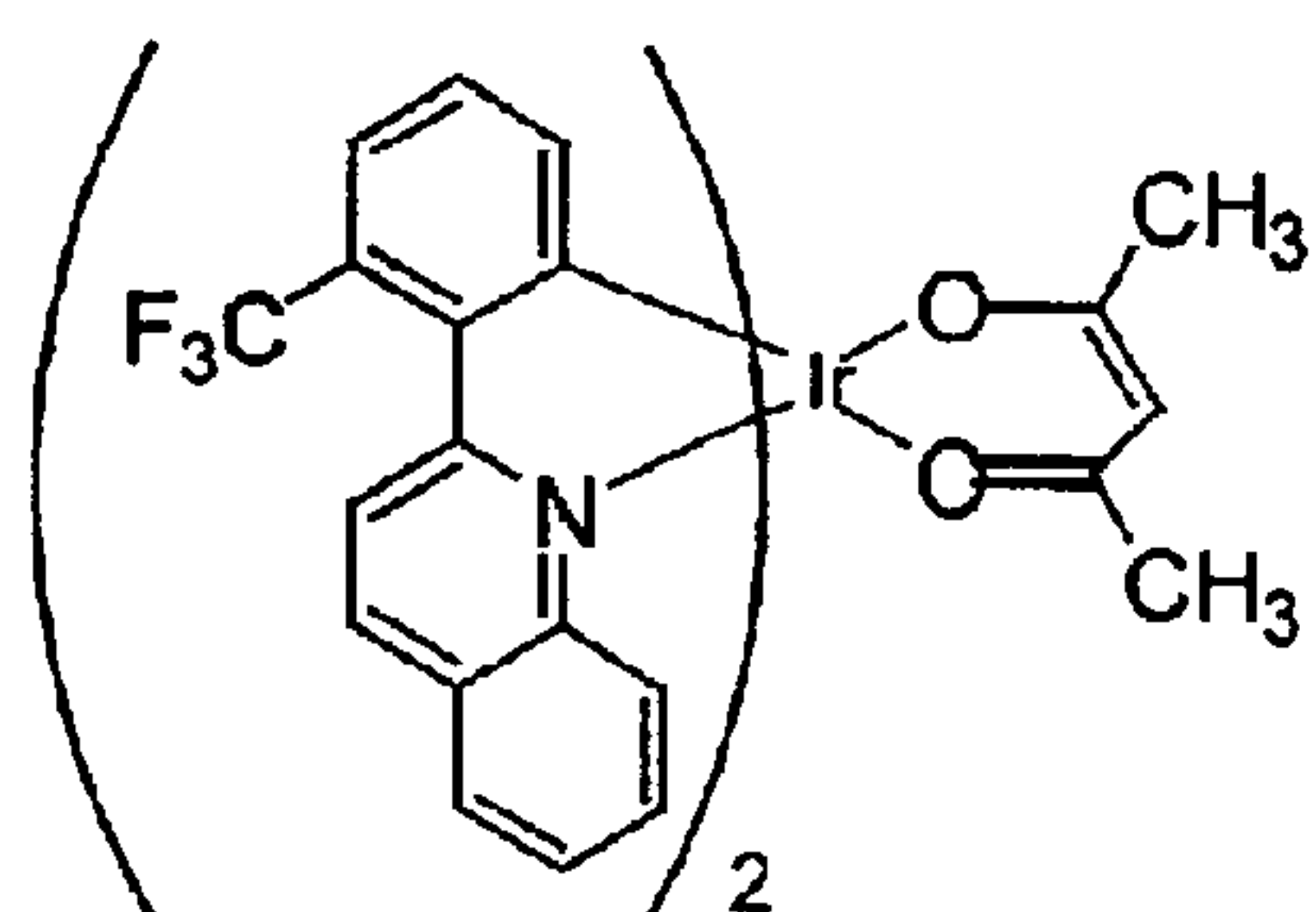
Compound 7
