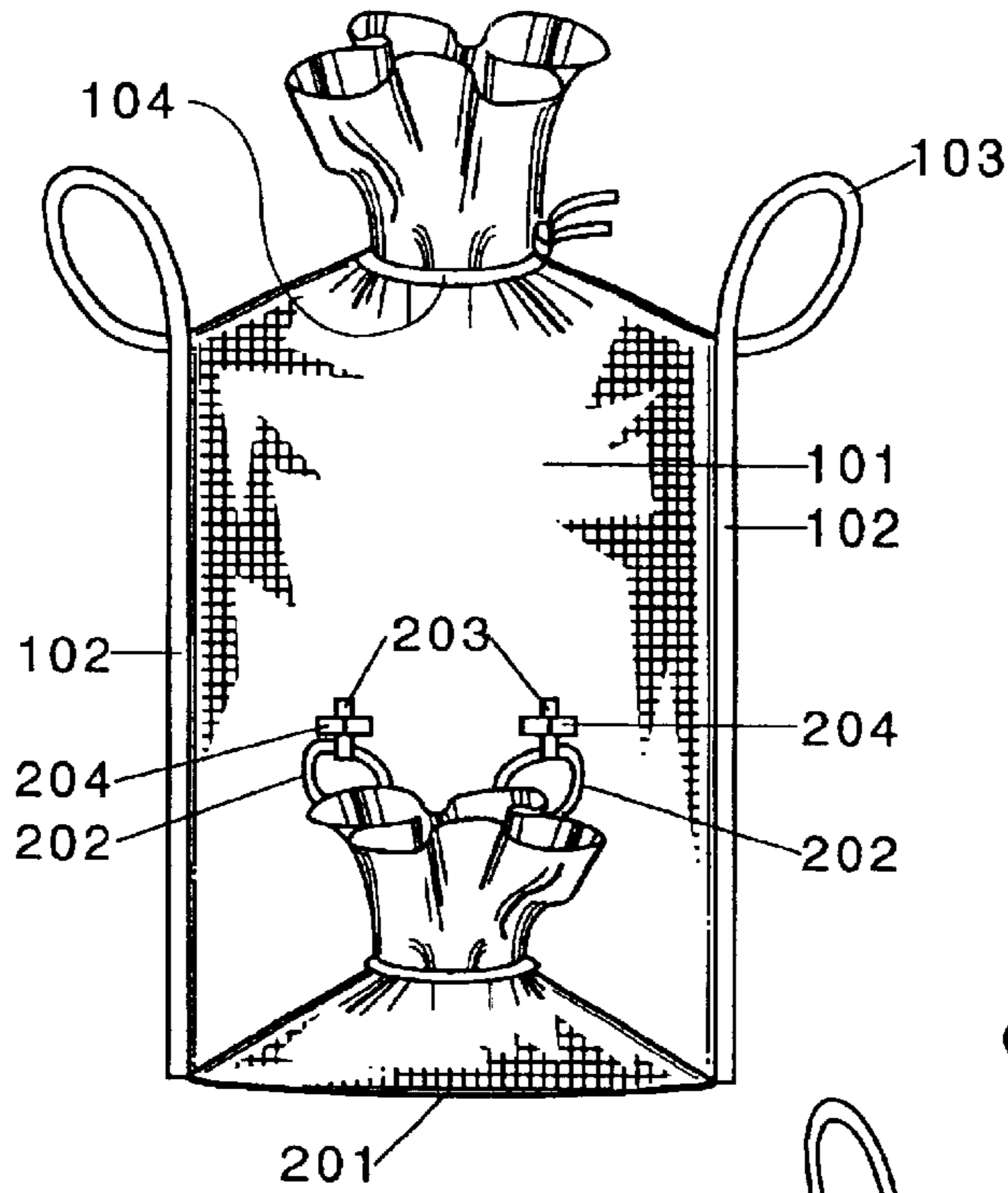
Fig. 1 (PRIOR ART)
