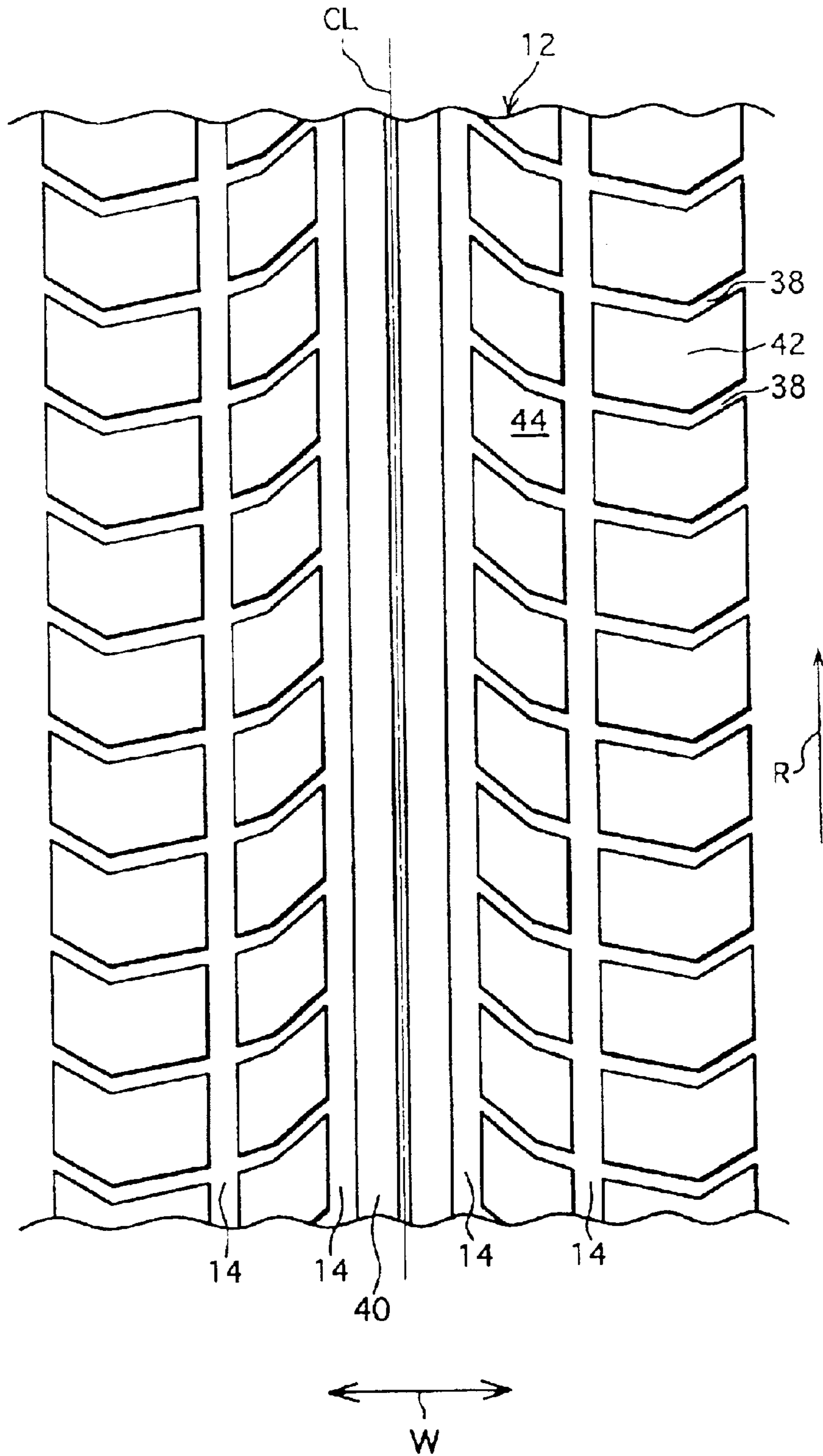
FIG. 8 PRIOR ART
