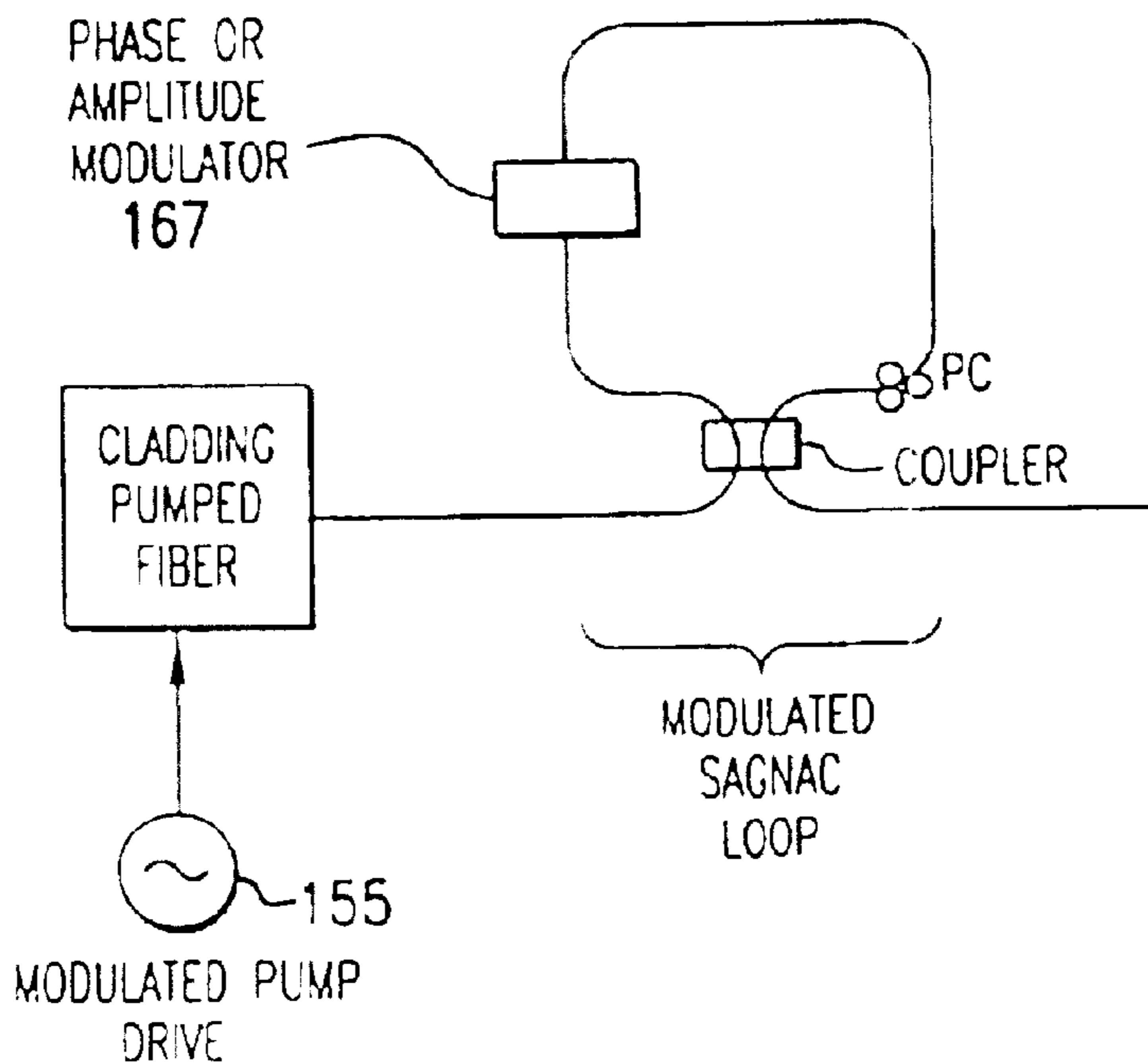
FIG.14c PRIOR ART
