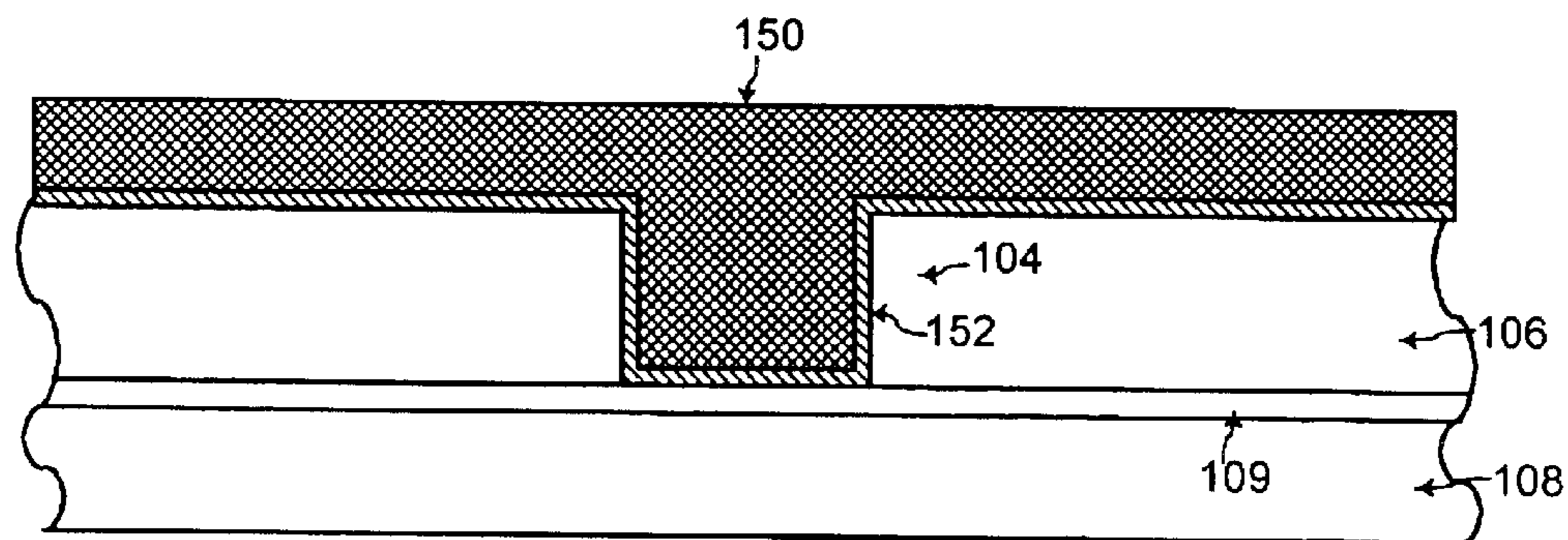
FIG. 3 (Prior Art)
