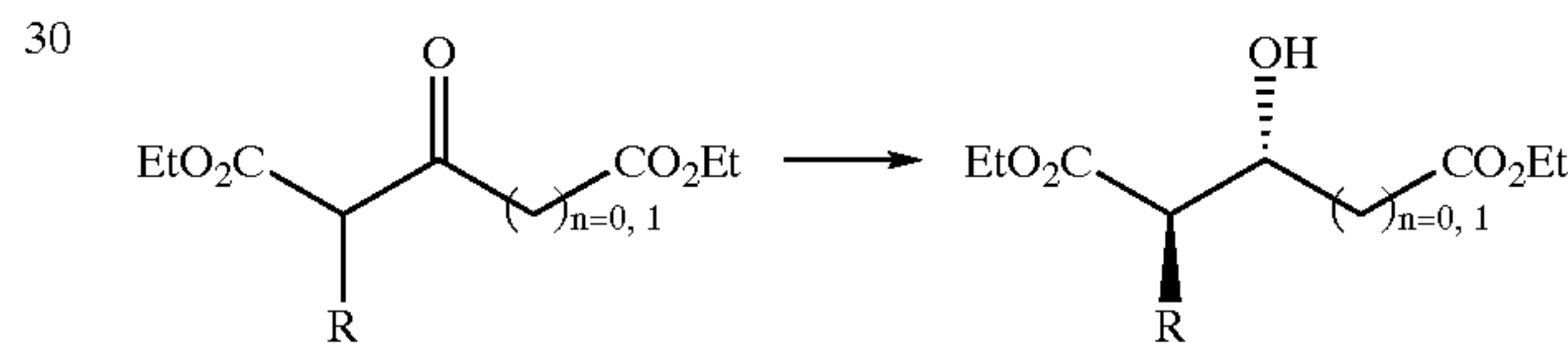
Figure 5: Diastereoselective reduction of \beta -ketodiesters
