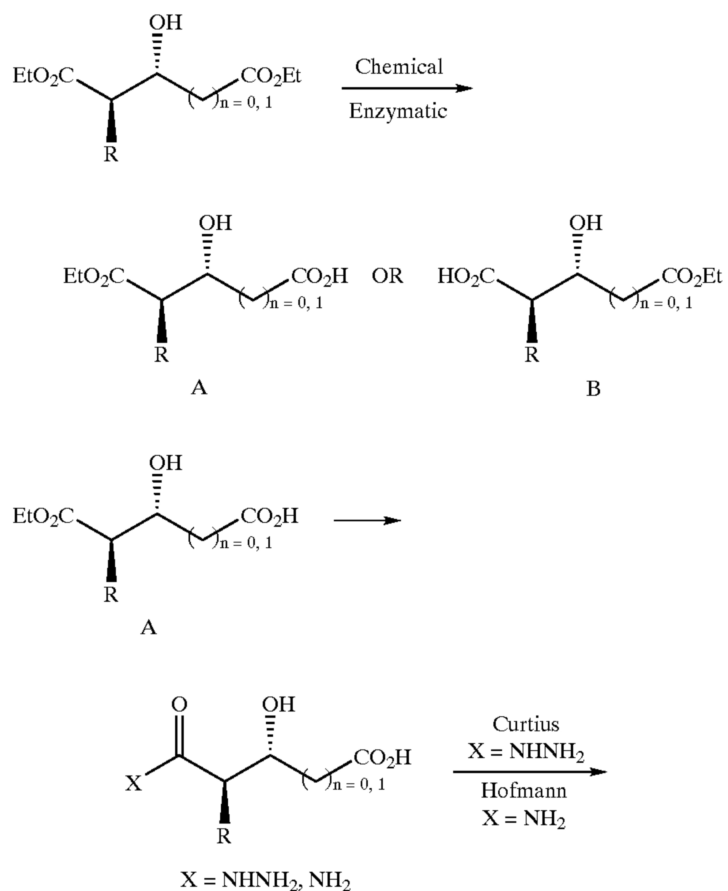
FIG. 6. Regioselective chemical or enzymatic hydrolysis followed by rearrangement gives the final product.
