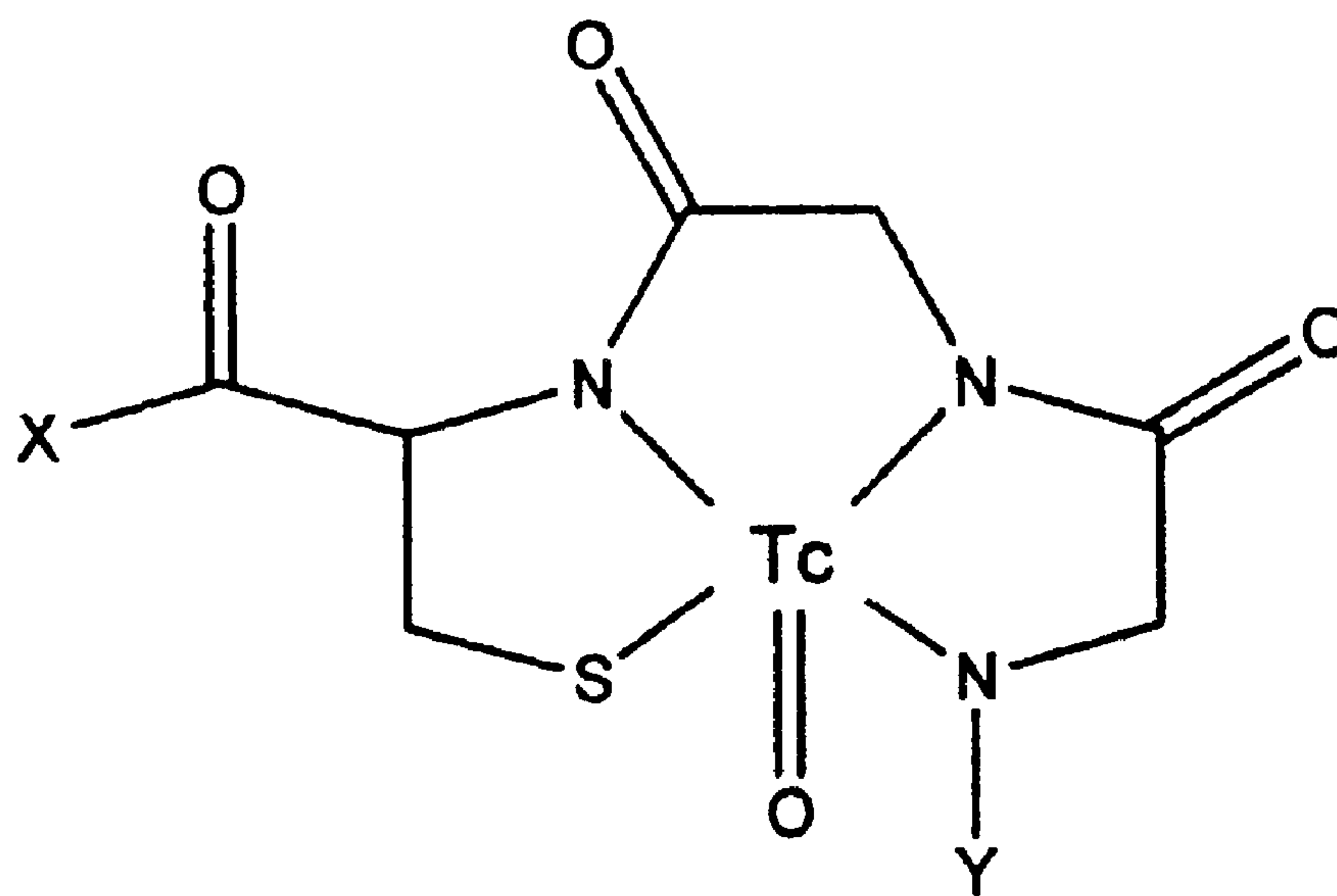
(NH 2 ) Gly-Gly-Cys (CO 2 H)
