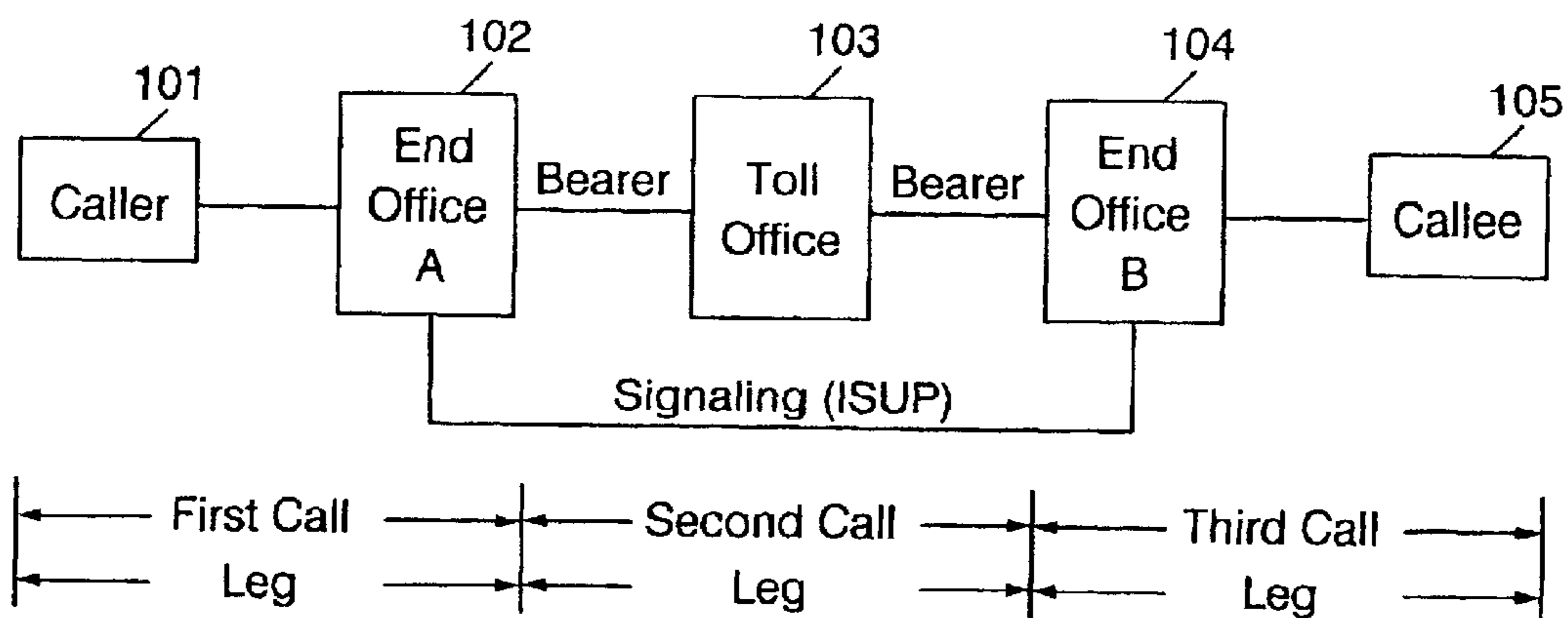
FIG. 1 PRIOR ART
