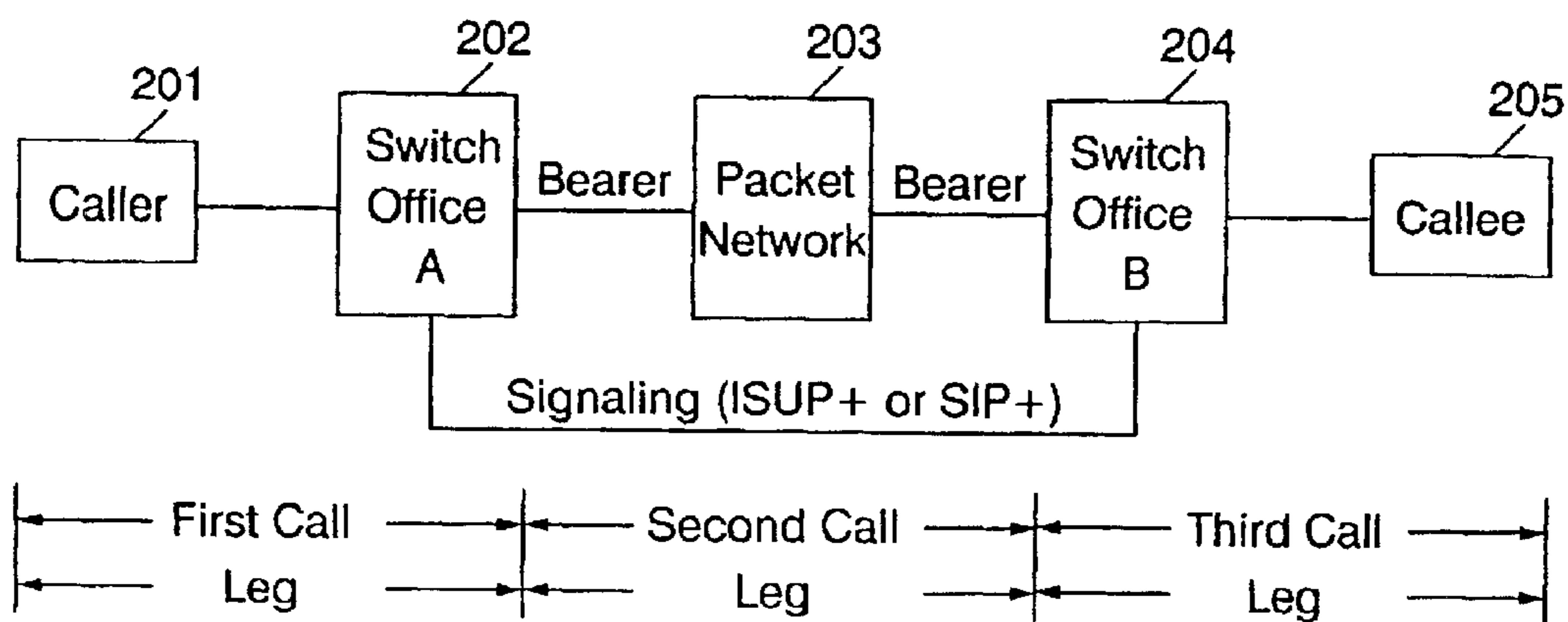
FIG. 2 PRIOR ART
