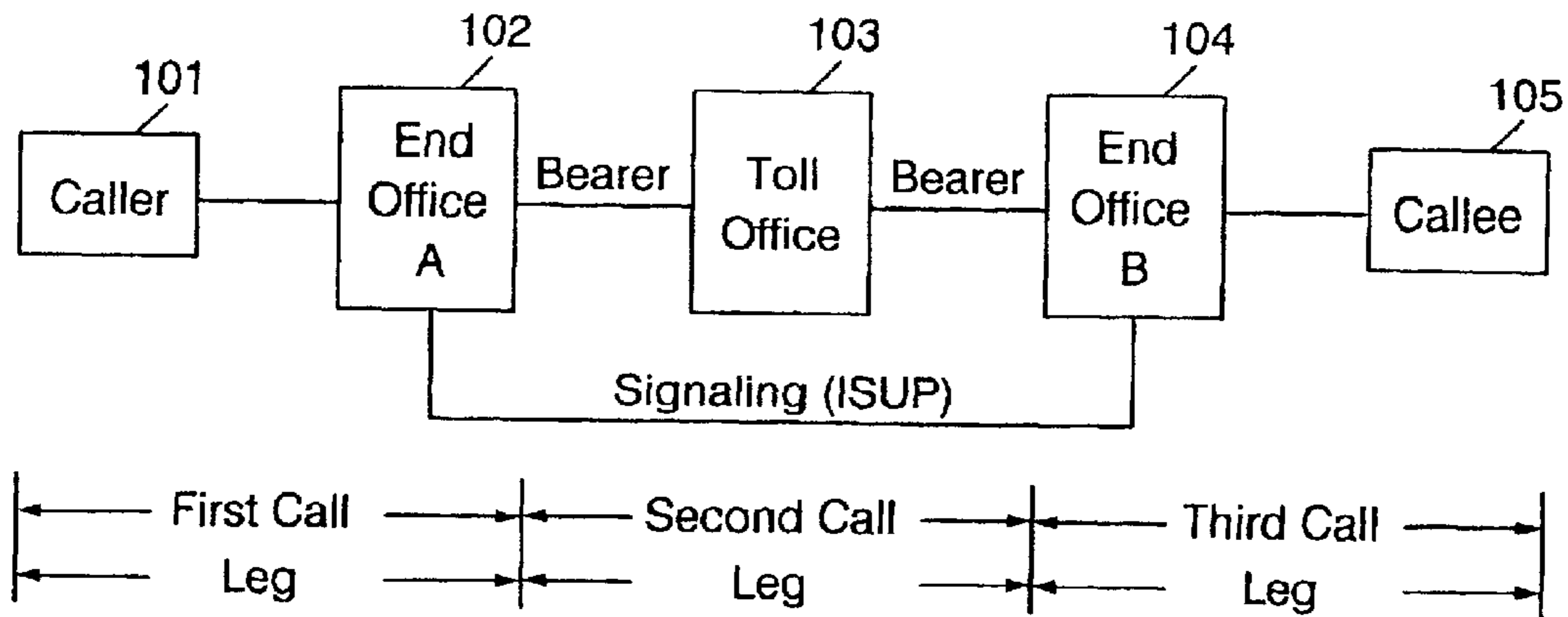
FIG. 1 PRIOR ART
