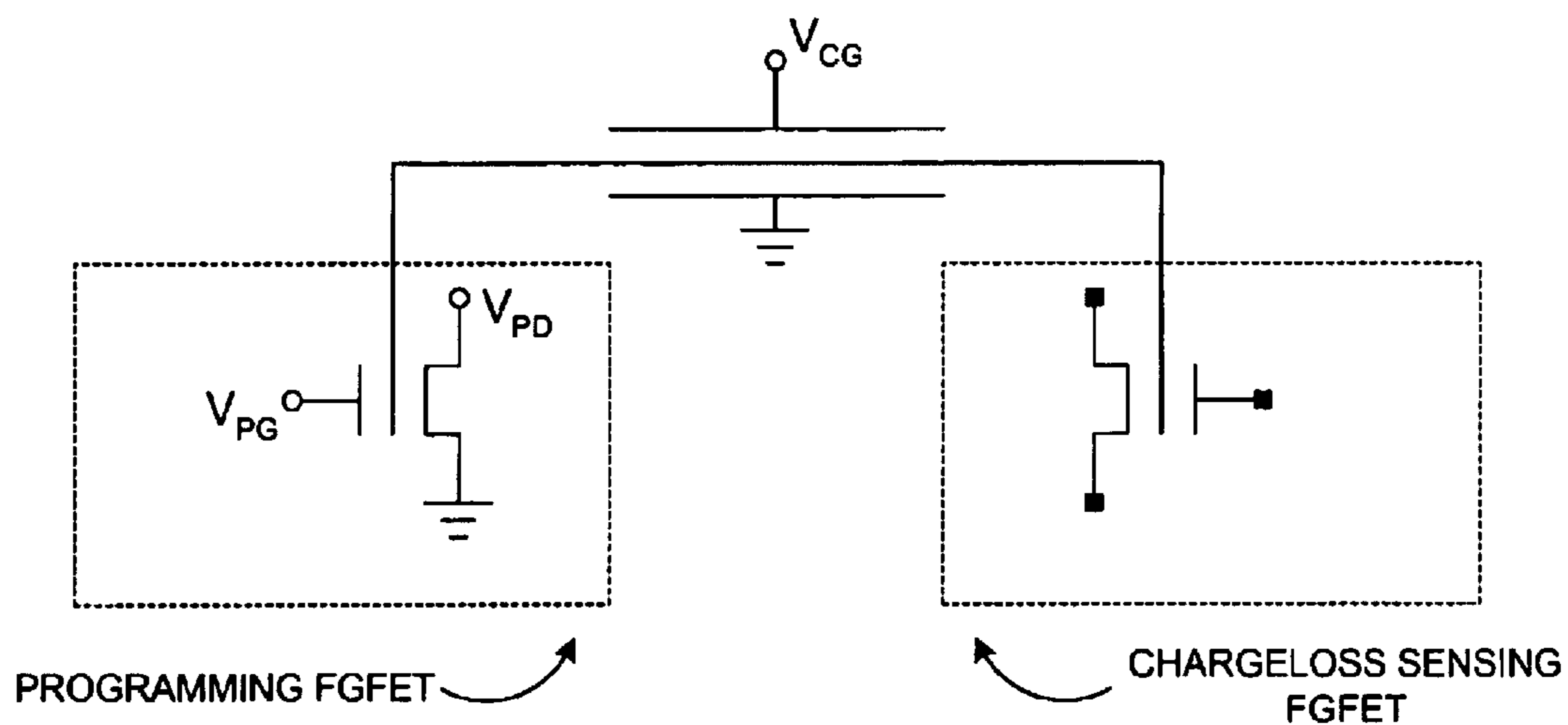
VOLTAGES DURING PROGRAMMING OPERATION
