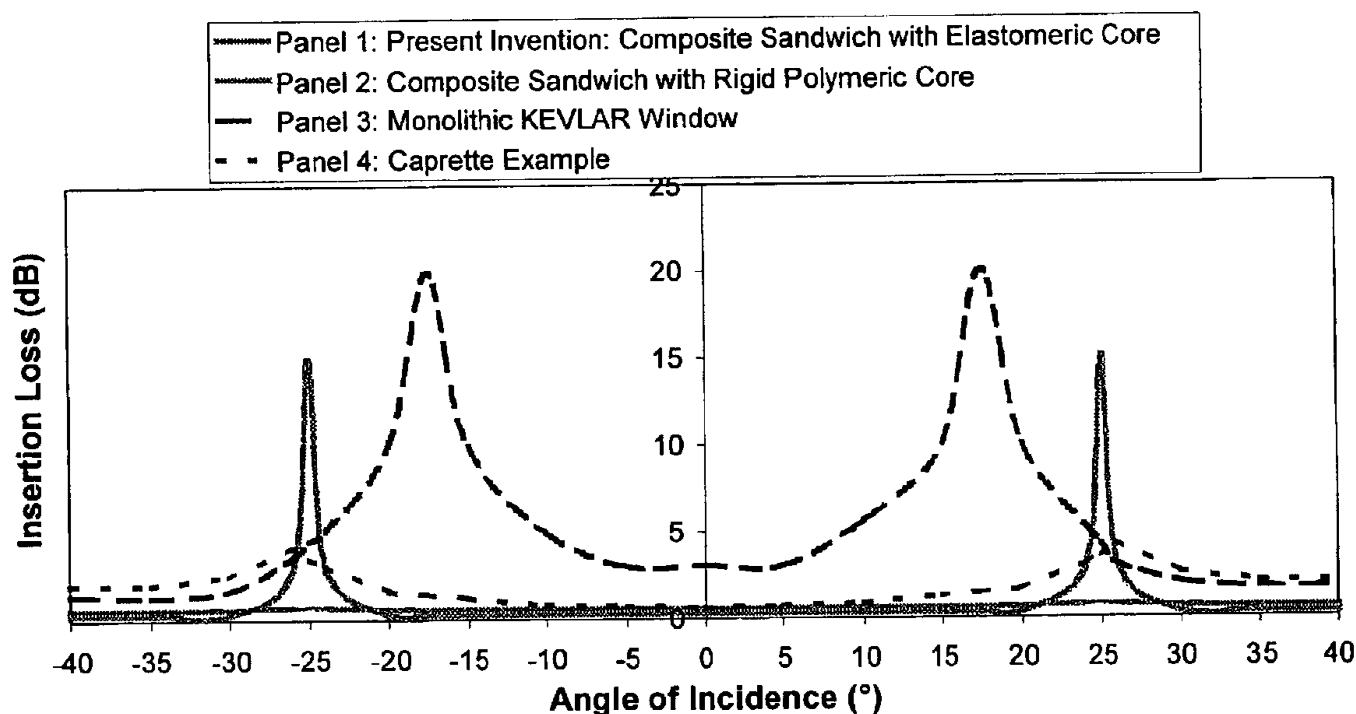
Typical Insertion Loss versus Angle of
