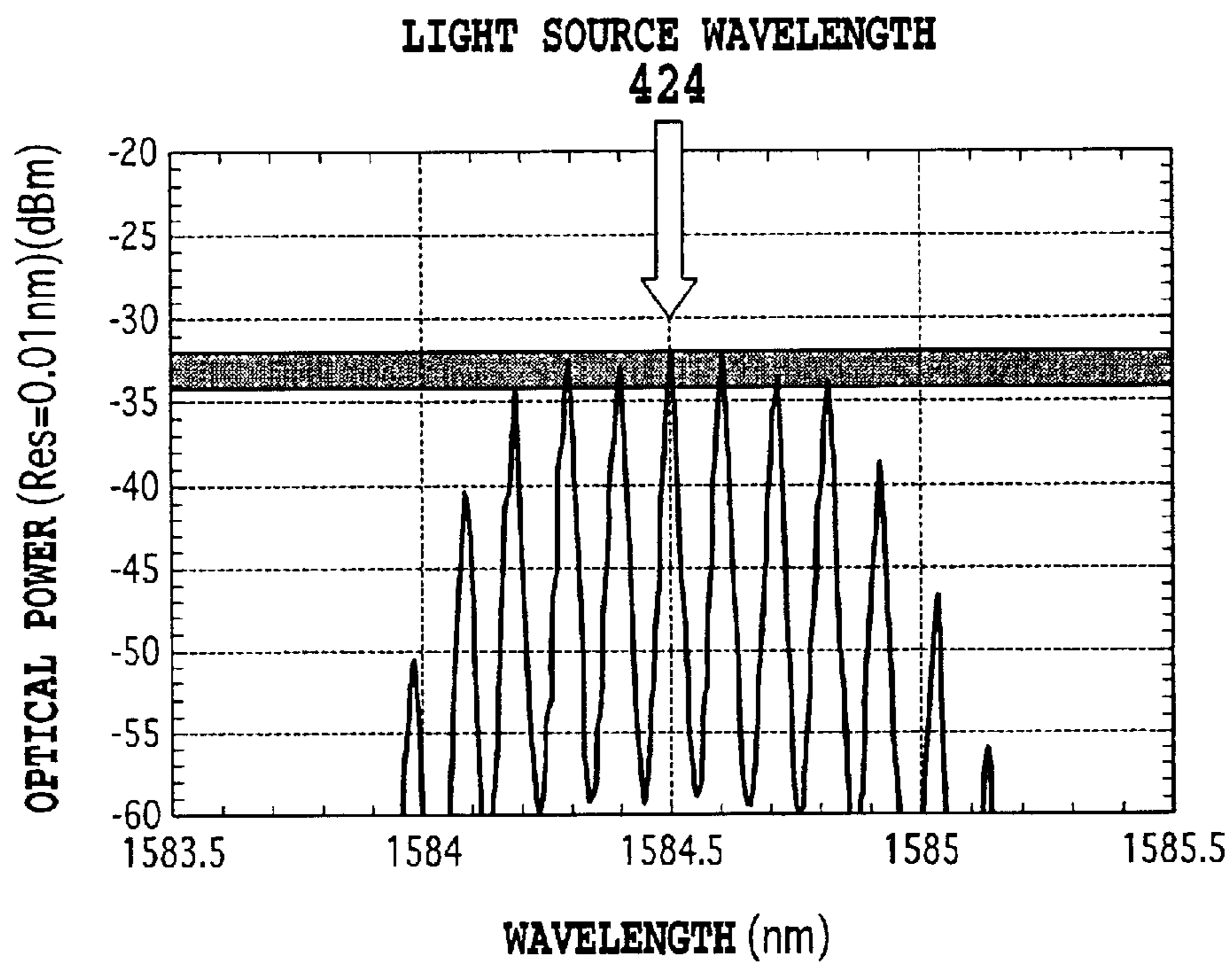
EVEN-NUMBER-TH LIGHT SOURCE WAVELENGTH AND SIDE MODES
