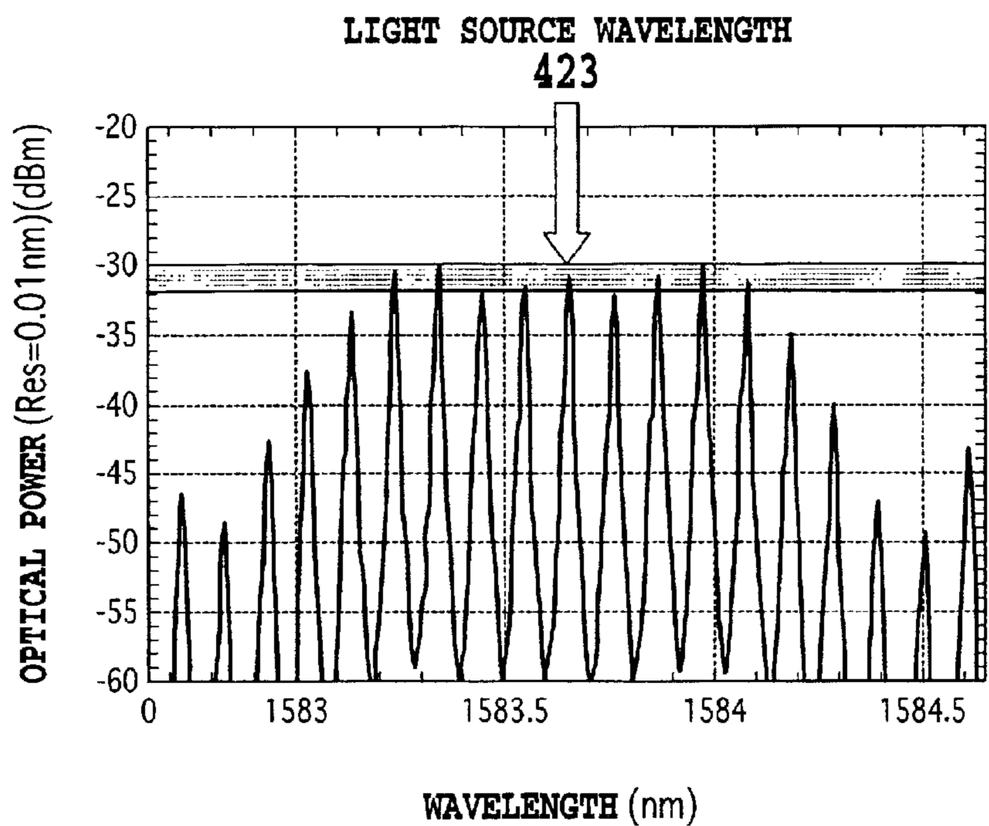
ODD-NUMBER-TH LIGHT SOURCE WAVELENGTH AND SIDE MODES
