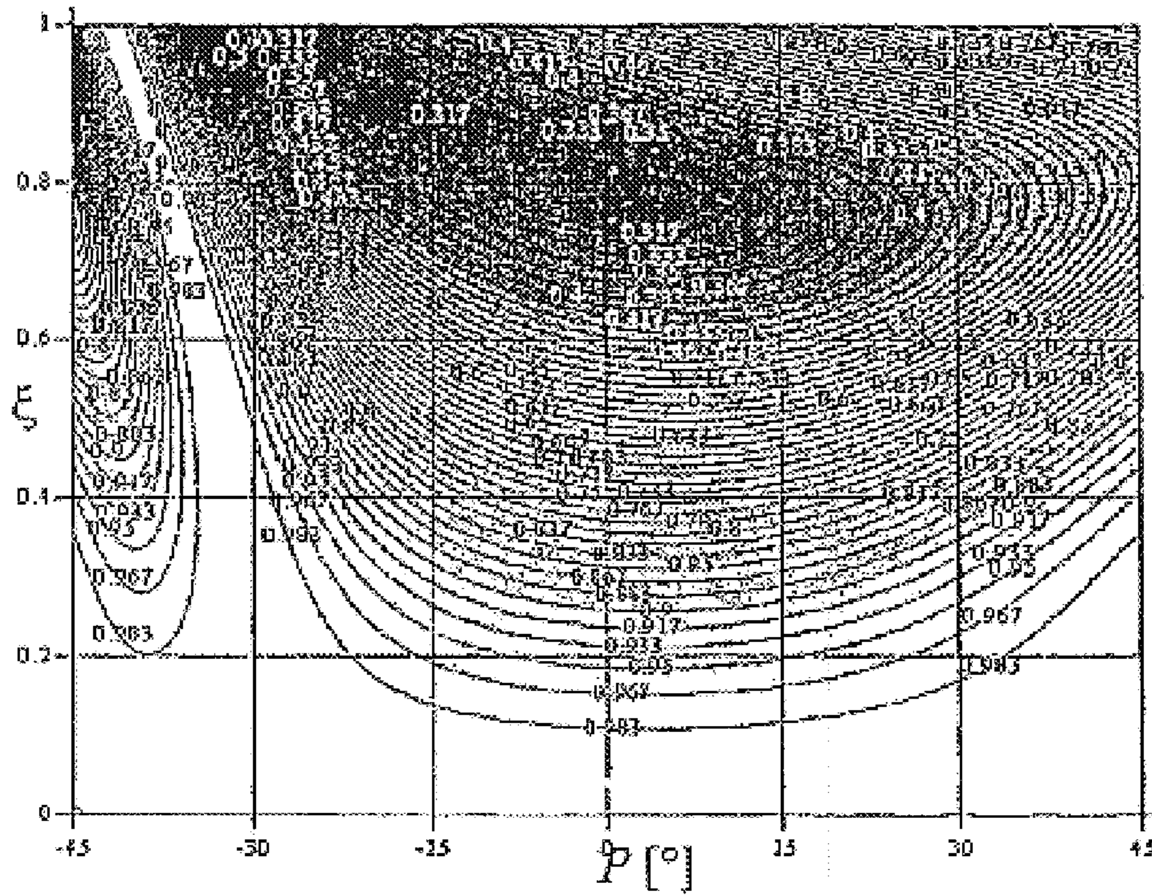
Twist state \Delta\Phi_0 + \pi
