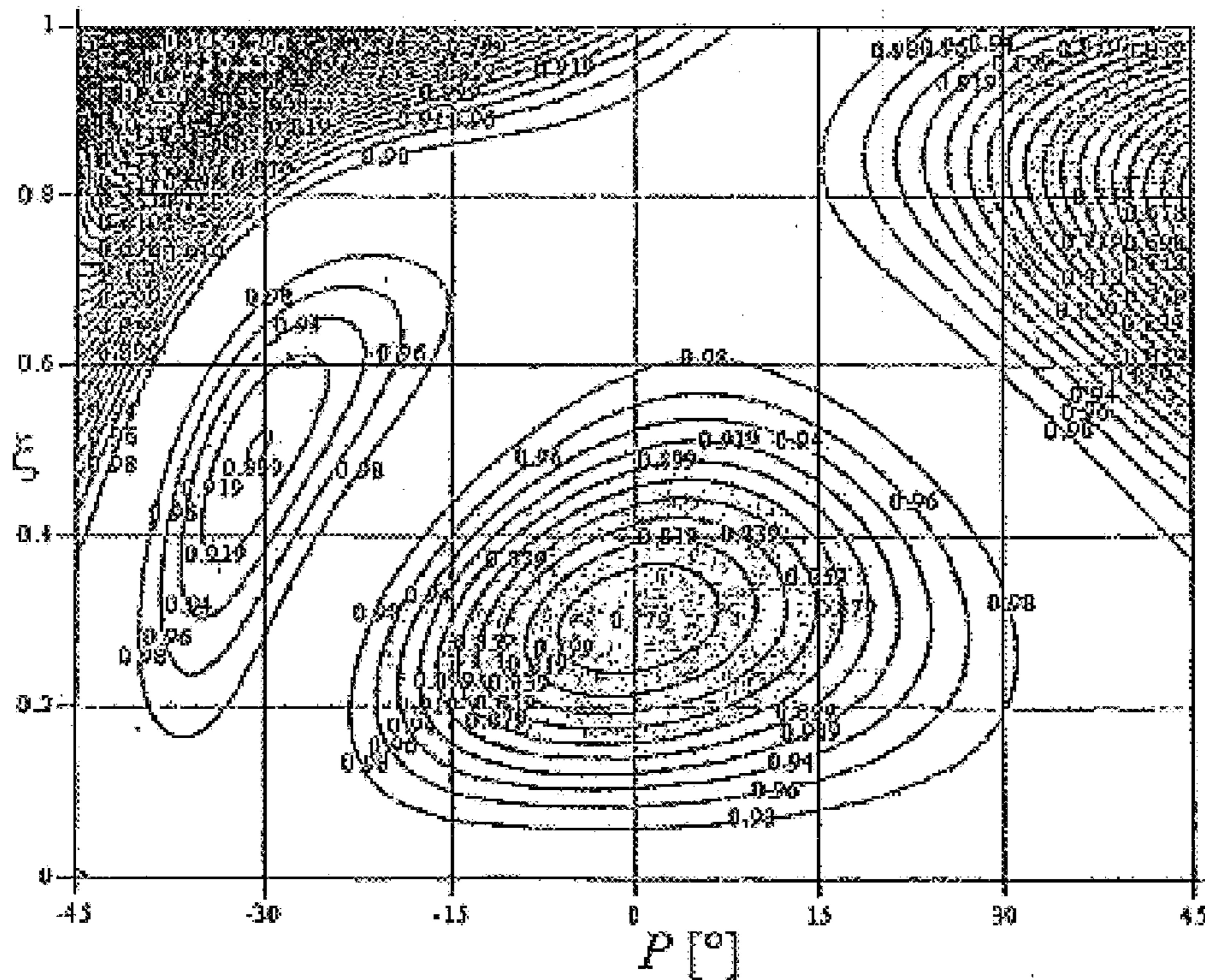
Twist state \Delta\Phi_0 - \pi
