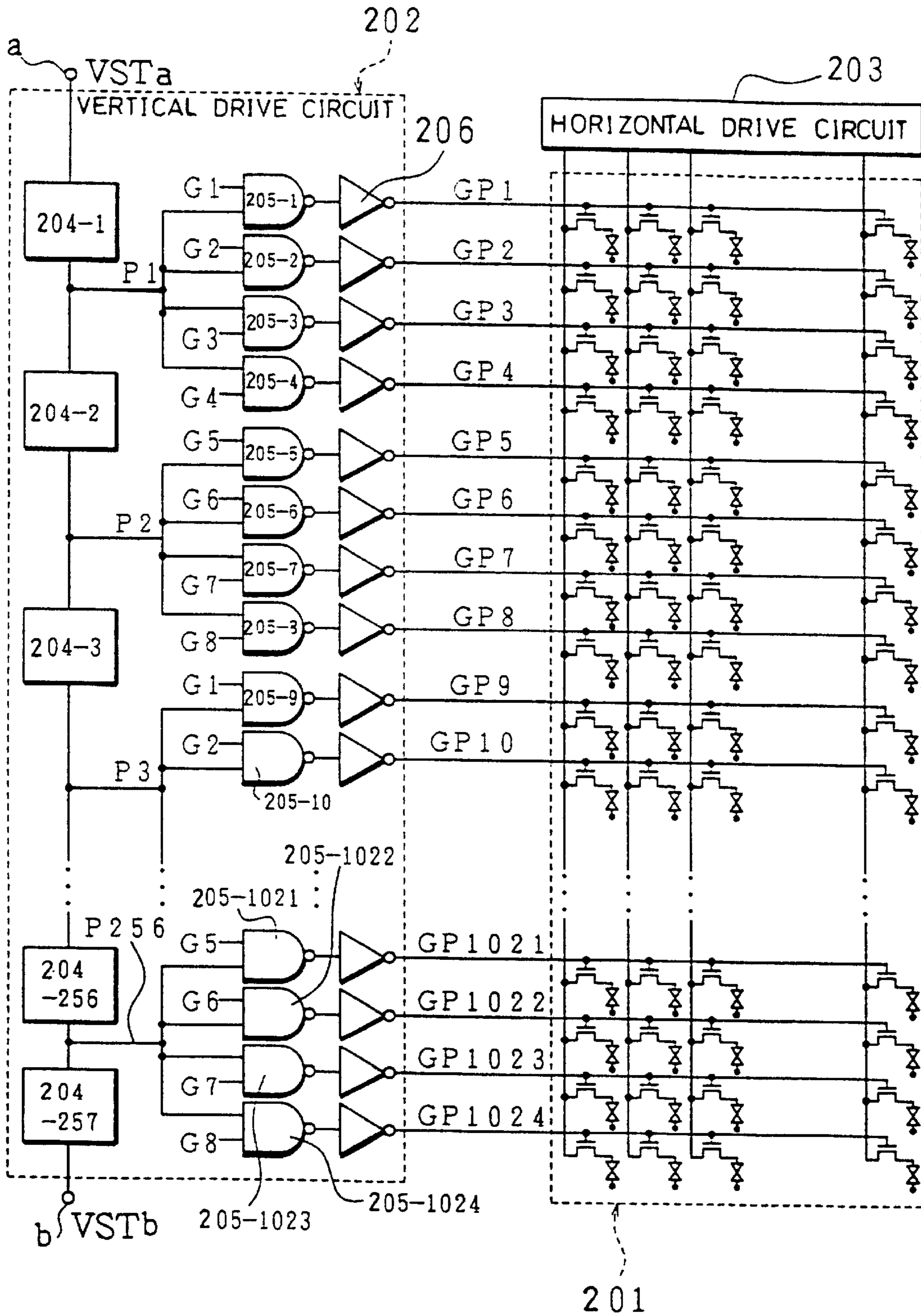
FIG. 31 (Prior Art)
