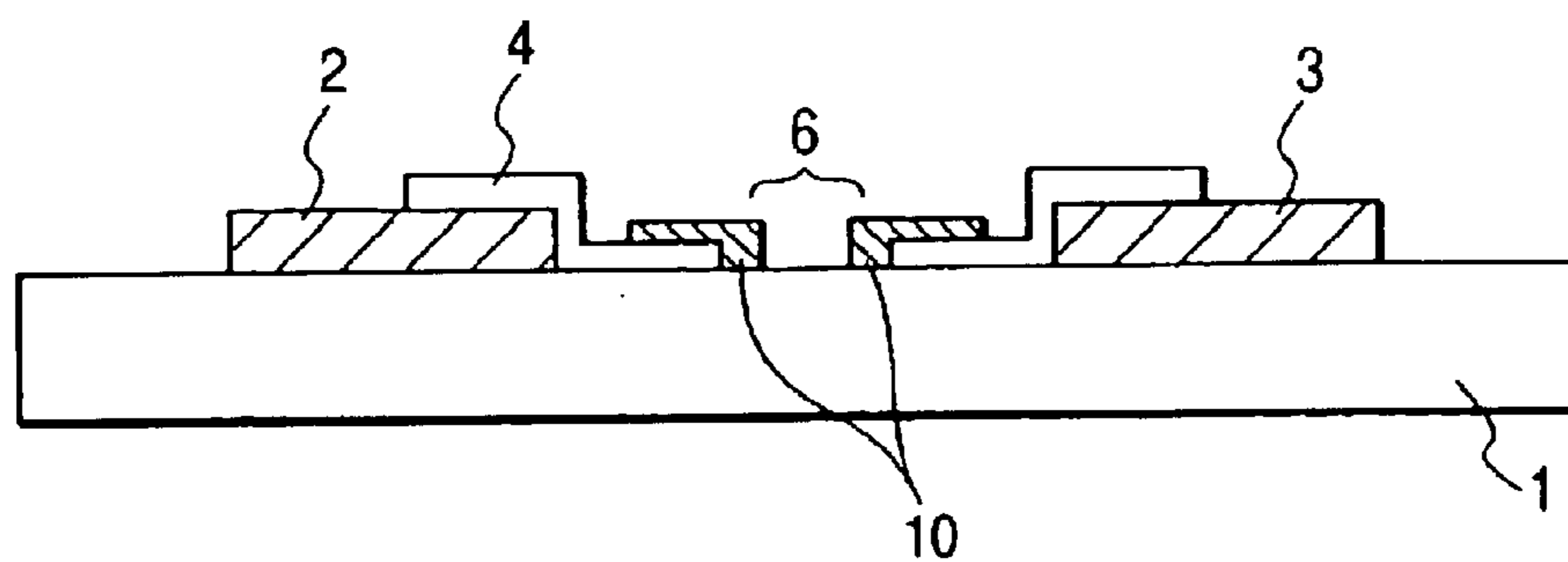
FIG. 3D
