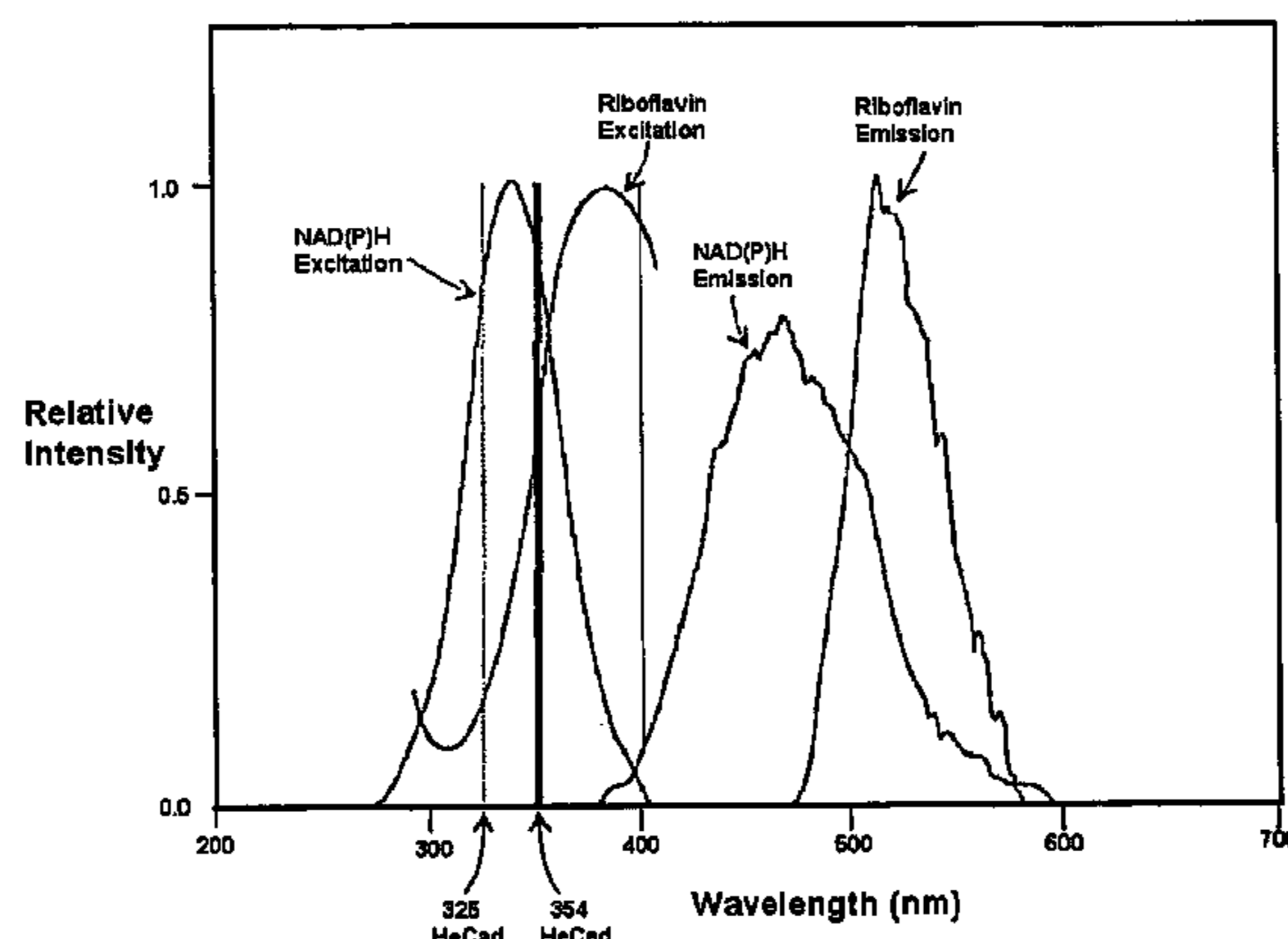
Excitation and Emission Bands of NAD(P)H and Riboflavin
