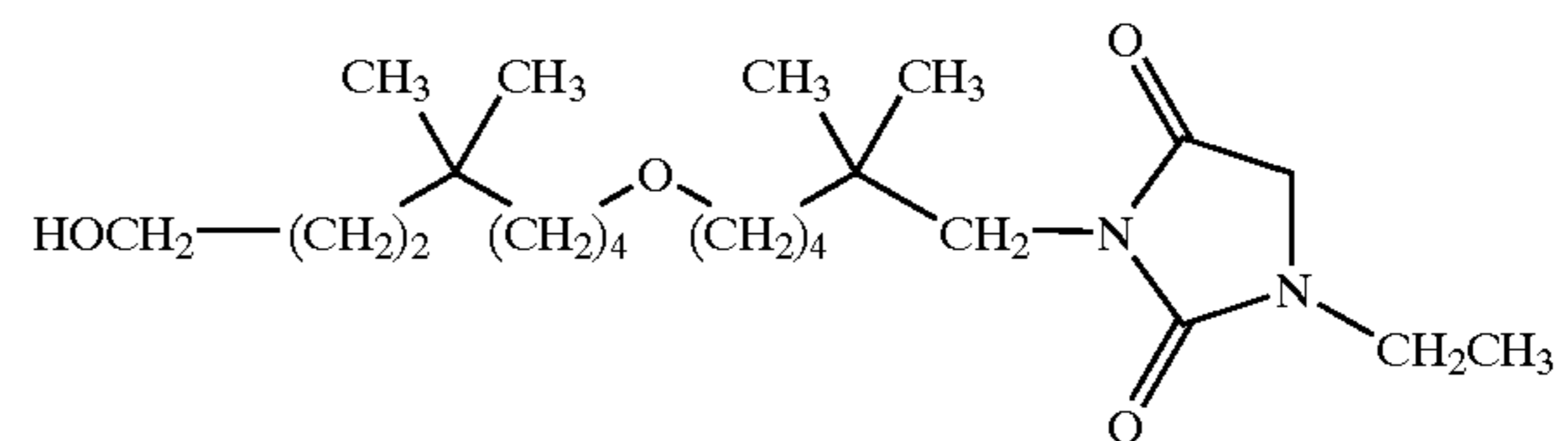
1-ethyl-3-[6-(8-hydroxy-5,5-dimethyl-octyloxy)-2,2-dimethyl-hexyl]-imidazolidine-2,4-dione;
