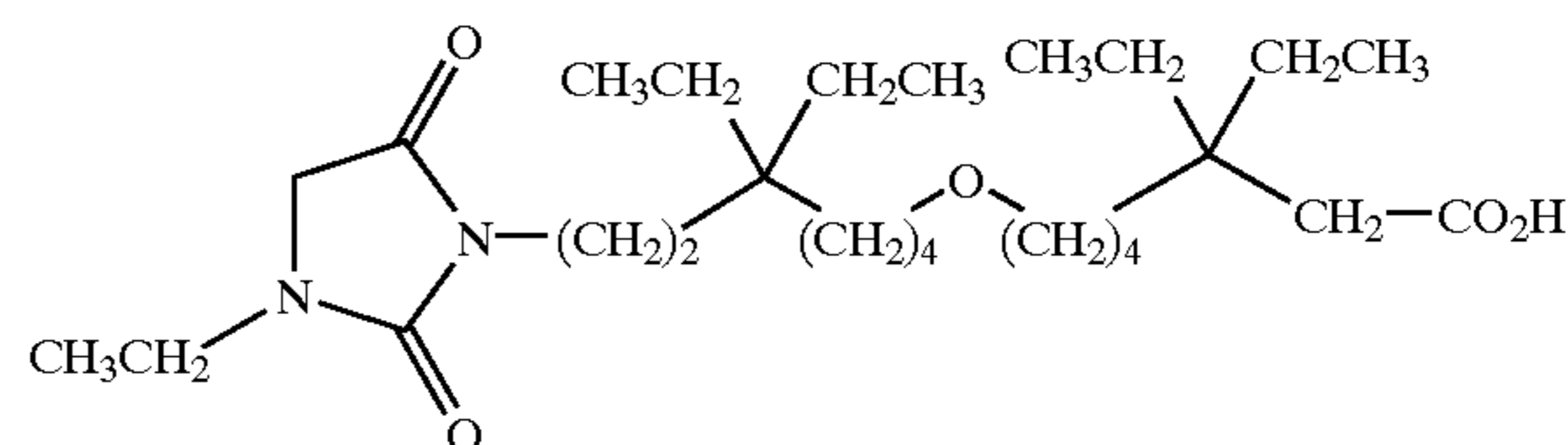
7-[5,5-diethyl-7-(3-ethyl-2,5-dioxo-imidazolidin-1-yl)-heptyloxy]-3,3-diethyl-heptanoic acid;
