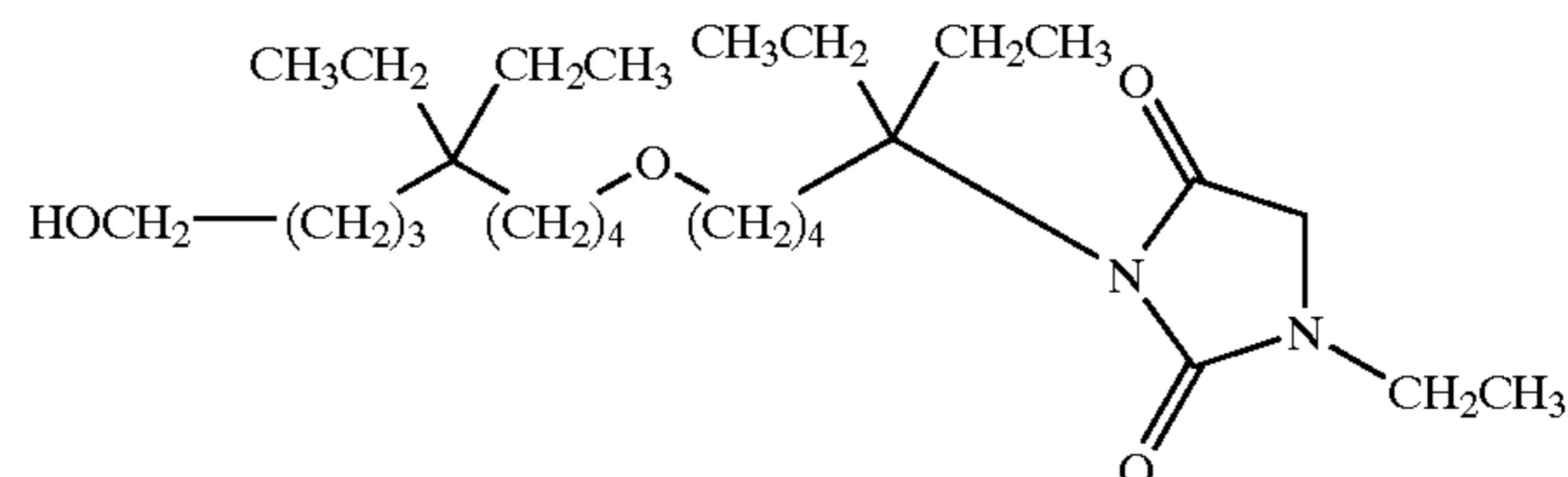
3-[5-(5,5-diethyl-9-hydroxy-nonyloxy)-1,1-diethyl-pentyl]-1-ethyl-imidazolidine-2,4-dione;
