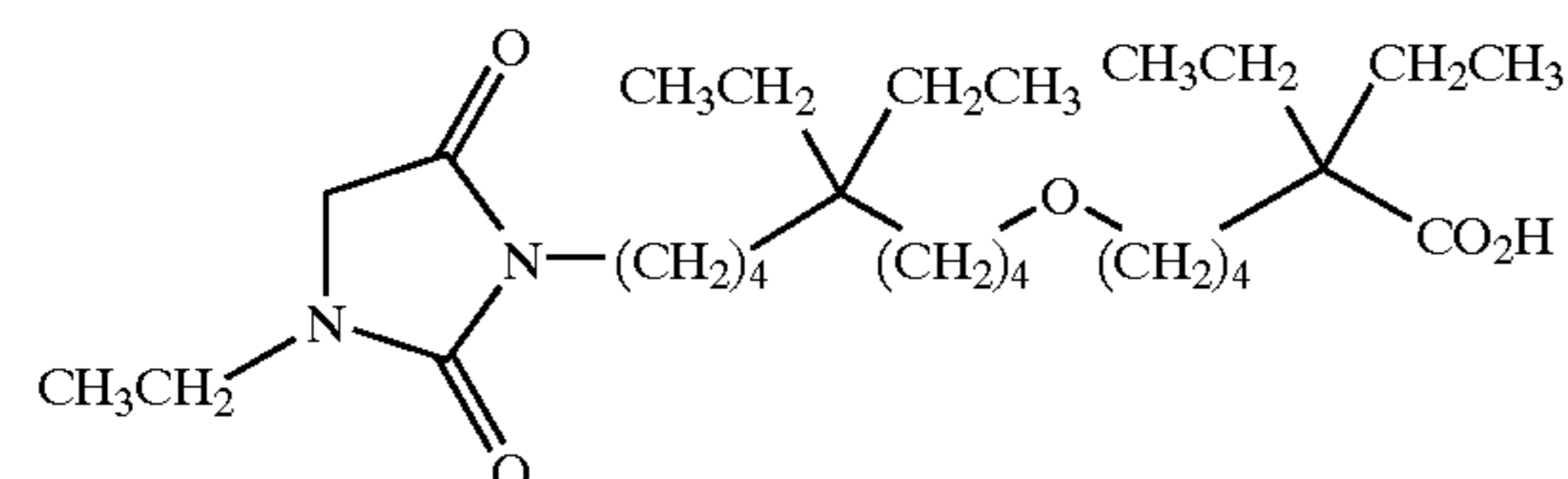
6-[5,5-diethyl-9-(3-ethyl-2,5-dioxo-imidazolidin-1-yl)-nonyloxy]-2,2-diethyl-hexanoic acid;
