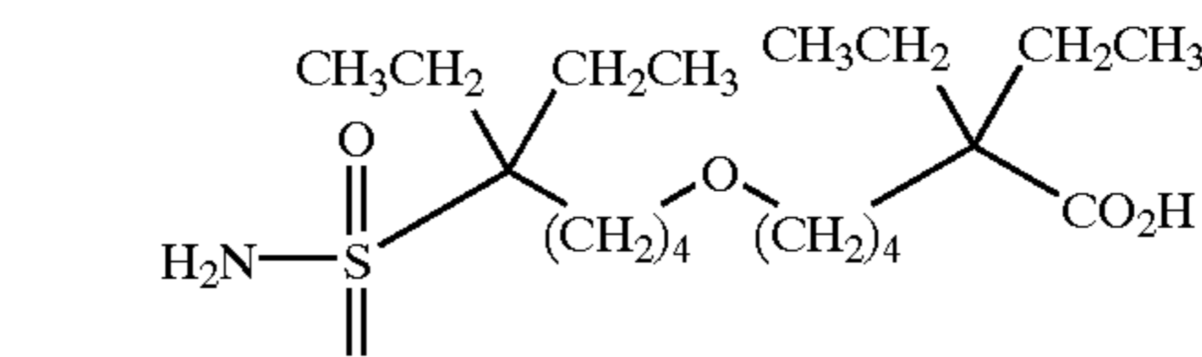
2,2-diethyl-6-(5-ethyl-5-sulfamoyl-heptyloxy)-hexanoic acid;
