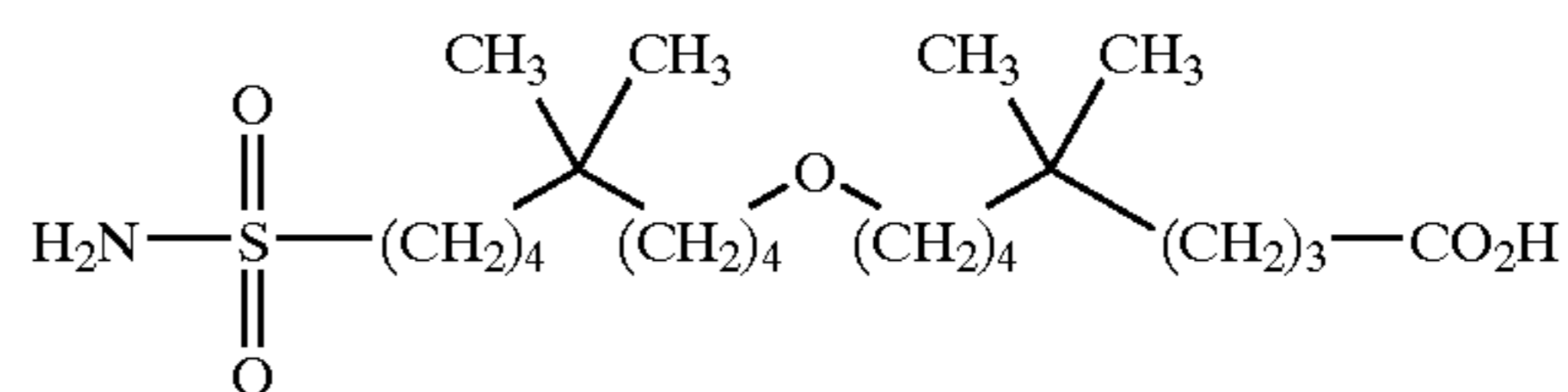
9-(5,5-dimethyl-9-sulfamoyl-nonyloxy)-5,5-dimethyl-nonanoic acid;
