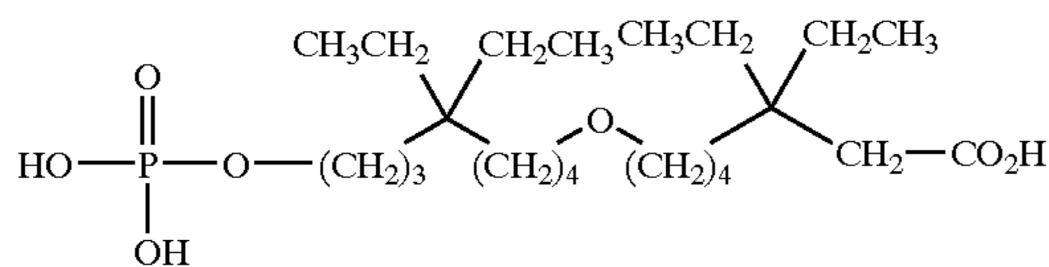
7-(5,5-diethyl-8-phosphonooxy-octyloxy)-3,3-diethyl-heptanoic acid;
