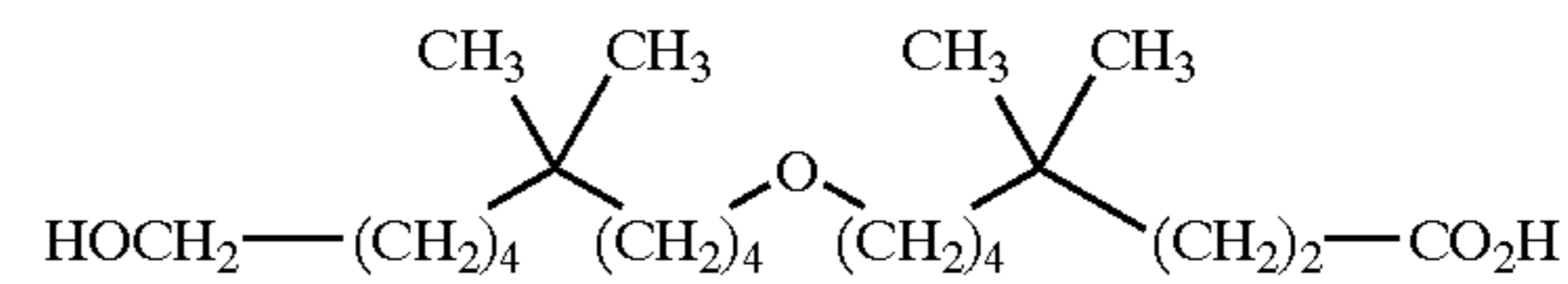
8-(10-hydroxy-5,5-dimethyl-decyloxy)-4,4-dimethyl-octanoic acid;
