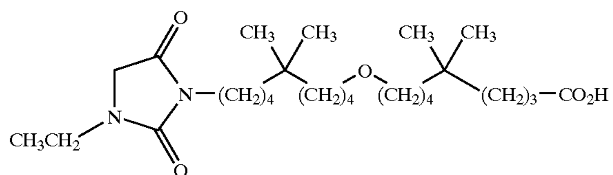
9-[9-(3-ethyl-2,5-dioxo-imidazolidin-1-yl)-5,5-dimethyl-nonyloxy]-5,5-dimethyl-nonanoic acid;
