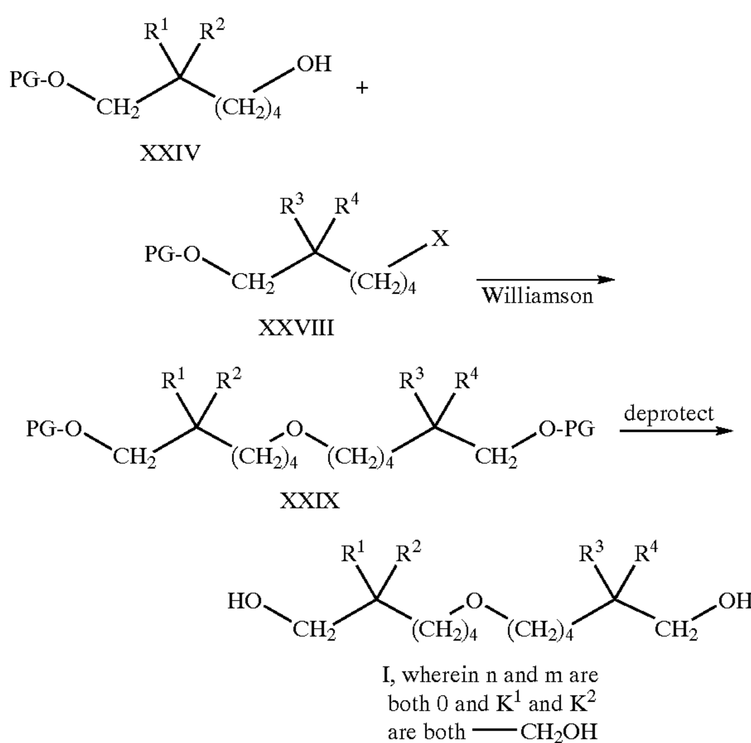
SCHEME 7: Synthesis of compounds of formula I wherein n and m are both 0 and K^1 and K^2 are both \text{—CH}_2\text{OH}
