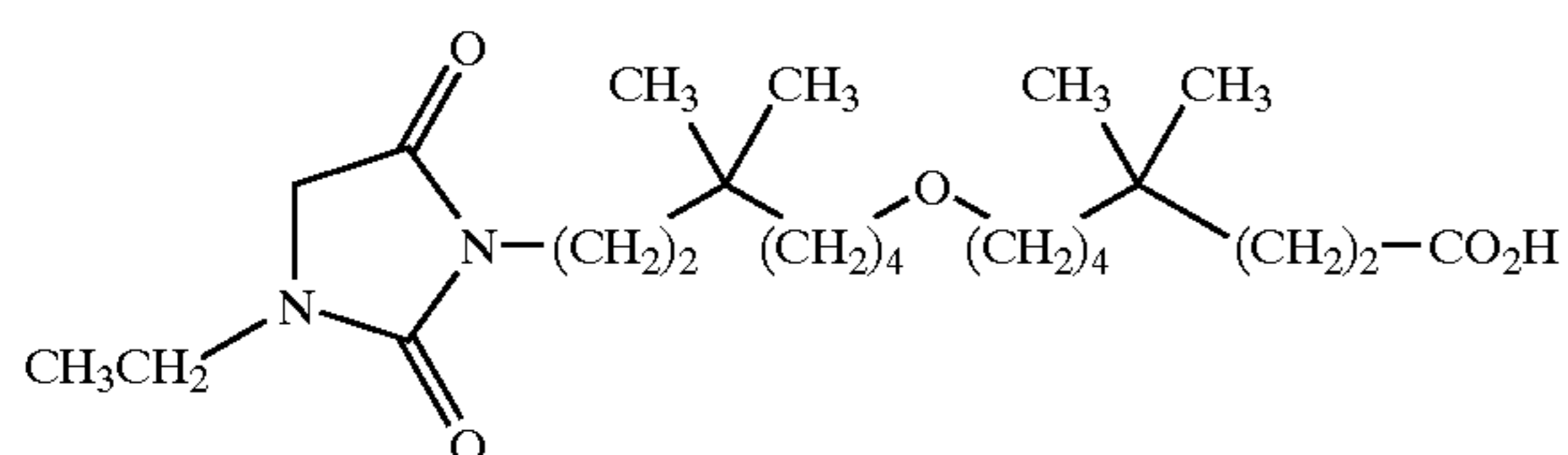
8-[7-(3-ethyl-2,5-dioxo-imidazolidin-1-yl)-5,5-dimethyl-heptyloxy]-4,4-dimethyl-octanoic acid;
