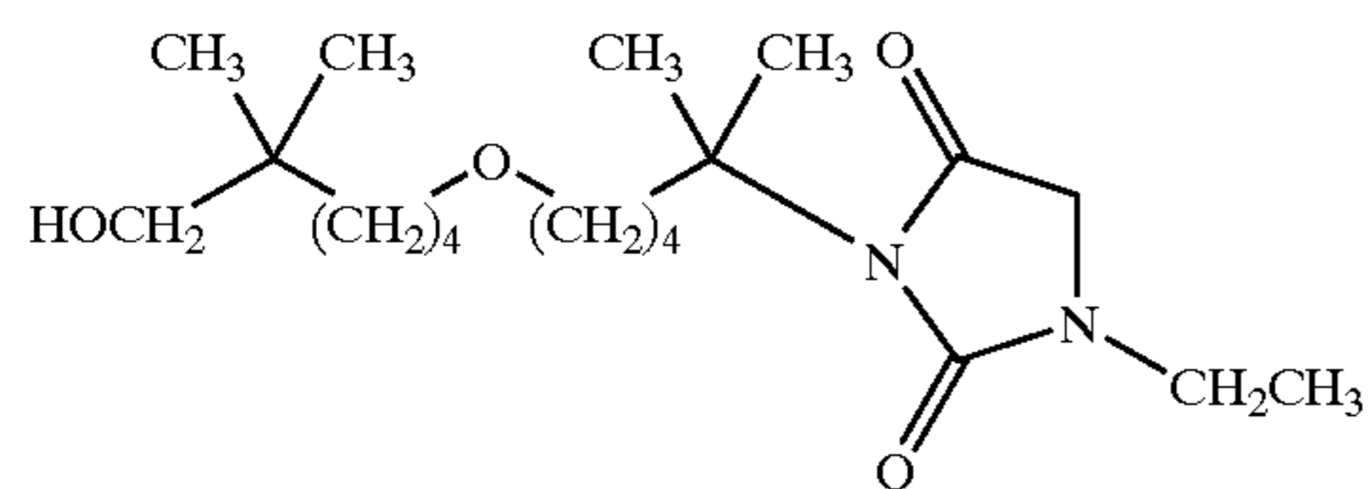
1-ethyl-3-[5-(6-hydroxy-5,5-dimethyl-hexyloxy)-1,1-dimethyl-pentyl]-imidazolidine-2,4-dione;
