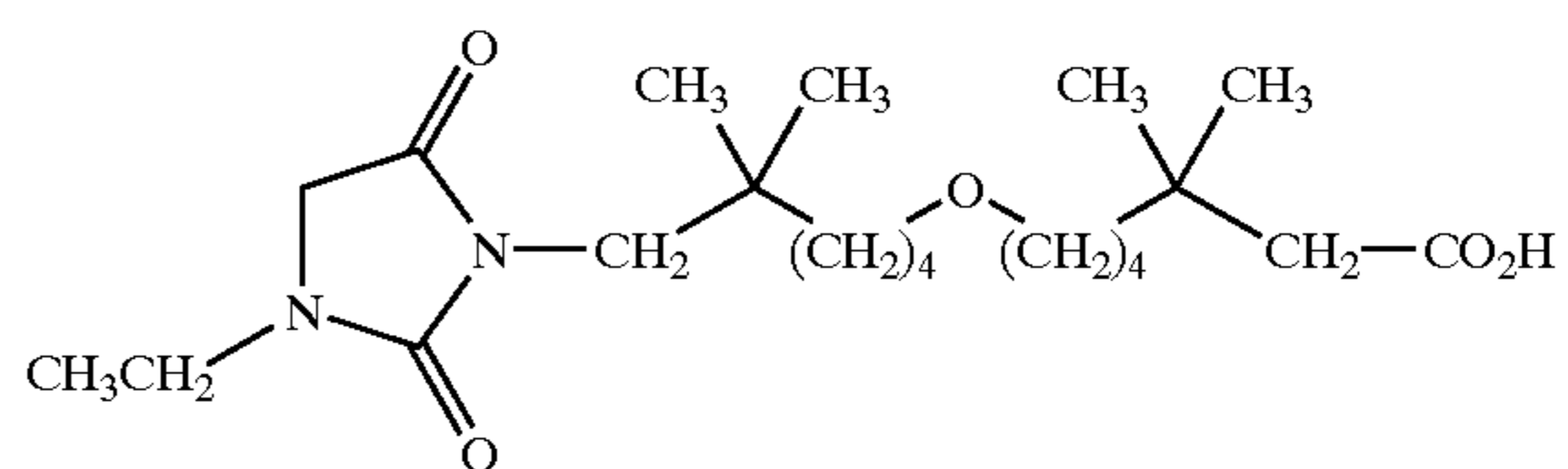
7-[6-(3-ethyl-2,5-dioxo-imidazolidin-1-yl)-5,5-dimethyl-hexyloxy]-3,3-dimethyl-heptanoic acid;
