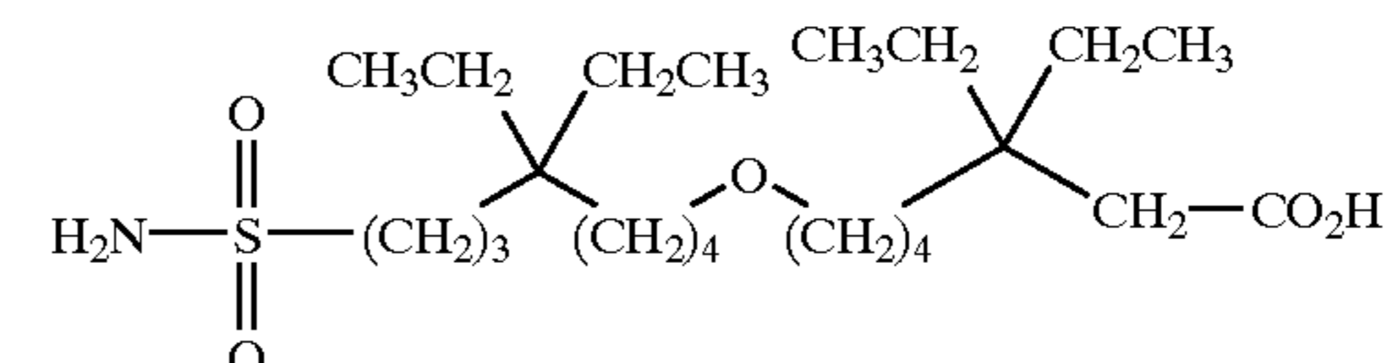
7-(5,5-diethyl-8-sulfamoyl-octyloxy)-3,3-diethyl-heptanoic acid;
