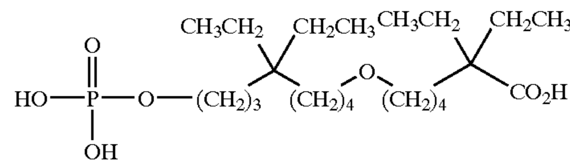
6-(5,5-diethyl-8-phosphonooxy-octyloxy)-2,2-diethyl-hexanoic acid;
