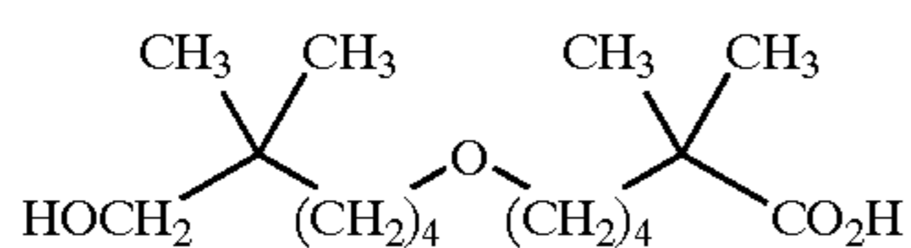
6-(6-hydroxy-5,5-dimethyl-hexyloxy)-2,2-dimethyl-hexanoic acid;
