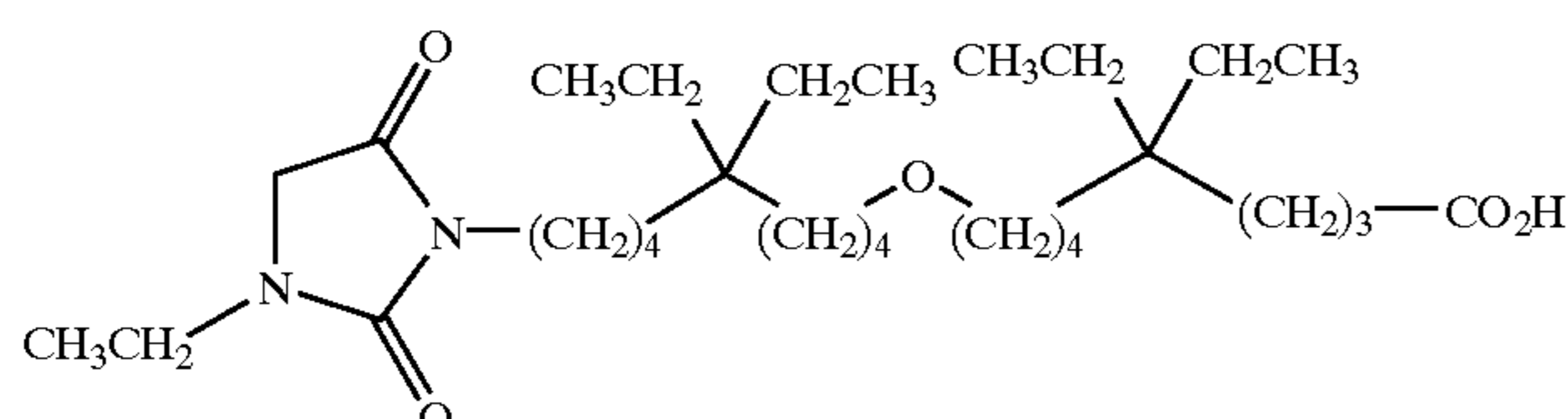
9-[5,5-diethyl-9-(3-ethyl-2,5-dioxo-imidazolidin-1-yl)-nonyloxy]-5,5-diethyl-nonanoic acid;
