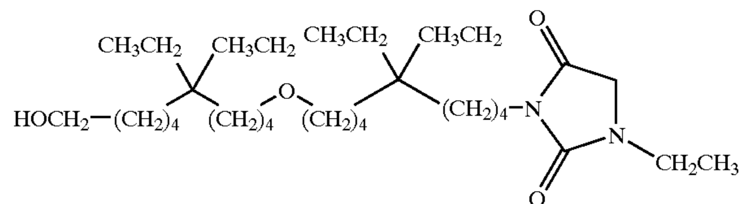
3-[9-(5,5-diethyl-10-hydroxy-decyloxy)-5,5-diethyl-nonyl]-1-ethyl-imidazolidine-2,4-dione;
