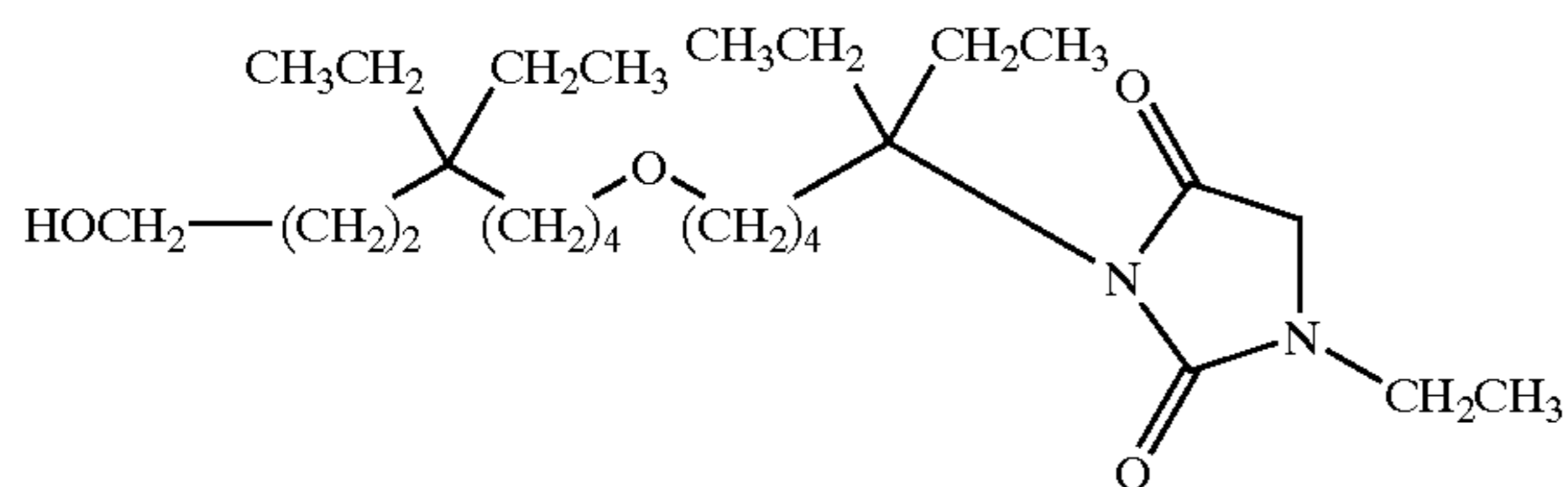
3-[5-(5,5-diethyl-8-hydroxy-octyloxy)-1,1-diethyl-pentyl]-1-ethyl-imidazolidine-2,4-dione;
