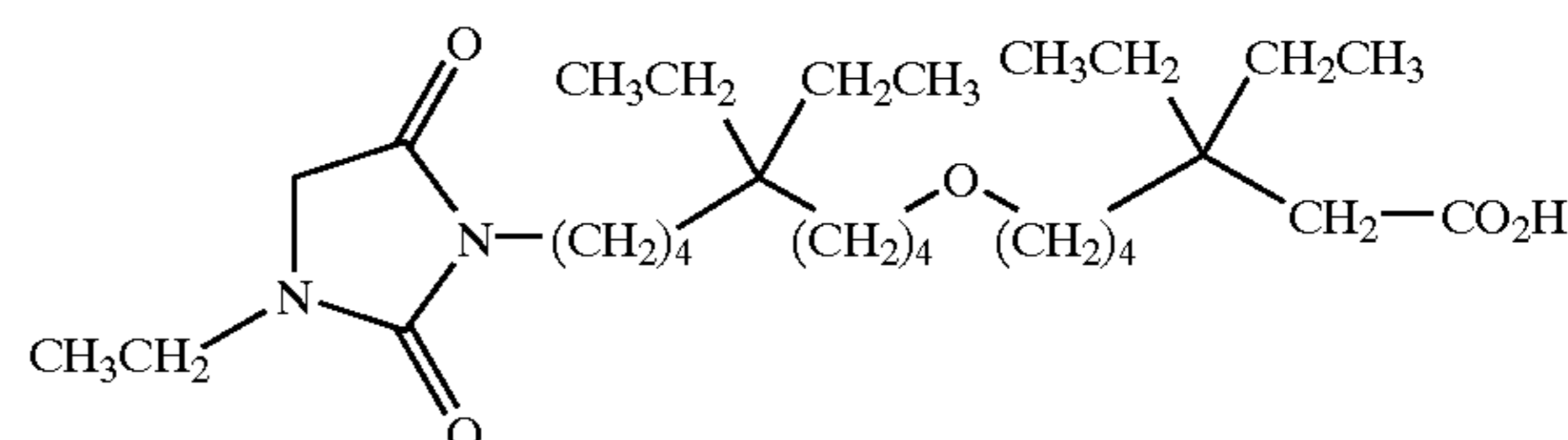
7-[5,5-diethyl-9-(3-ethyl-2,5-dioxo-imidazolidin-1-yl)-nonyloxy]-3,3-diethyl-heptanoic acid;
