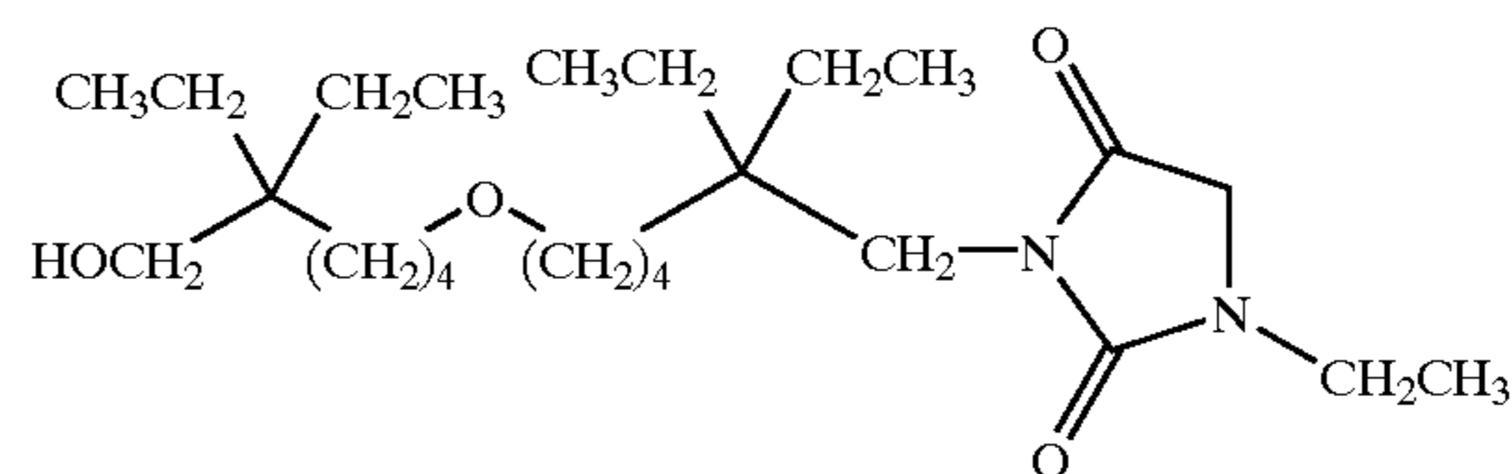
3-[2,2-diethyl-6-(5-ethyl-5-hydroxymethyl-heptyloxy)-hexyl]-1-ethyl-imidazolidine-2,4-dione;
