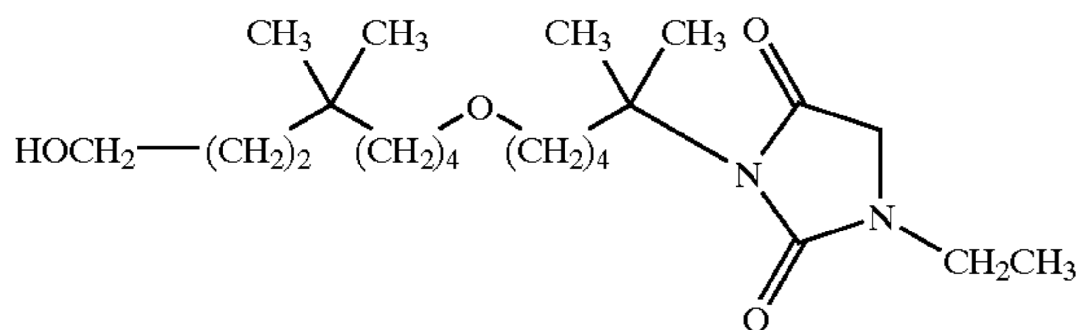
1-ethyl-3-[5-(8-hydroxy-5,5-dimethyl-octyloxy)-1,1-dimethyl-pentyl]-imidazolidine-2,4-dione;
