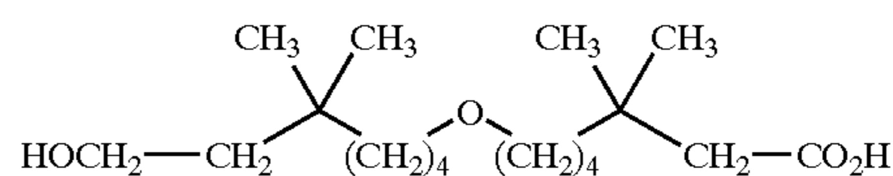
7-(7-hydroxy-5,5-dimethyl-heptyloxy)-3,3-dimethyl-heptanoic acid;
