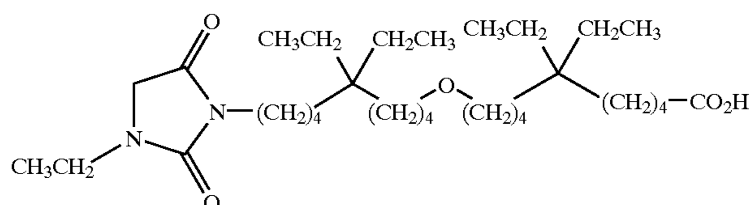
10-[5,5-diethyl-9-(3-ethyl-2,5-dioxo-imidazolidin-1-yl)-nonyloxy]-6,6-diethyl-decanoic acid;
