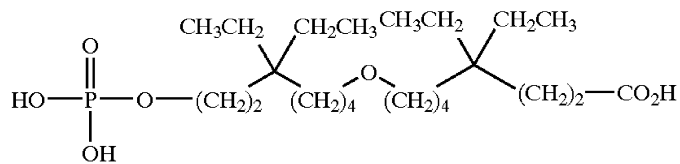
8-(5,5-diethyl-7-phosphonooxy-heptyloxy)-4,4-diethyl-octanoic acid;
