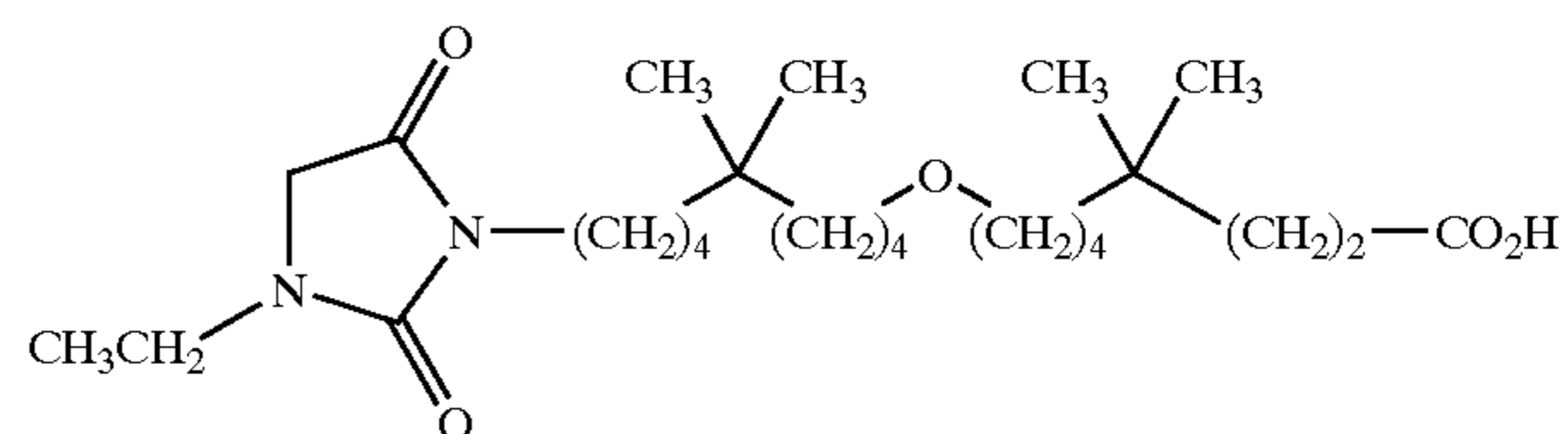
8-[9-(3-ethyl-2,5-dioxo-imidazolidin-1-yl)-5,5-dimethyl-nonyloxy]-4,4-dimethyl-octanoic acid;
