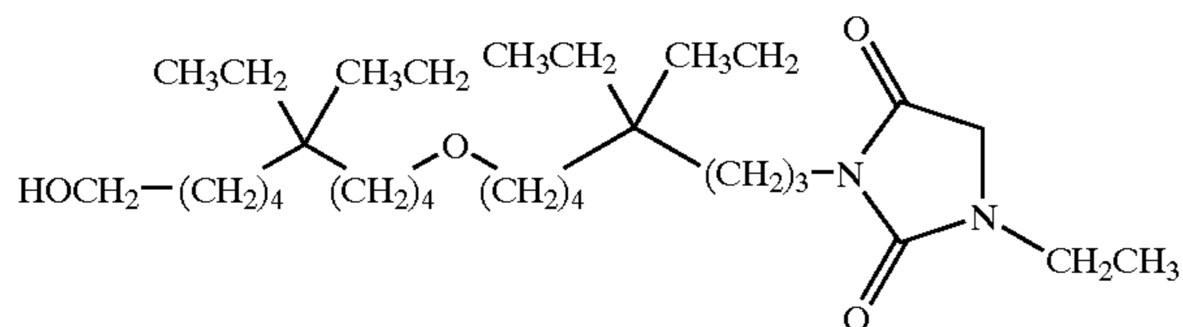
3-[8-(5,5-diethyl-10-hydroxy-decyloxy)-4,4-diethyl-octyl]-1-ethyl-imidazolidine-2,4-dione;
