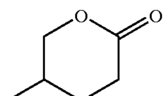
delta lactone
