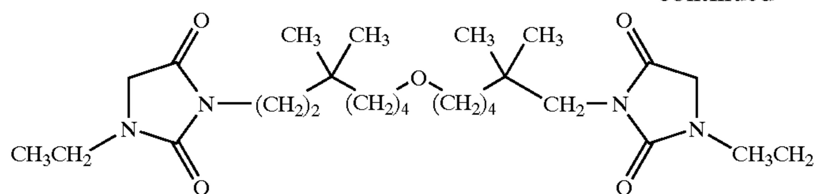
3-[6-(7-(3-ethyl-2,5-dioxo-imidazolidin-1-yl)-5,5-dimethyl-heptyloxy)-2,2-dimethyl-hexyl]-1-ethyl-imidazolidine-2,4-dione;
