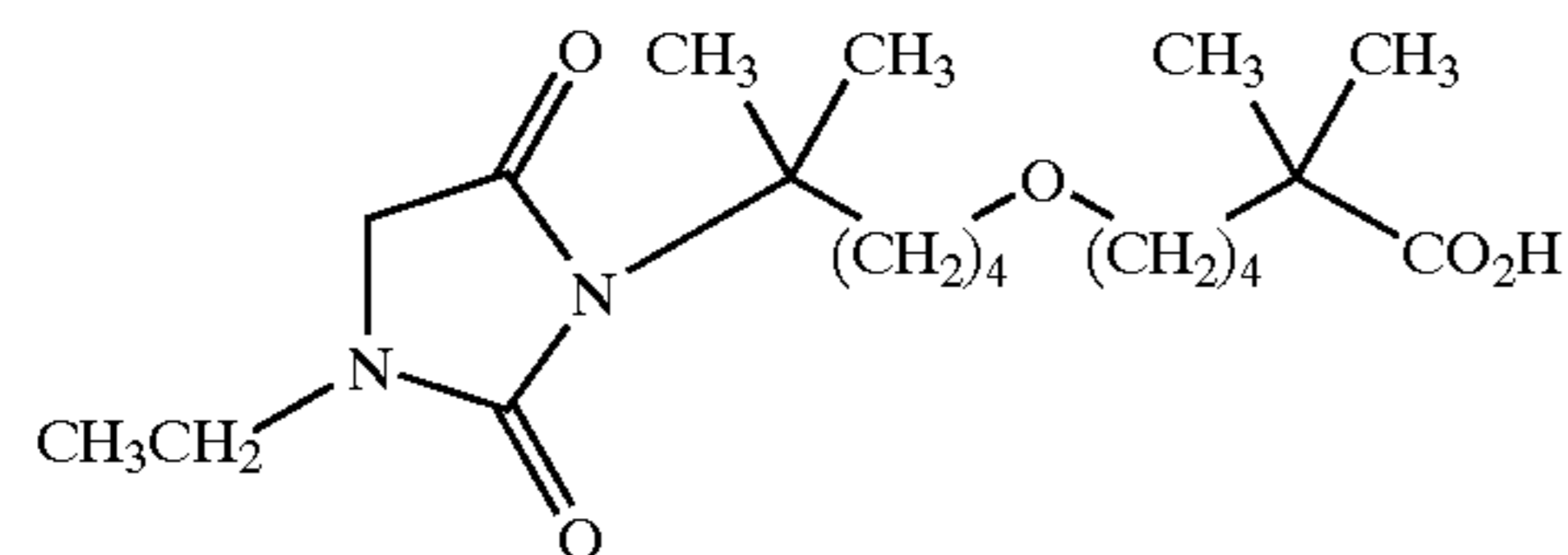
6-[5-(3-ethyl-2,5-dioxo-imidazolidin-1-yl)-5-methyl-hexyloxy]-2,2-dimethyl-hexanoic acid;
