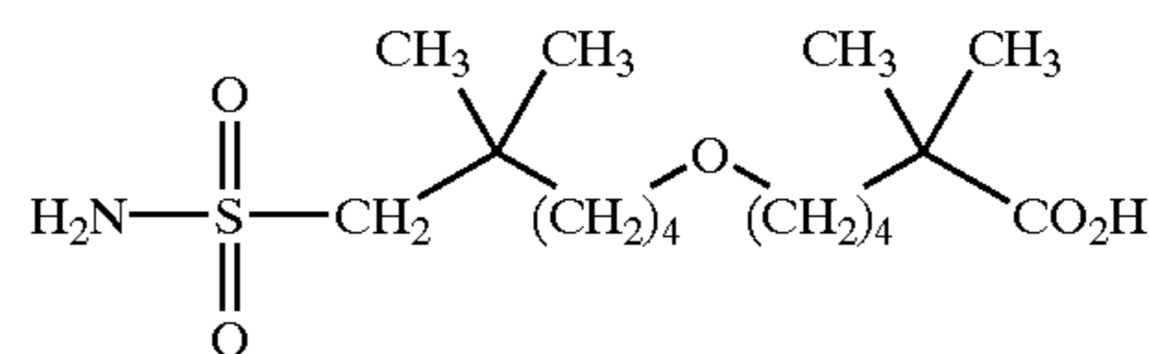
6-(5,5-dimethyl-6-sulfamoyl-hexyloxy)-2,2-dimethyl-hexanoic acid;
