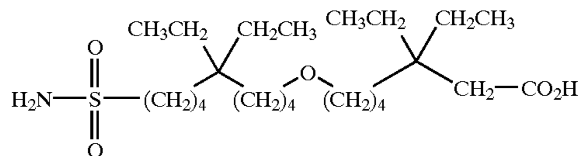
7-(5,5-diethyl-9-sulfamoyl-nonyloxy)-3,3-diethyl-heptanoic acid;
