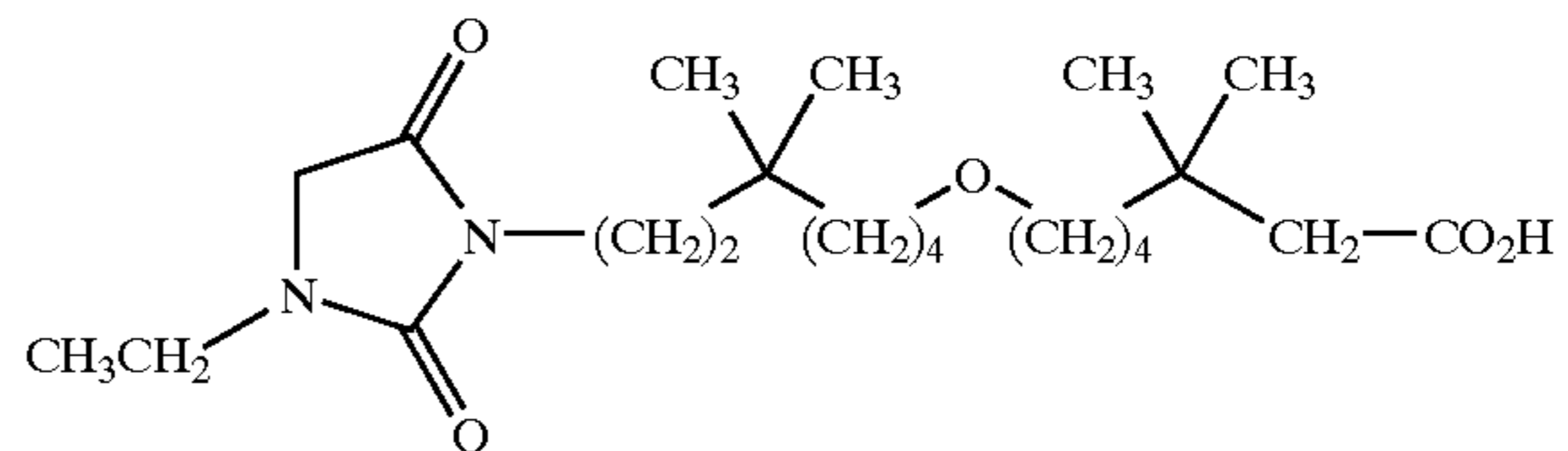
7-[7-(3-ethyl-2,5-dioxo-imidazolidin-1-yl)-5,5-dimethyl-heptyloxy]-3,3-dimethyl-heptanoic acid;
