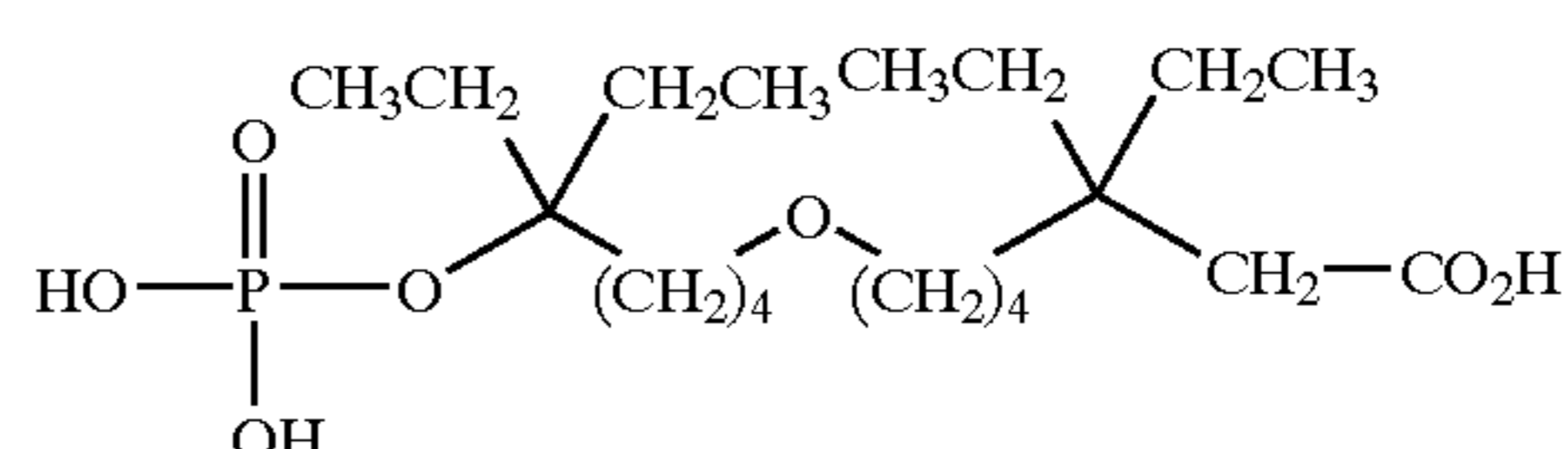
3,3-diethyl-7-(5-ethyl-5-phosphonoxy-heptyloxy)-heptanoic acid;
