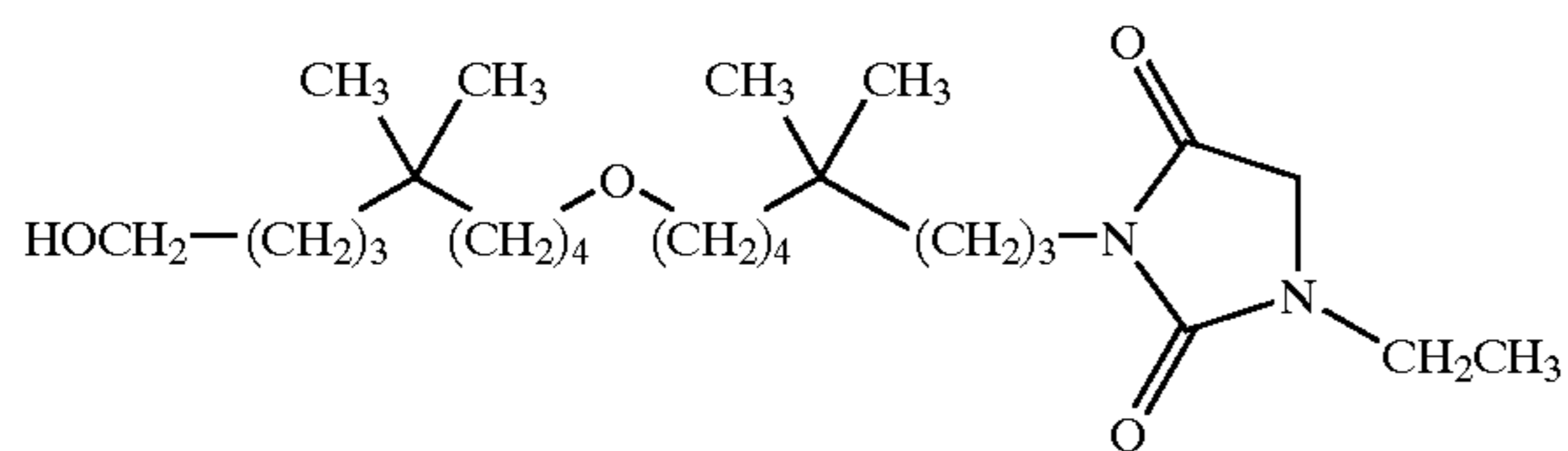
1-ethyl-3-[8-(9-hydroxy-5,5-dimethyl-nonyloxy)-4,4-dimethyl-octyl]-imidazolidine-2,4-dione;
