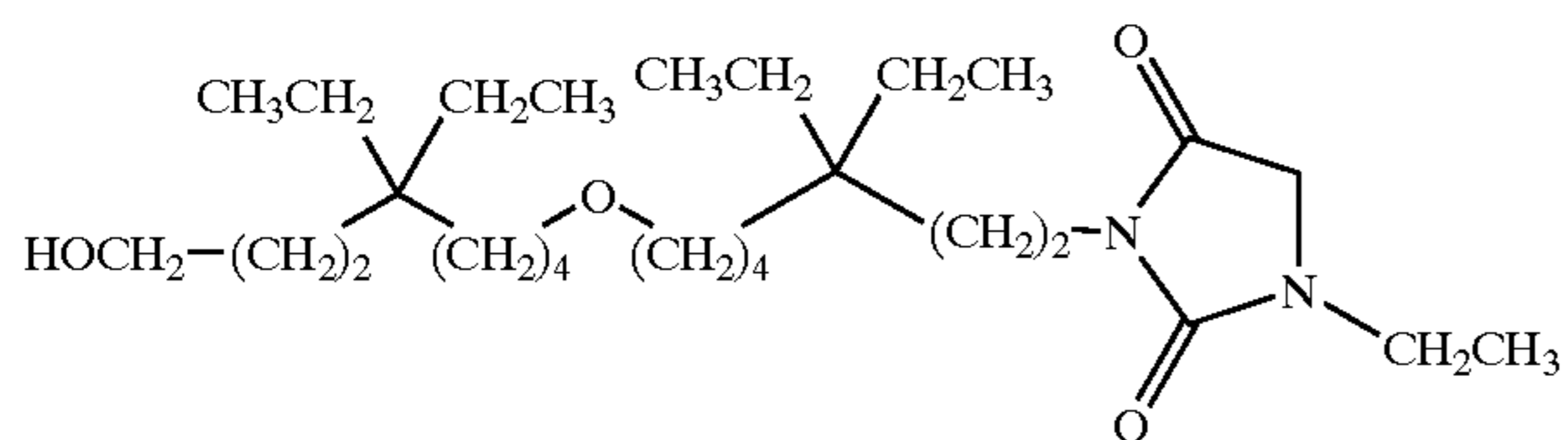
3-[7-(5,5-diethyl-8-hydroxy-octyloxy)-3,3-diethyl-heptyl]-1-ethyl-imidazolidine-2,4-dione;
