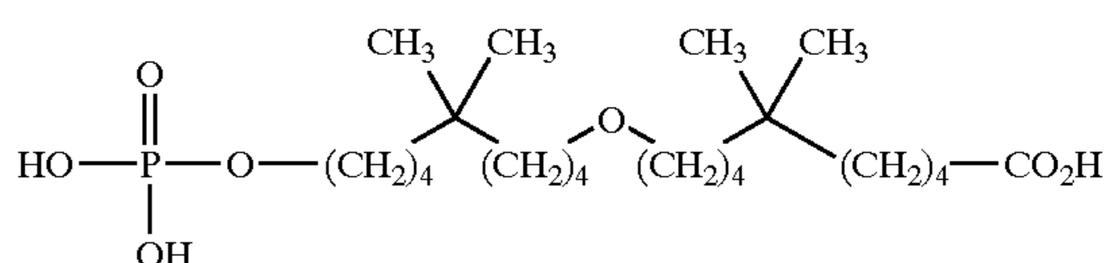
10-(5,5-dimethyl-9-phosphonoxy-nonyloxy)-6,6-dimethyl-decanoic acid;
