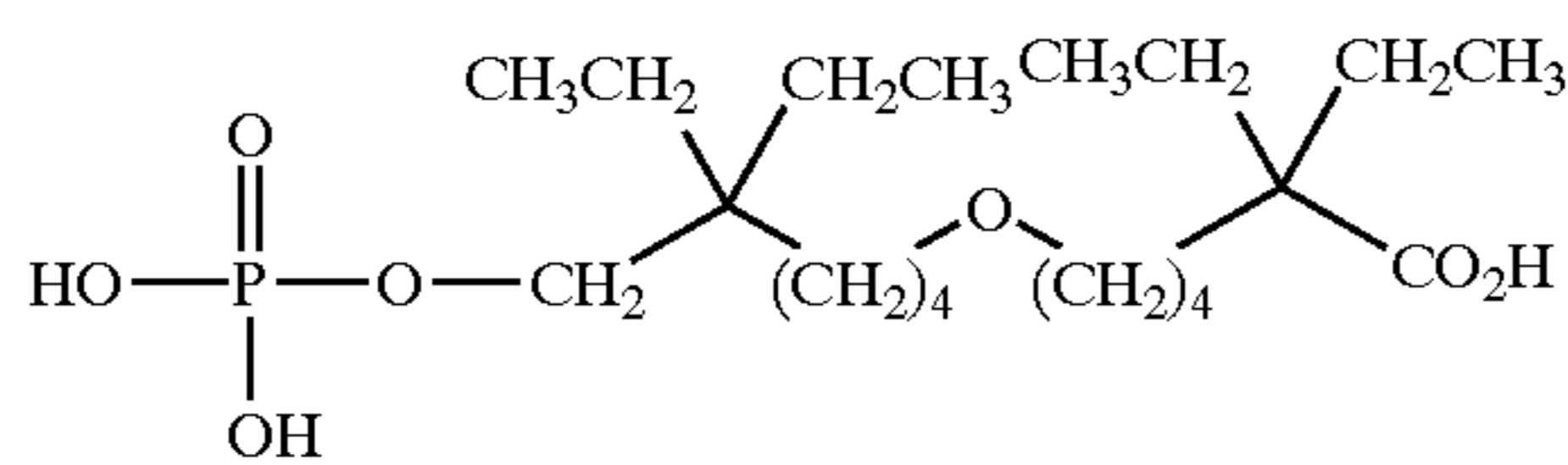
2,2-diethyl-6-(5-ethyl-5-phosphonooxymethyl-heptyloxy)-hexanoic acid;
