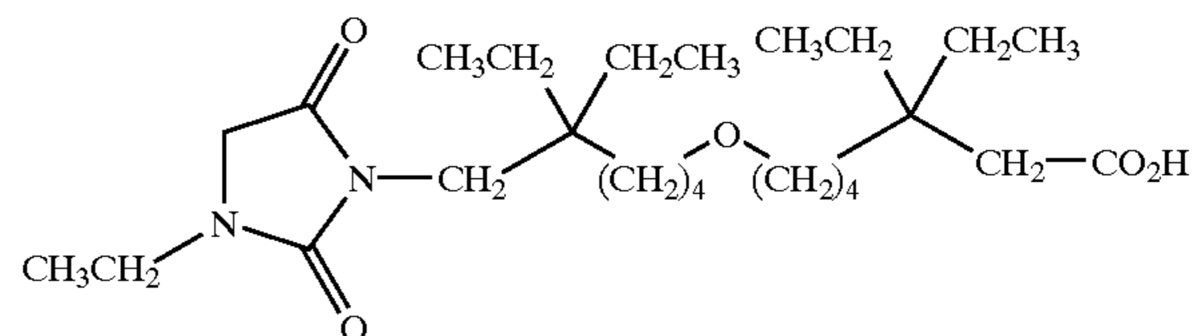
3,3-diethyl-7-[5-ethyl-5-(3-ethyl-2,5-dioxo-imidazolidin-1-ylmethyl)-heptyloxy]-heptanoic acid;
