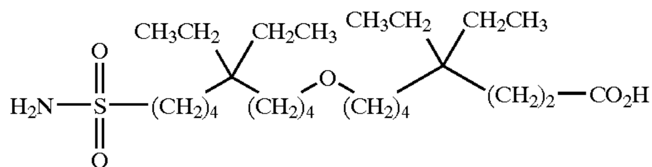
8-(5,5-diethyl-9-sulfamoyl-nonyloxy)-4,4-diethyl-octanoic acid;
