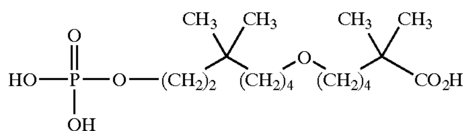
6-(5,5-dimethyl-7-phosphonoxy-heptyloxy)-2,2-dimethyl-hexanoic acid;
