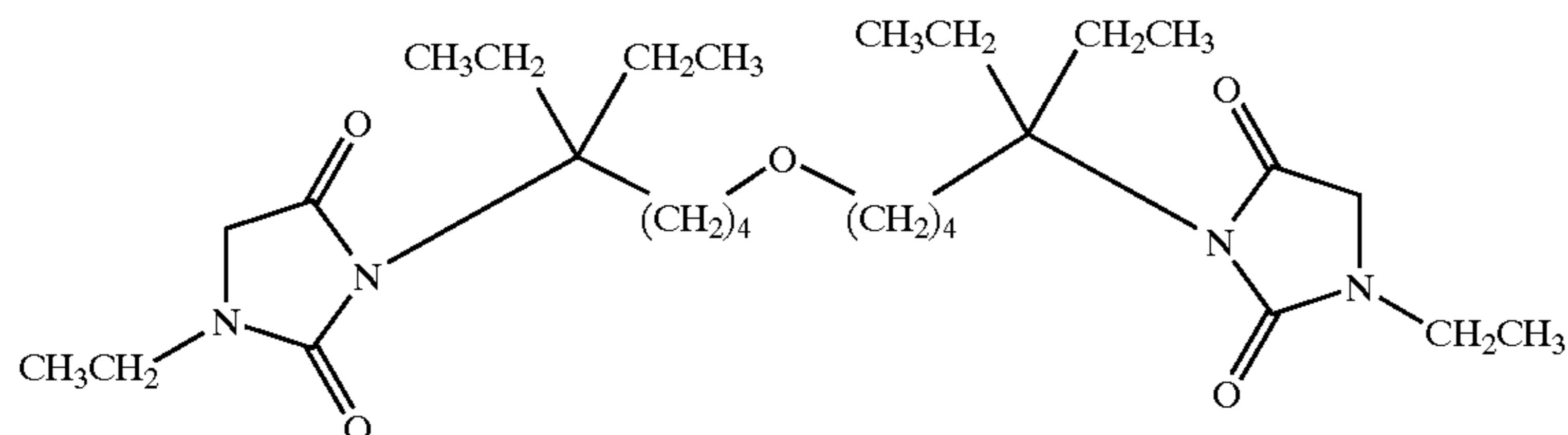
3-[5-(3-ethyl-2,5-dioxo-imidazolidin-1-yl)-5-ethyl-heptyloxy]-1,1-diethyl-pentyl-1-ethyl-imidazolidine-2,4-dione;
