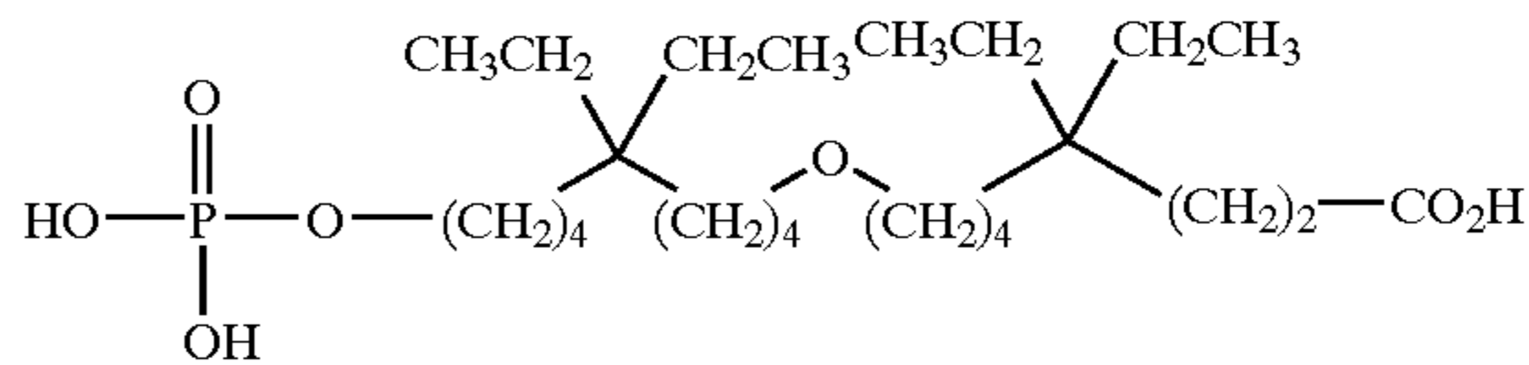
8-(5,5-diethyl-9-phosphonooxy-nonyloxy)-4,4-diethyl-octanoic acid;
