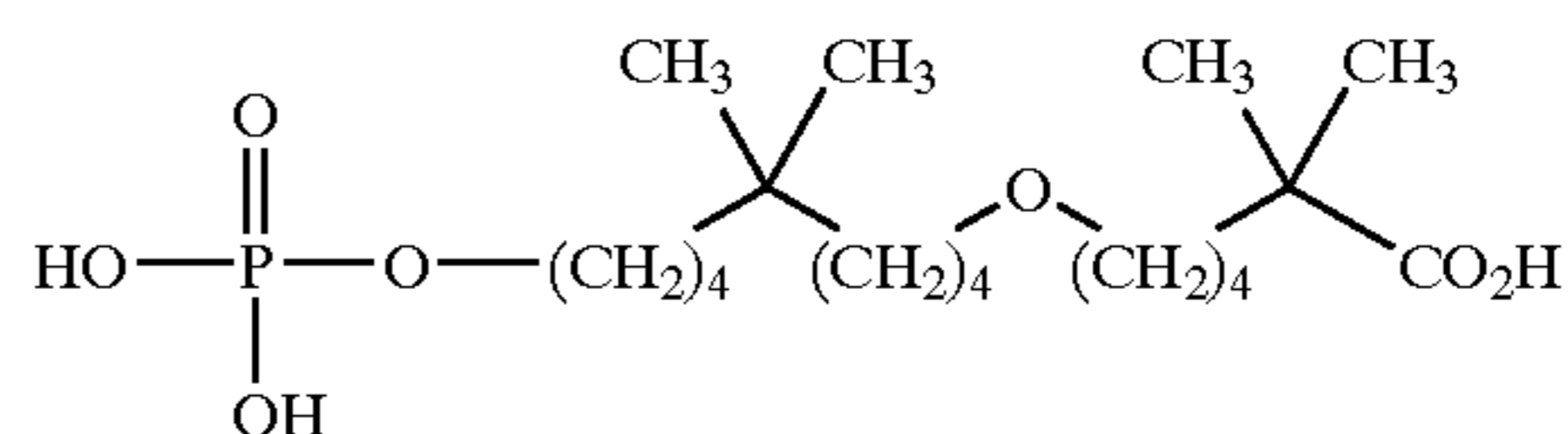
6-(5,5-dimethyl-9-phosphonoxy-nonyloxy)-2,2-dimethyl-hexanoic acid;
