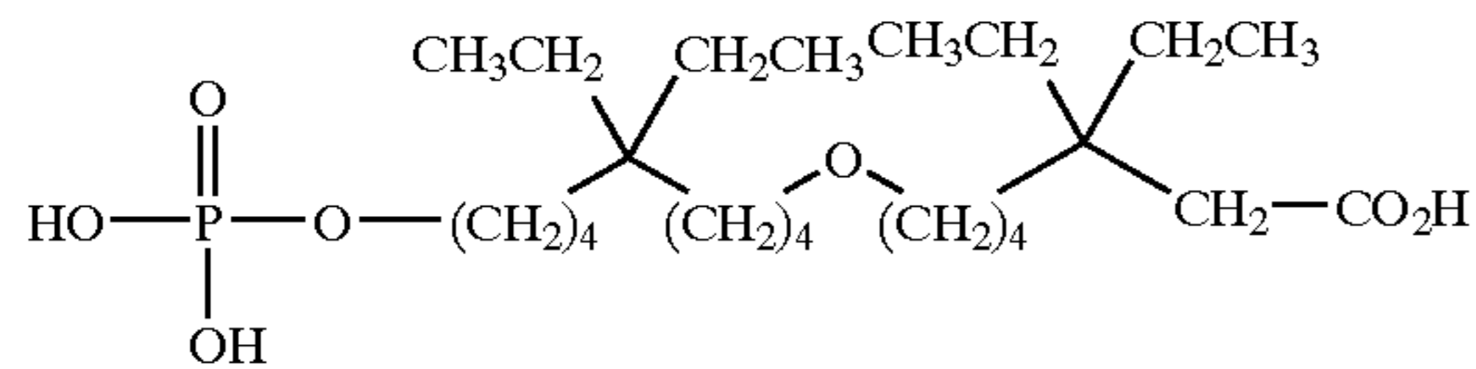
7-(5,5-diethyl-9-phosphonooxy-nonyloxy)-3,3-diethyl-heptanoic acid;
