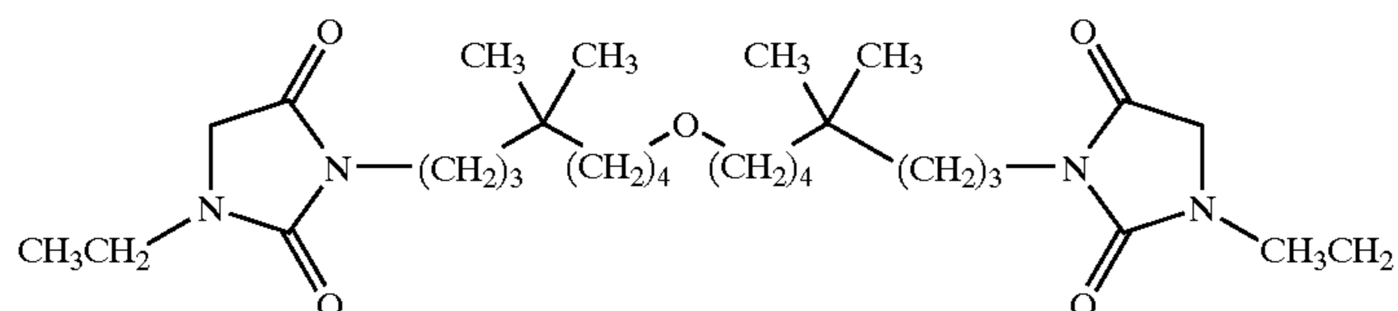
3-[8-(8-(3-ethyl-2,5-dioxo-imidazolidin-1-yl)-5,5-dimethyl-octyloxy)-4,4-dimethyl-octyl]-1-ethyl-imidazolidine-2,4-dione;
