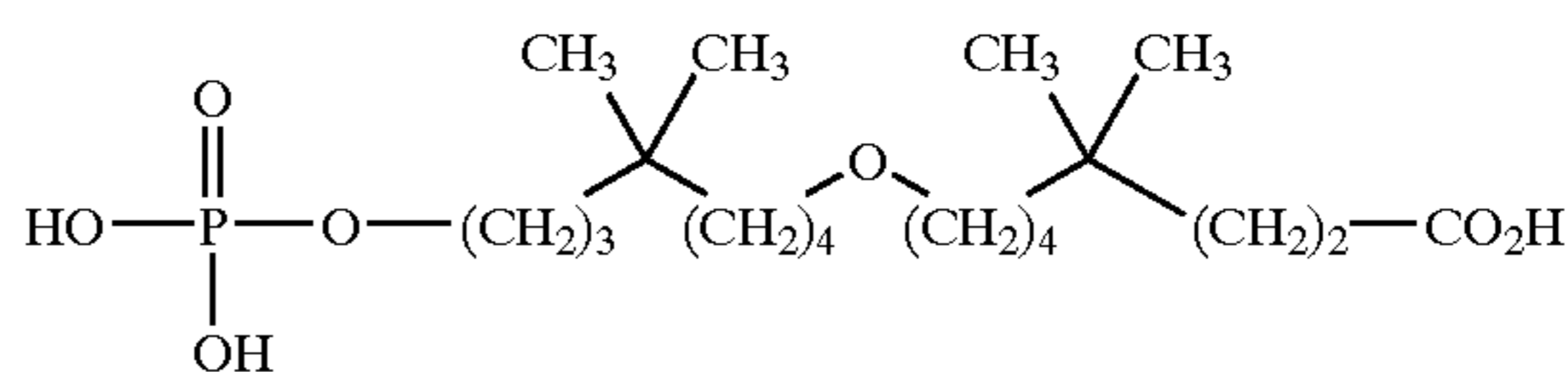
8-(5,5-dimethyl-8-phosphonoxy-octyloxy)-4,4-dimethyl-octanoic acid;
