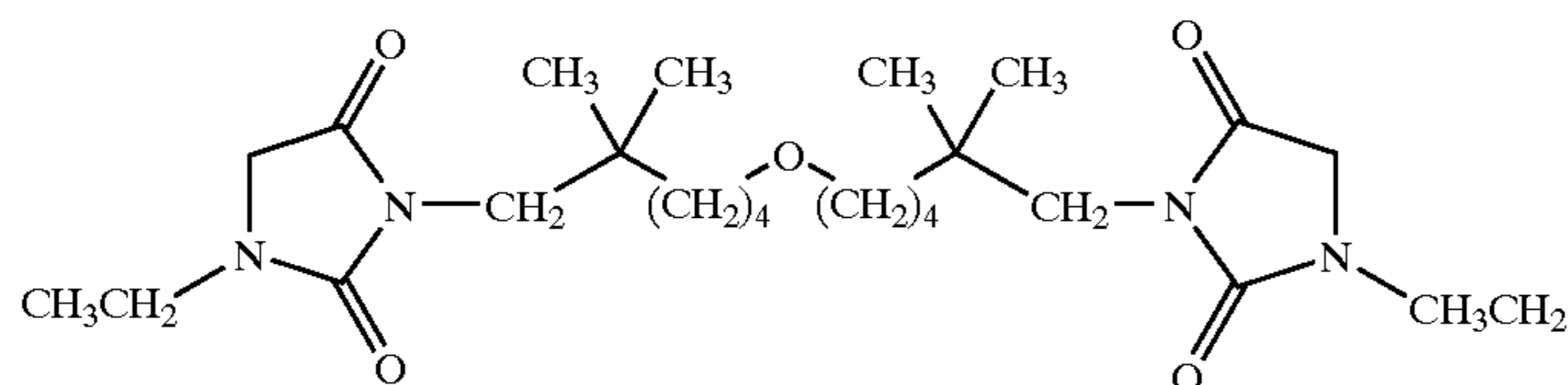
3-[6-(6-(3-ethyl-2,5-dioxo-imidazolidin-1-yl)-5,5-dimethyl-hexyloxy)-2,2-dimethyl-hexyl]-1-ethyl-imidazolidine-2,4-dione;
