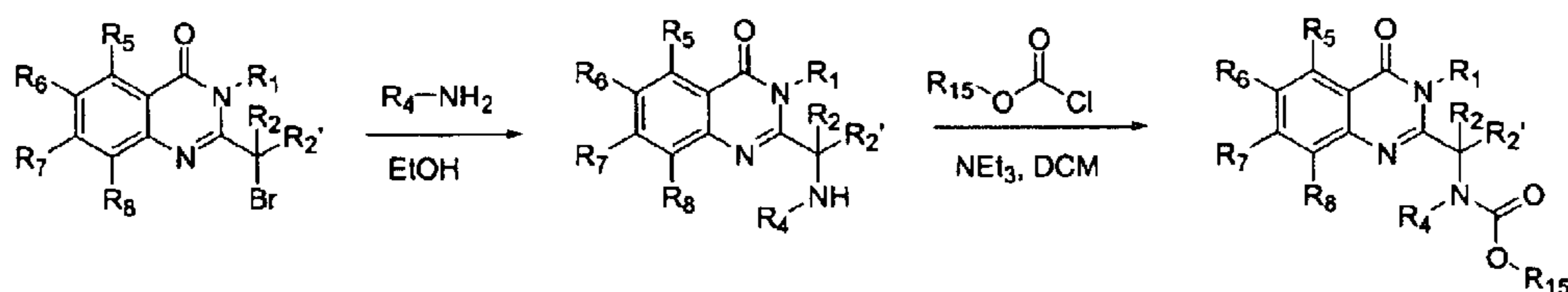
Figure 5c: Urea Synthesis
