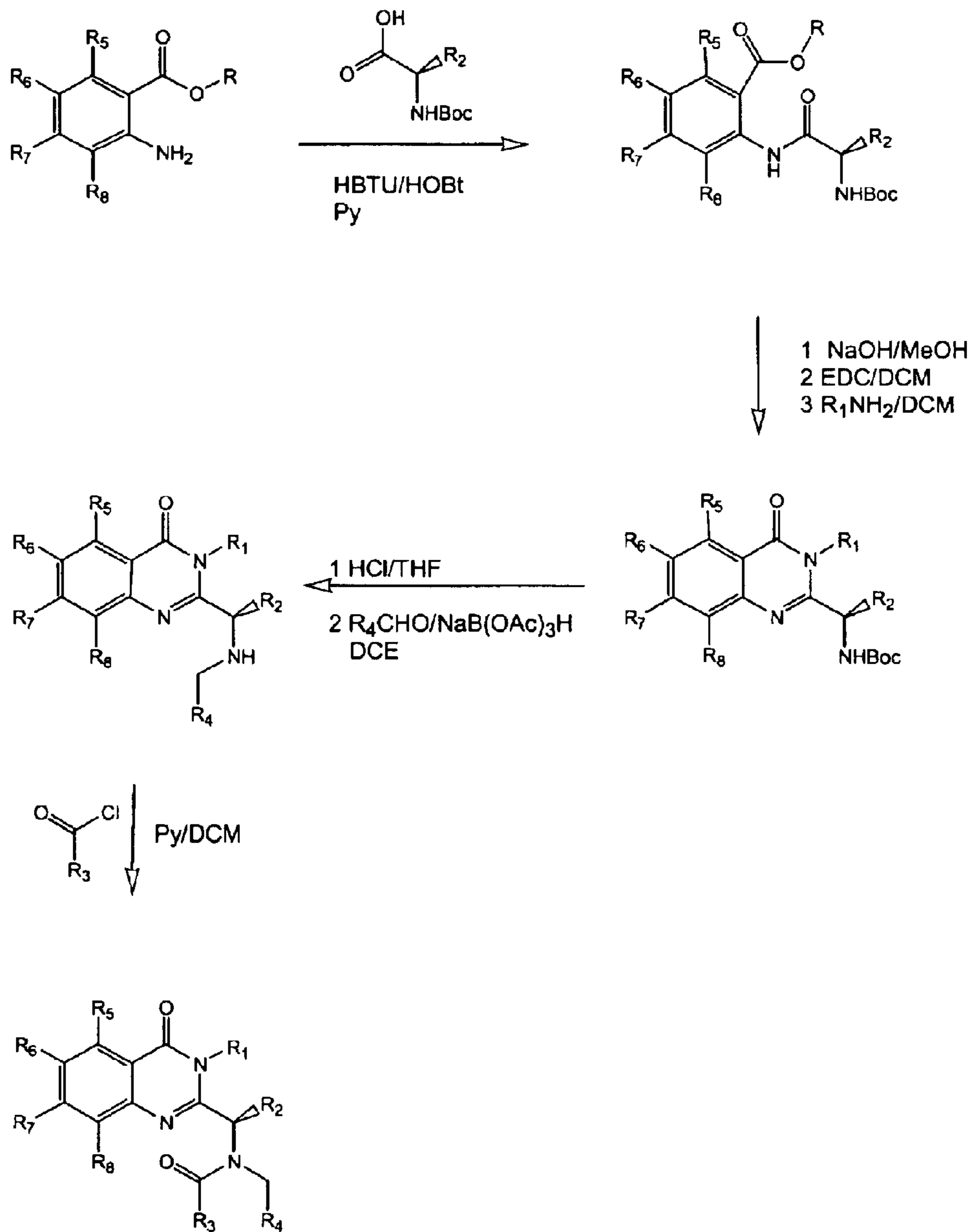
Figure 4: Asymmetric Synthesis
