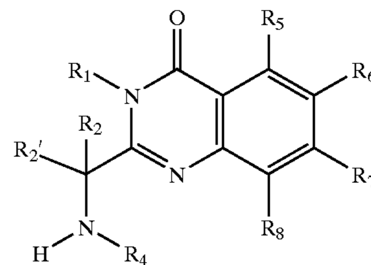
and quinazolinone amines of formulae 1c and 1d
