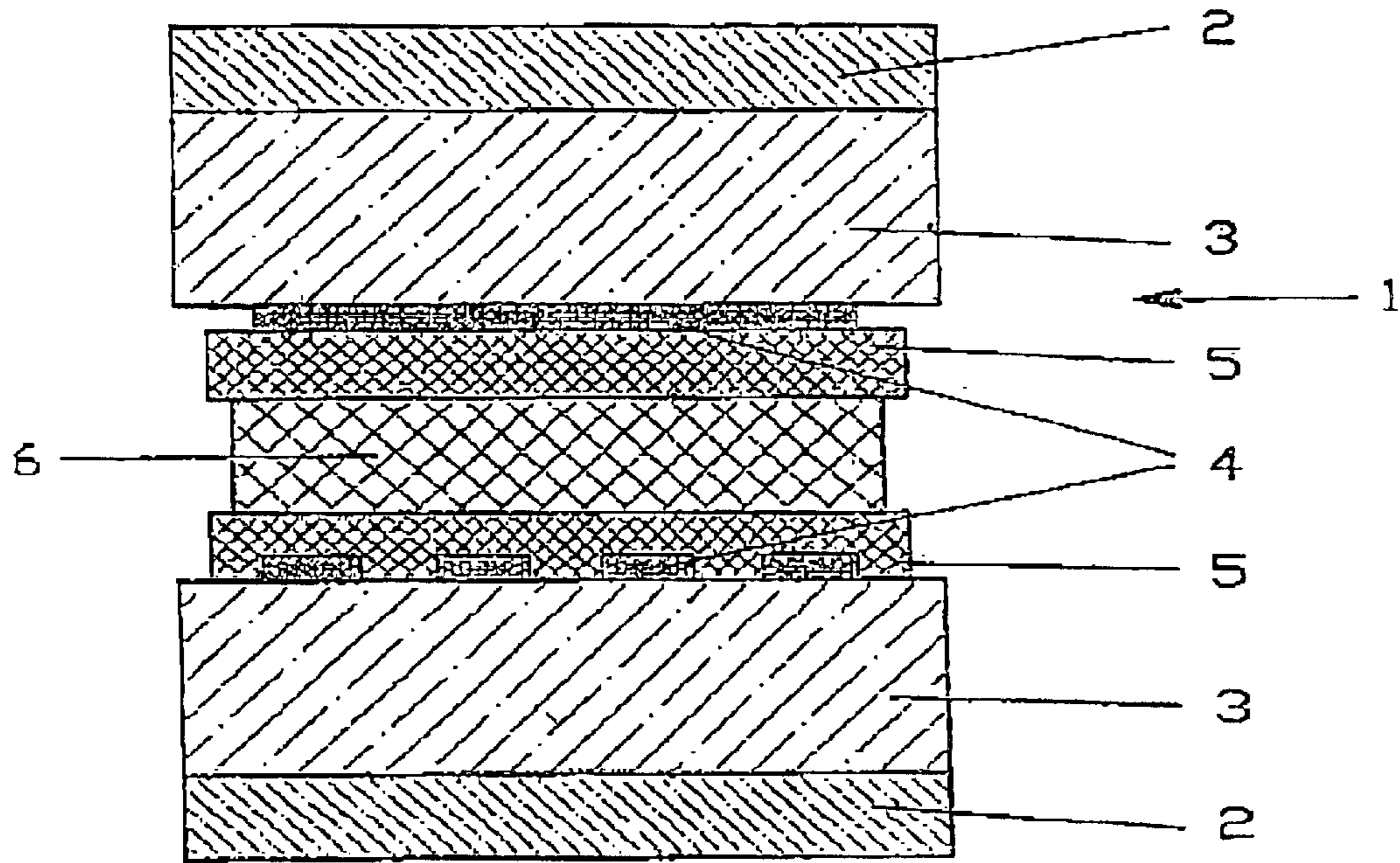
Fig. 1 PRIOR ART
