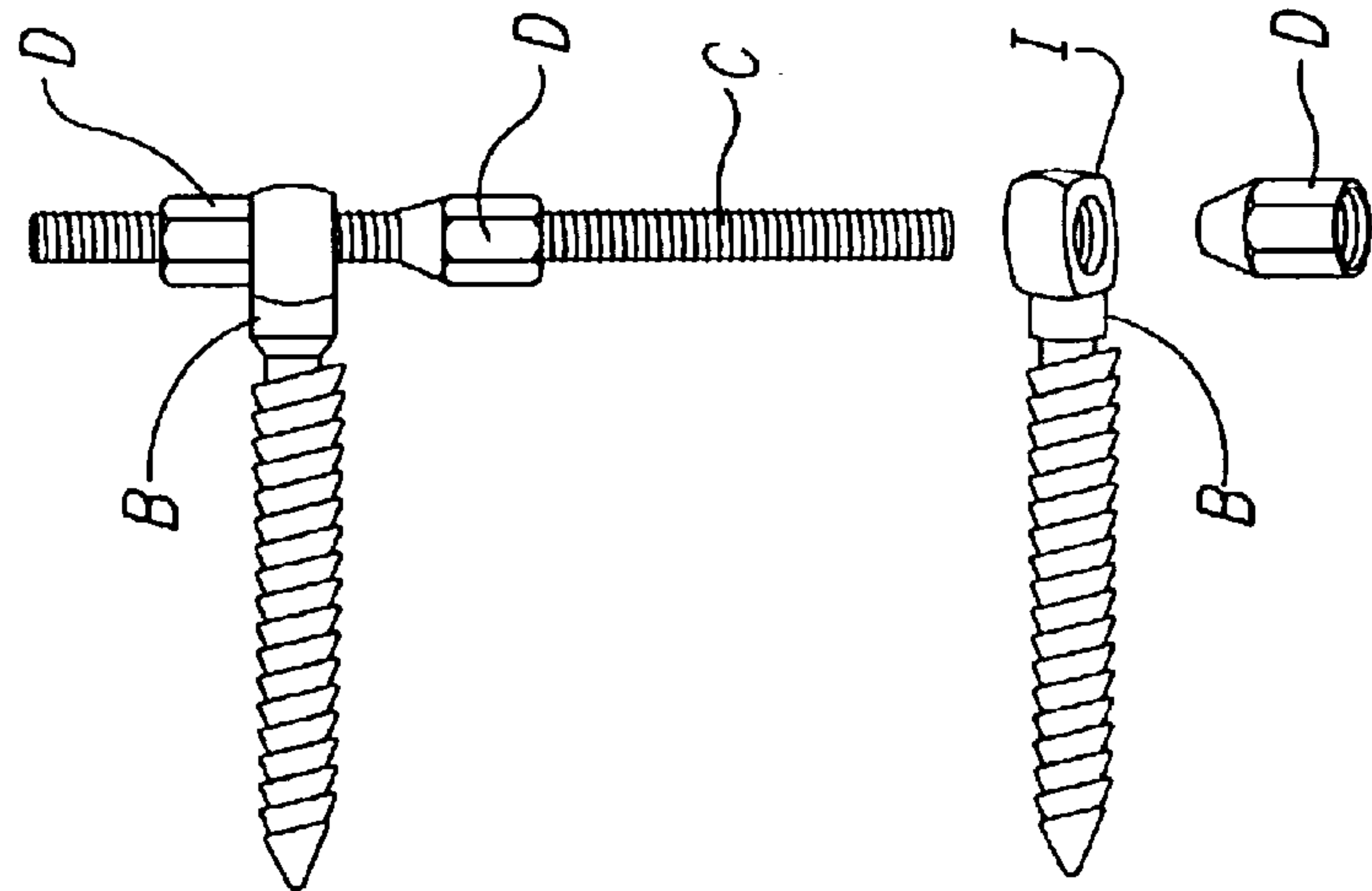
Fig. 2 (Prior Art)
