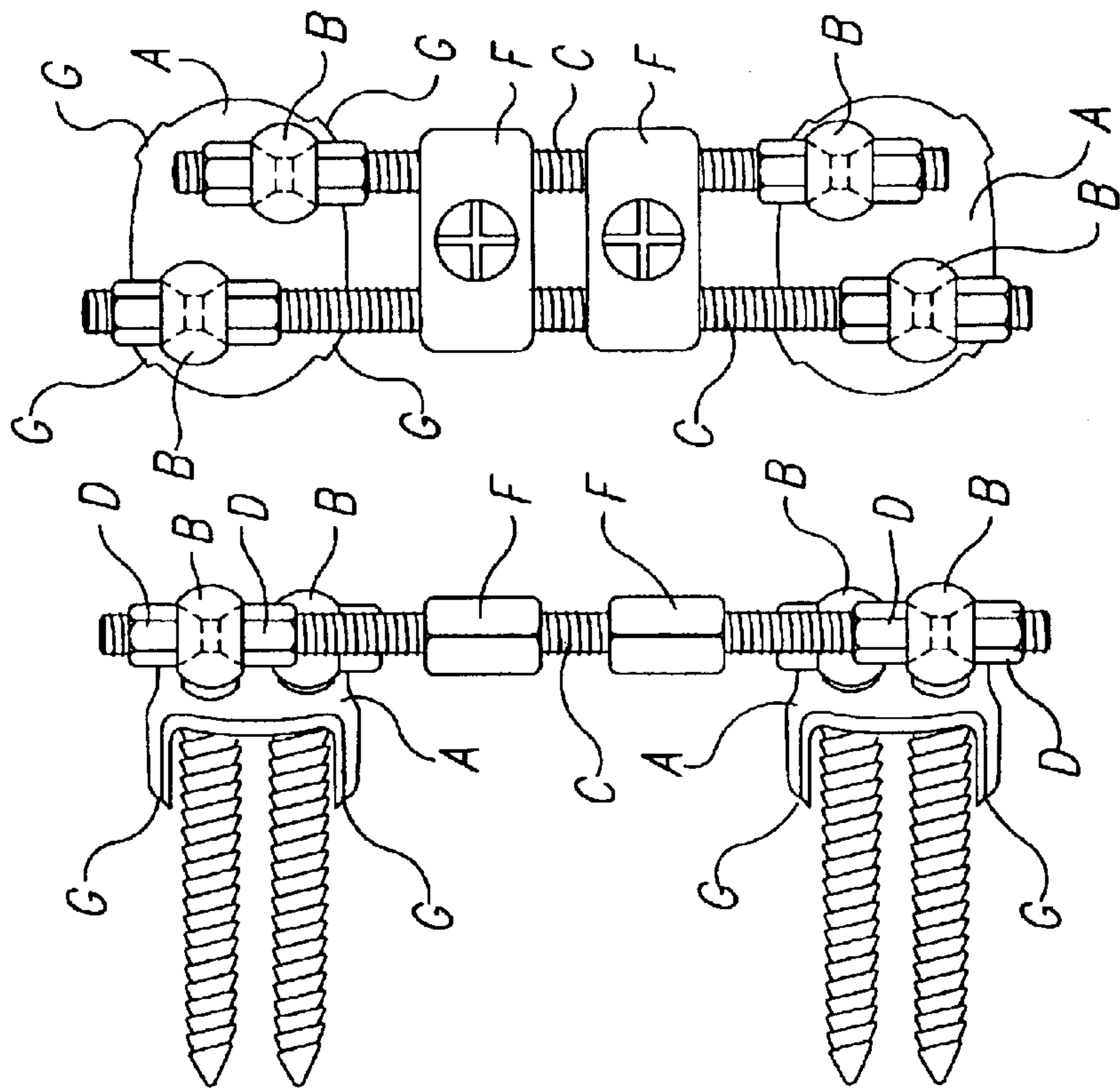
Fig. 3 (Prior Art)
