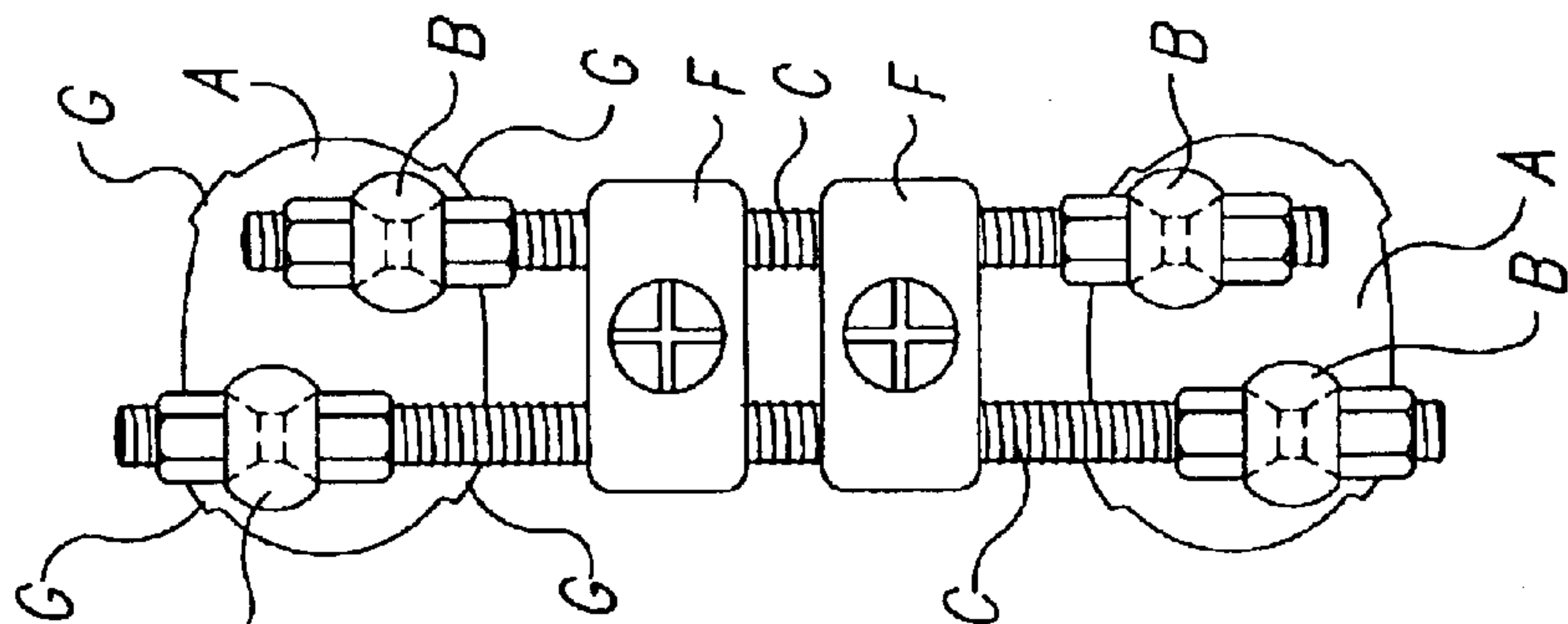
Fig. 4 (Prior Art)
