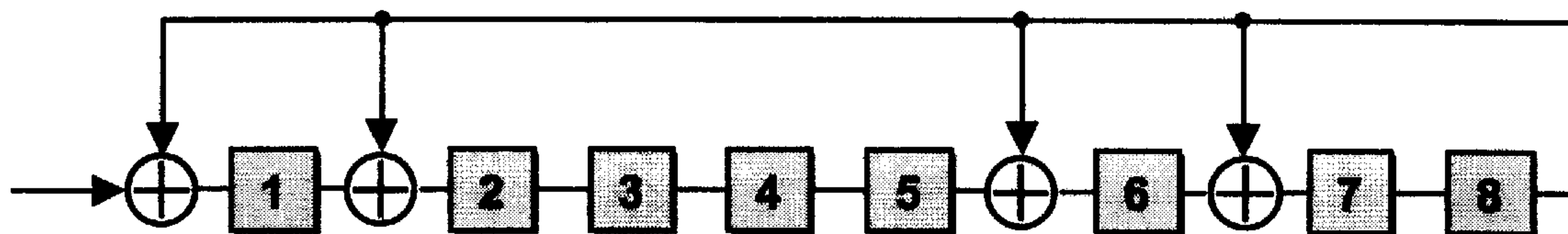
FIG. 4 (PRIOR ART)
