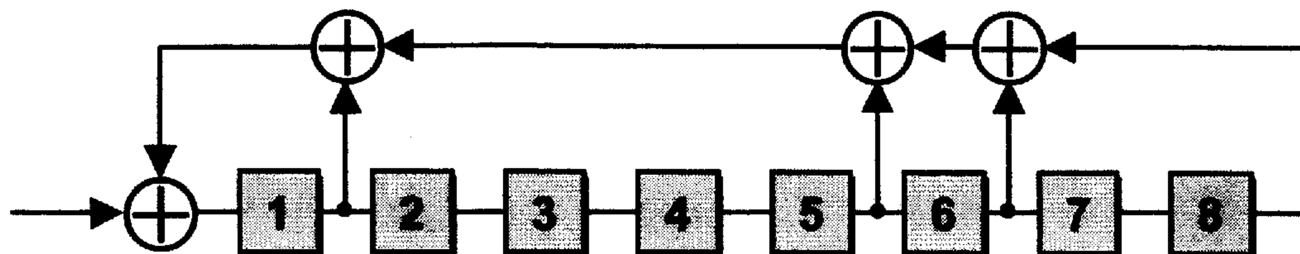
FIG. 3 (PRIOR ART)
