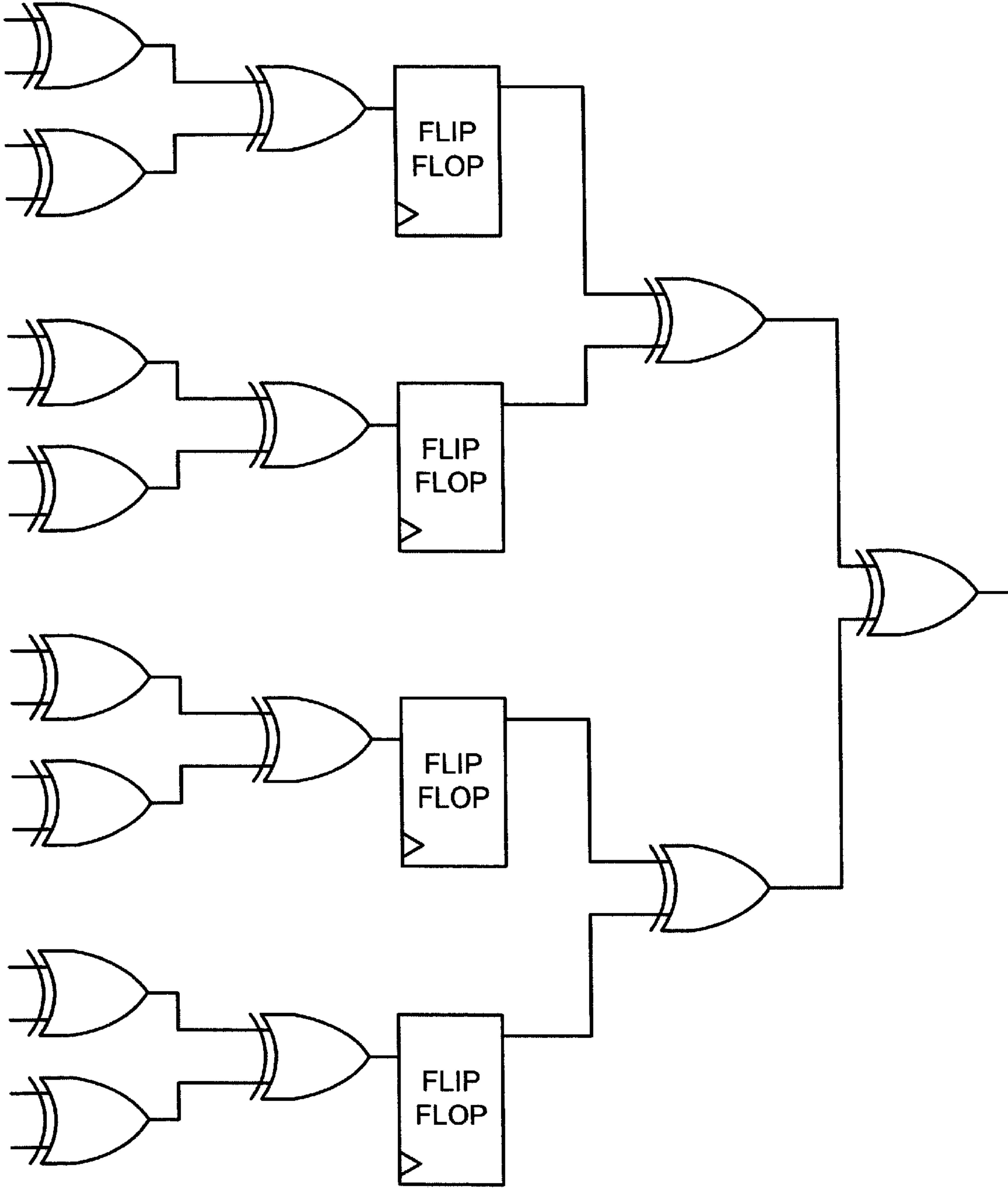
FIG. 6 (PRIOR ART)
