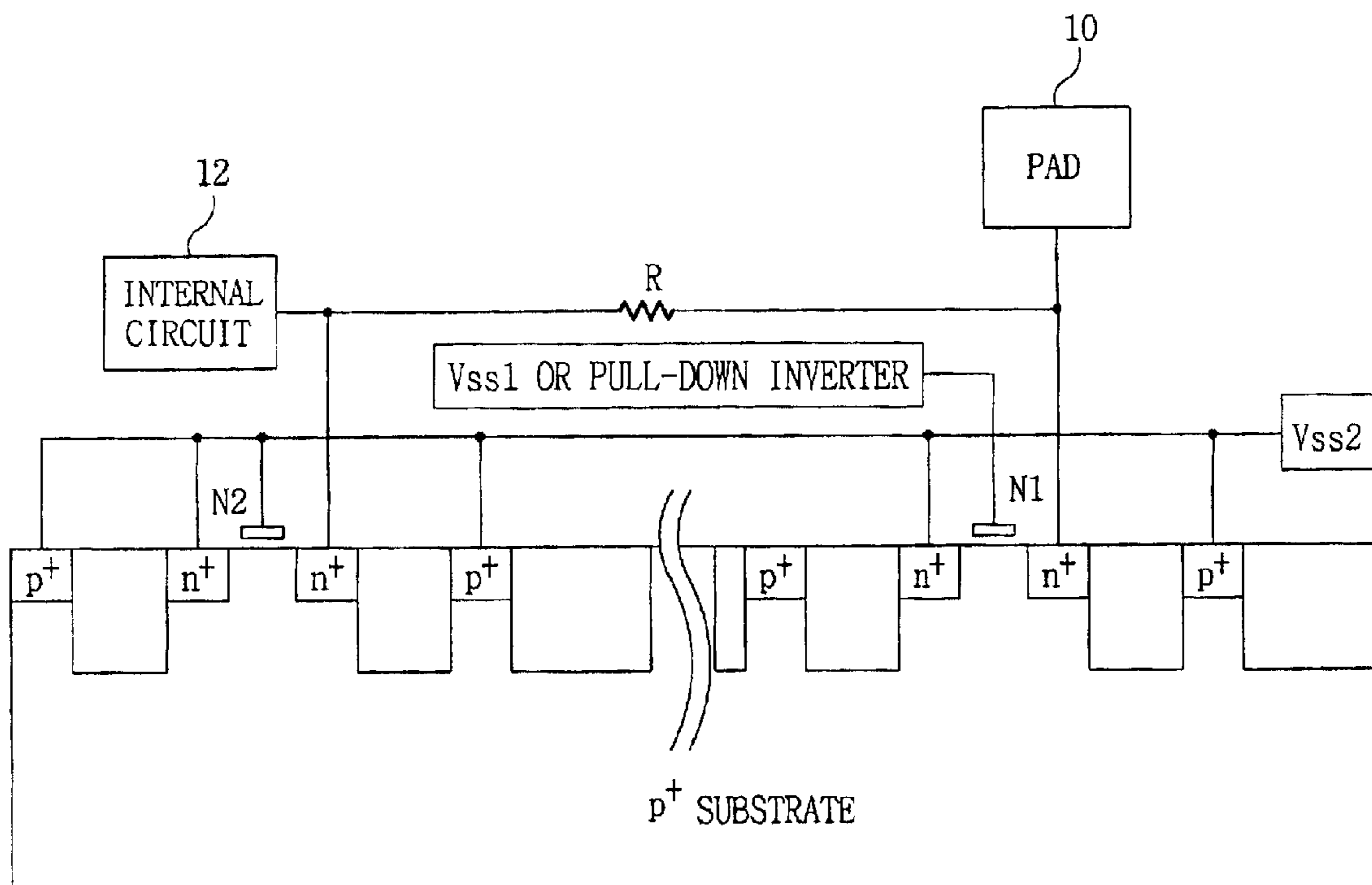
FIG. 2 BACKGROUND ART
