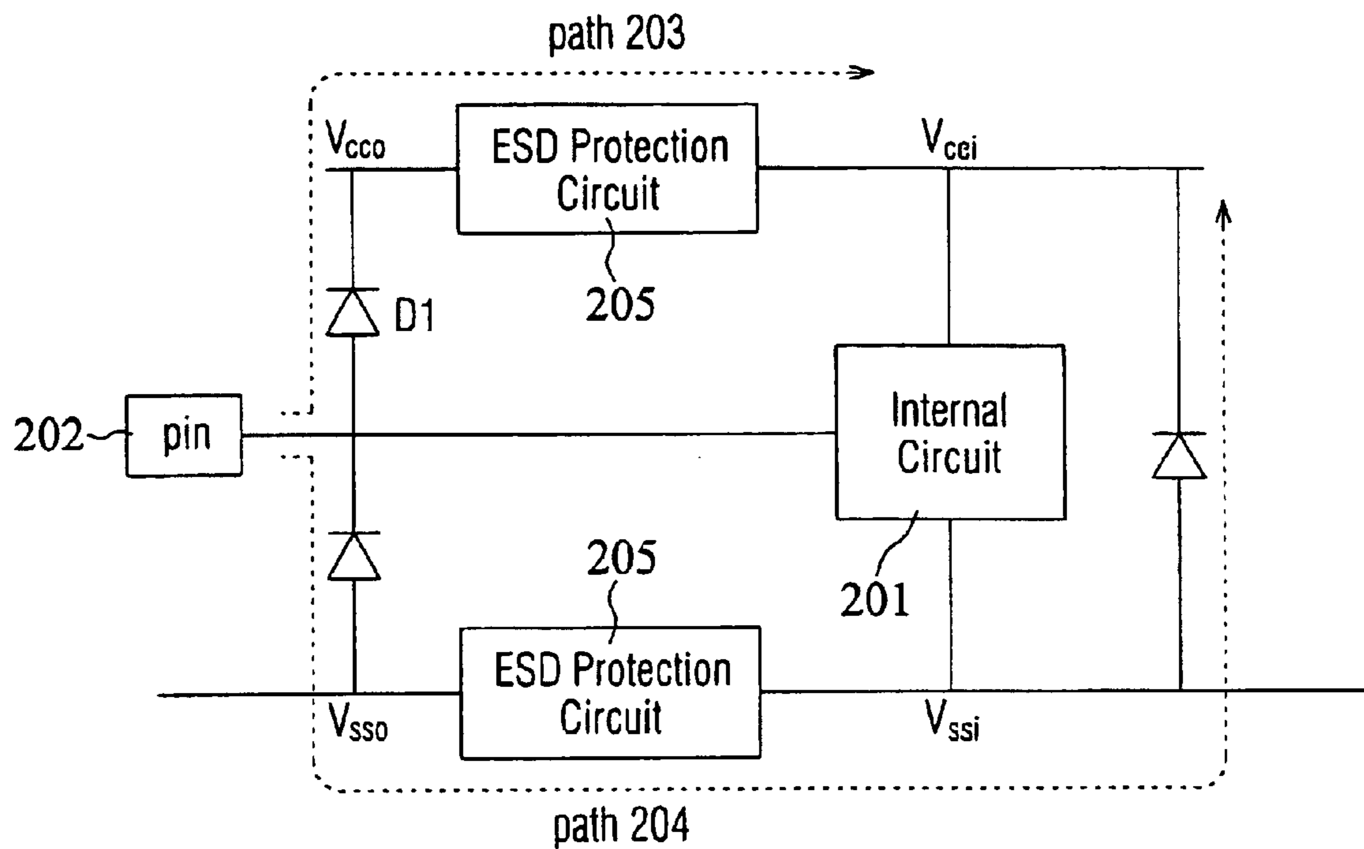
FIG. 2 (PRIOR ART)
