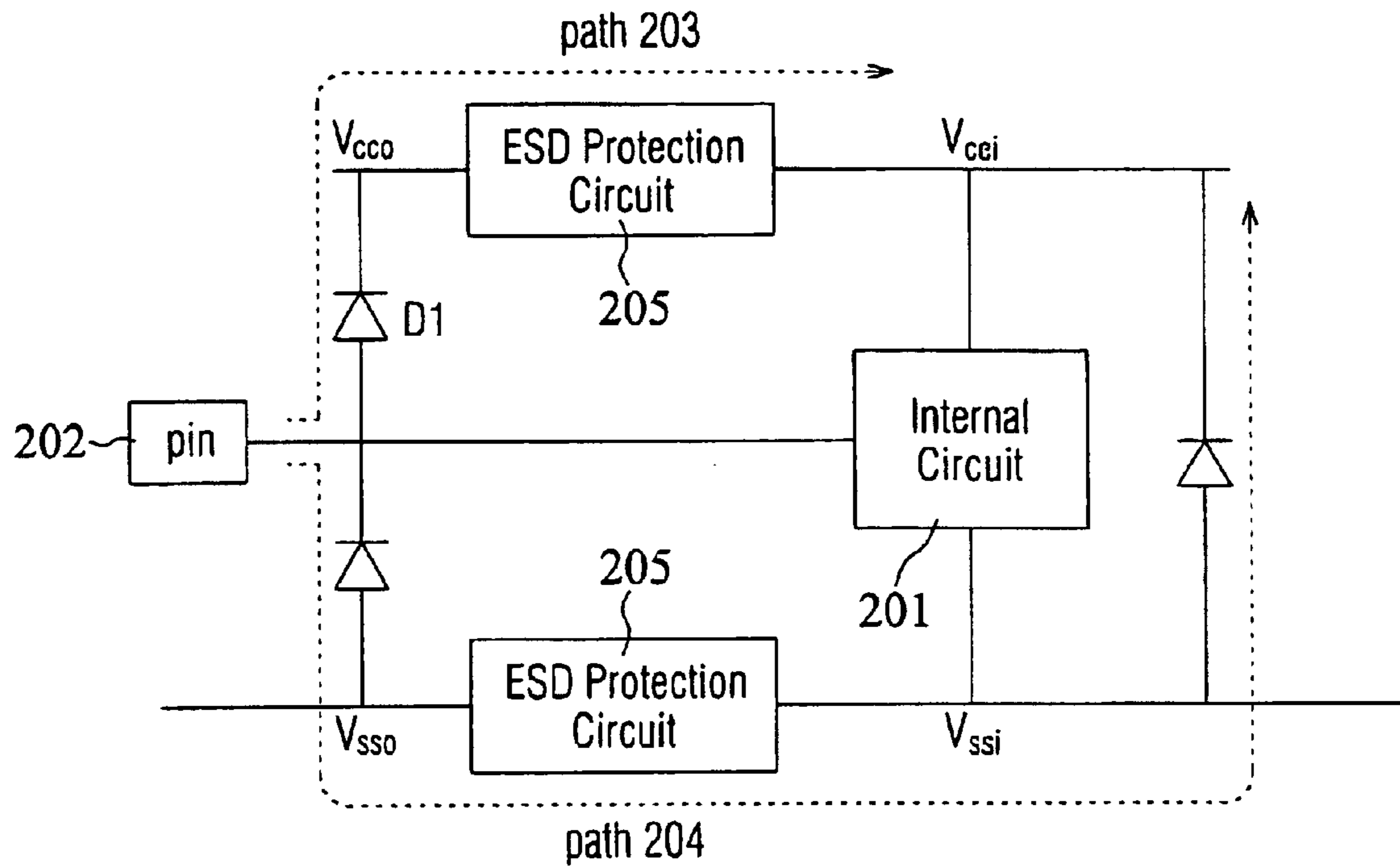
FIG. 2 (PRIOR ART)
