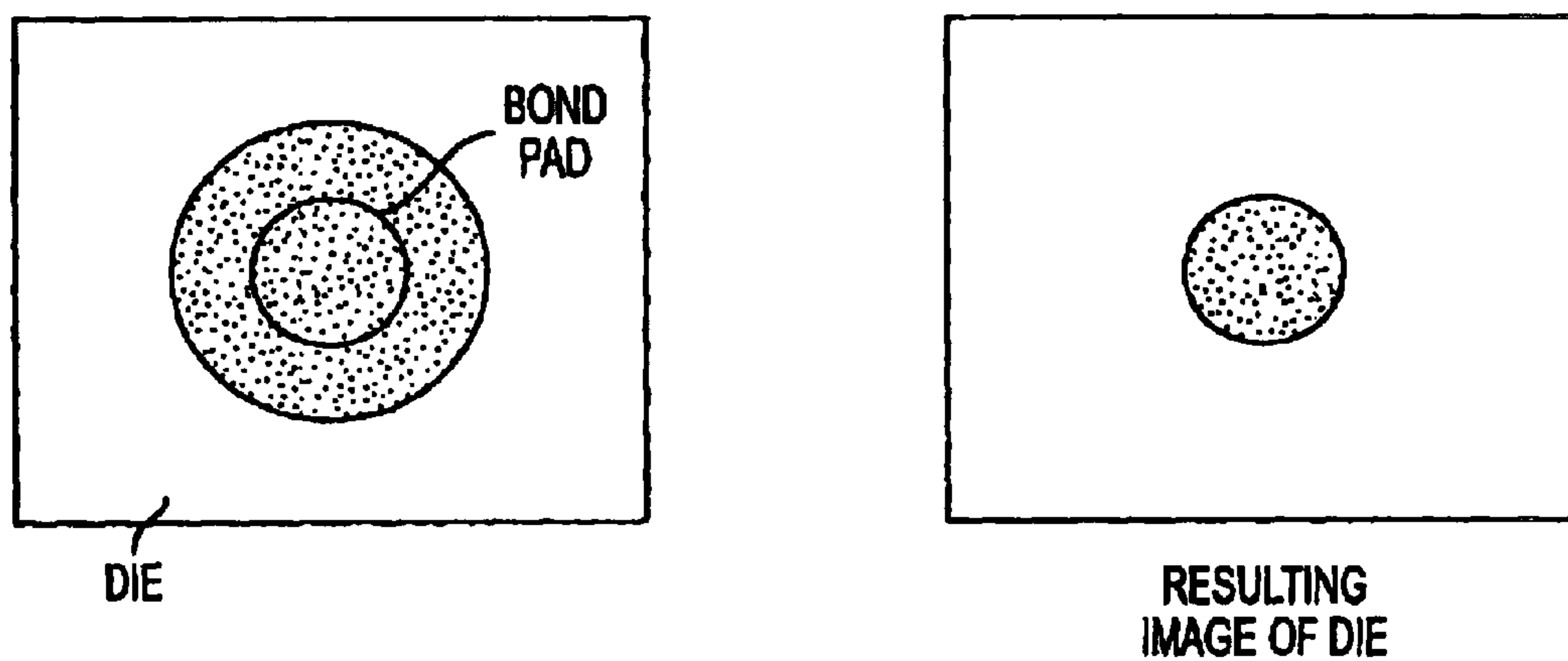
FIG. 10 (PRIOR ART)
