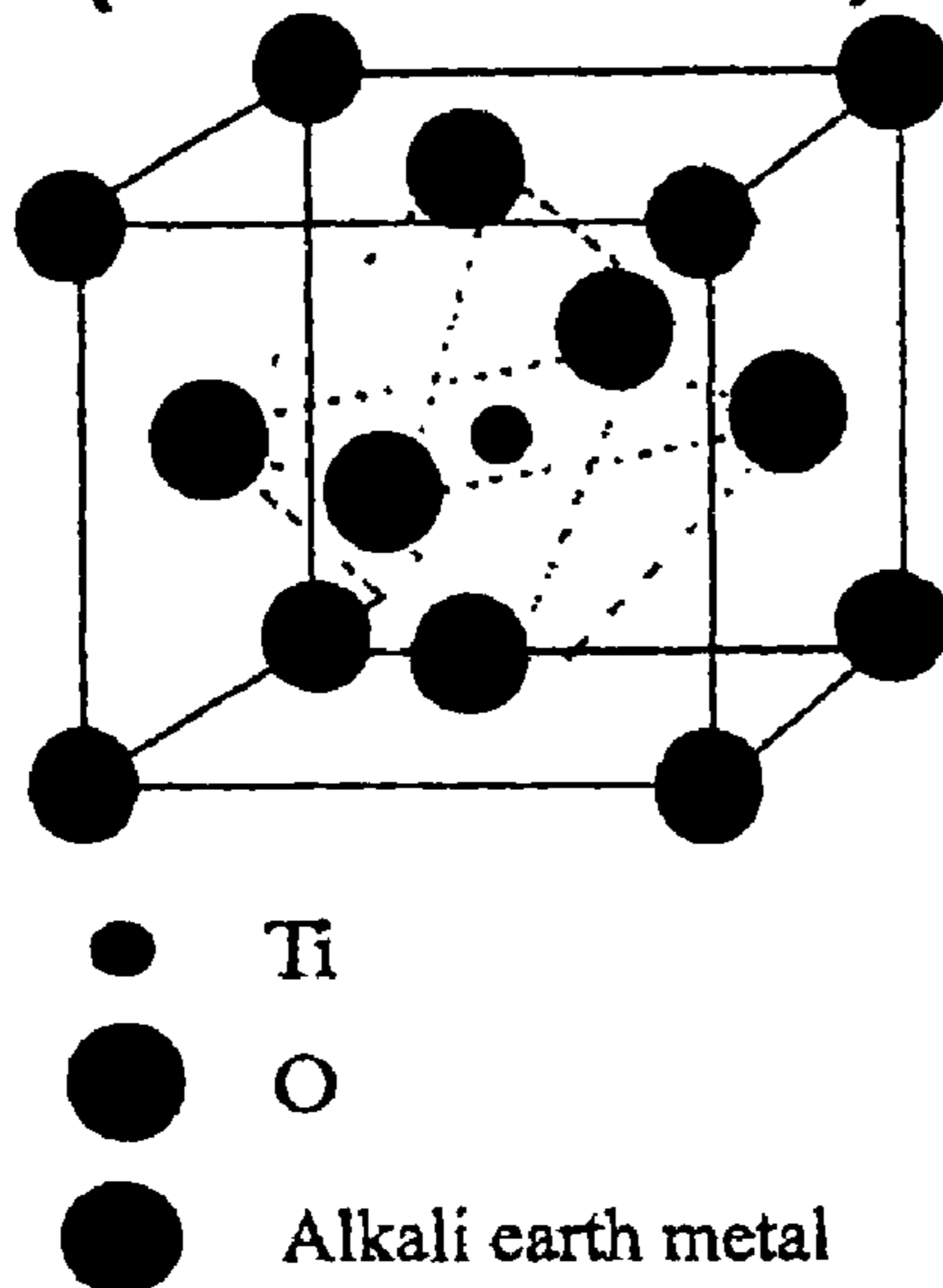
Fig. 1 (PRIOR ART)
