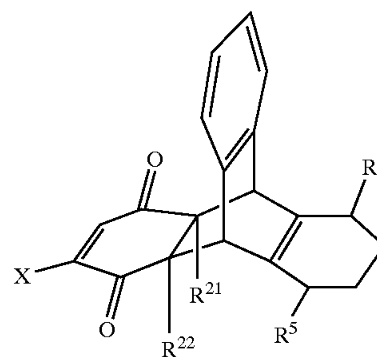
S analog 9: Y = Br, X = SCH 2 CH(CO 2 H)NH 2
