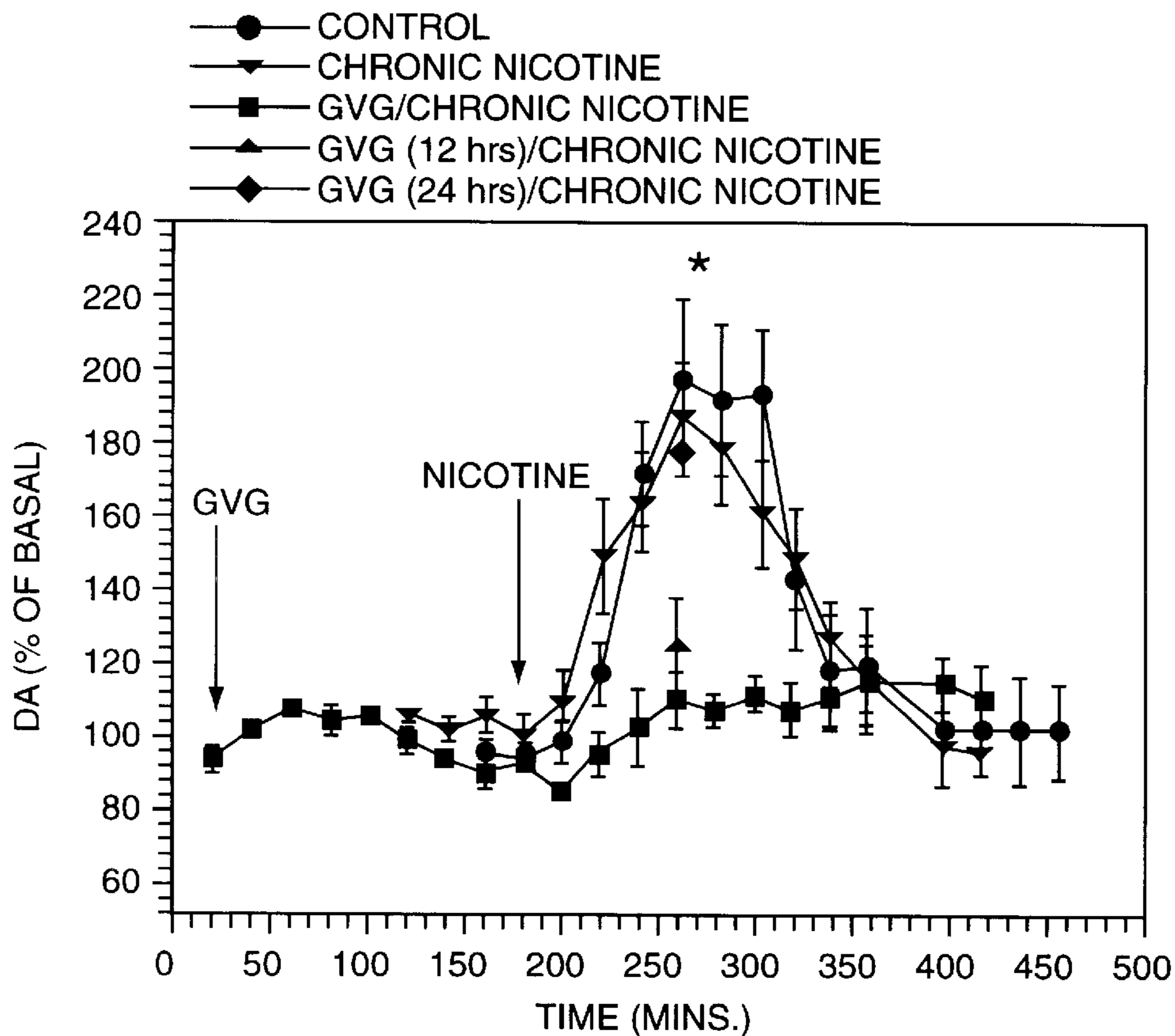
Effect of (-)-nicotine on extracellular NACC DA in chronically treated freely moving rats. * Values obtained following nicotine challenge in nicotine-treated animals and animals that received GVG (100 mg/kg) 24 hours prior to a nicotine challenge are not statistically different than normal control values (ANOVA and Student Neuman-Keuls test).
