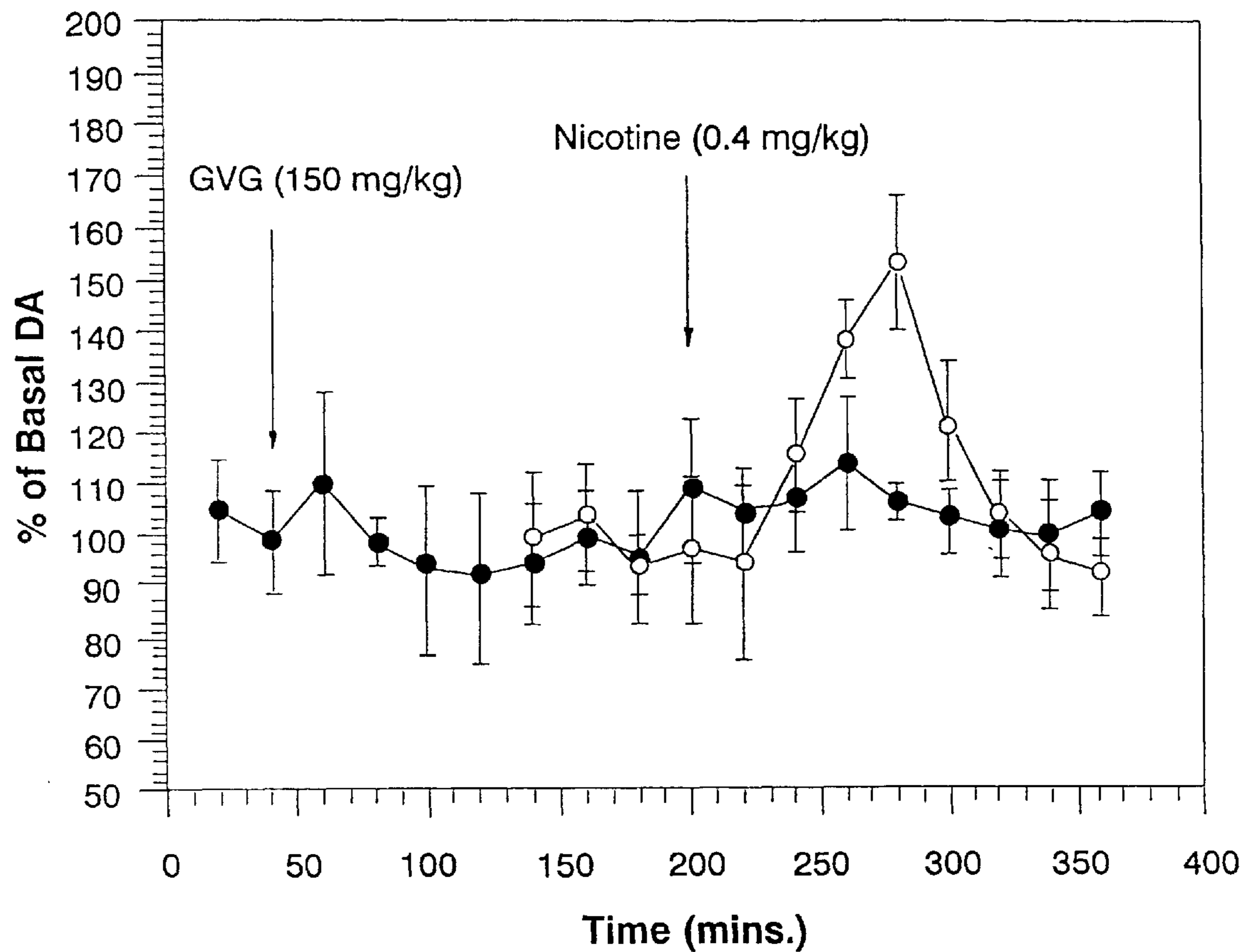
Effects of GVG on nicotine-induced extracellular DA
