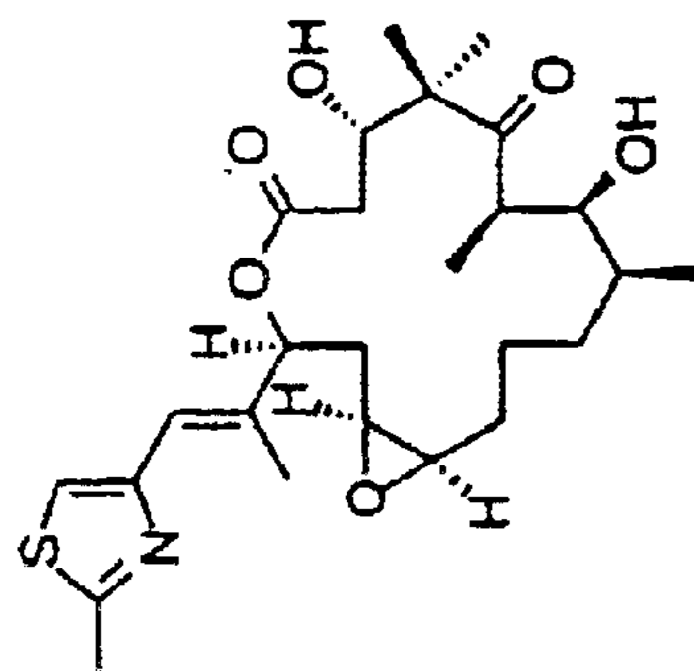
epothilone A
