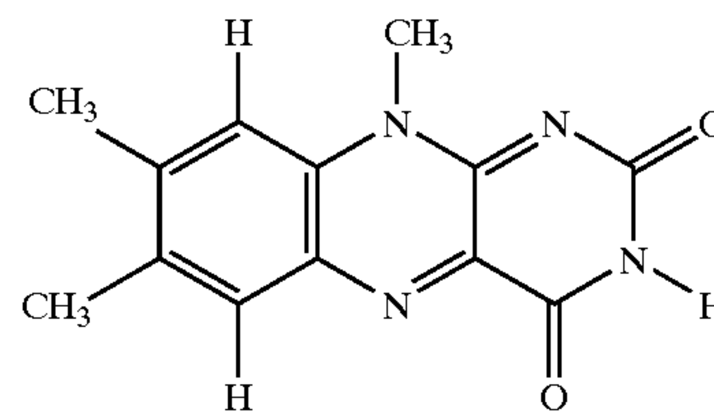
7,8,10-trimethylisoalloxazine
